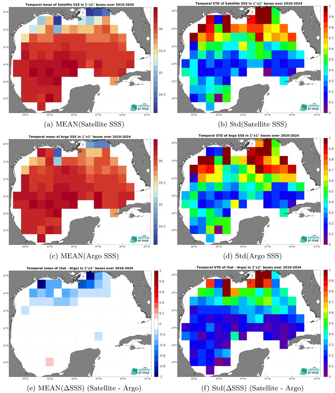
Figure 7: Temporal mean (left) and Std (right) of SSS from SMOS SSS L4 v1 - Daily (CMEMS-CNR) (top), Argo (middle), and of \Delta SSS (Satellite - Argo). Only match-up pairs are used to generate these maps.
