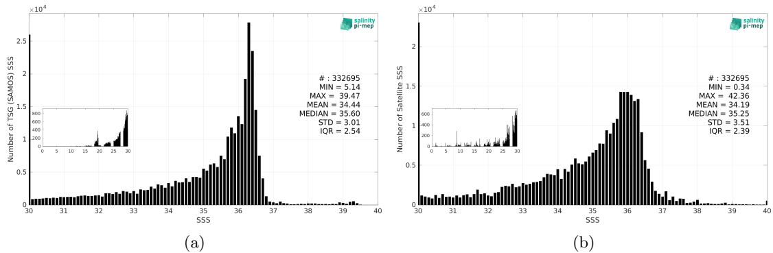
Figure 3: Histograms of SSS from TSG (SAMOS) (a) and SMOS SSS L4 OI v346 - Weekly (CMEMS-CATDS-LOPS) (b) considering all match-up pairs per bins of 0.1 over the Gulf of Mexico Pi-MEP region and for the full satellite product period.
