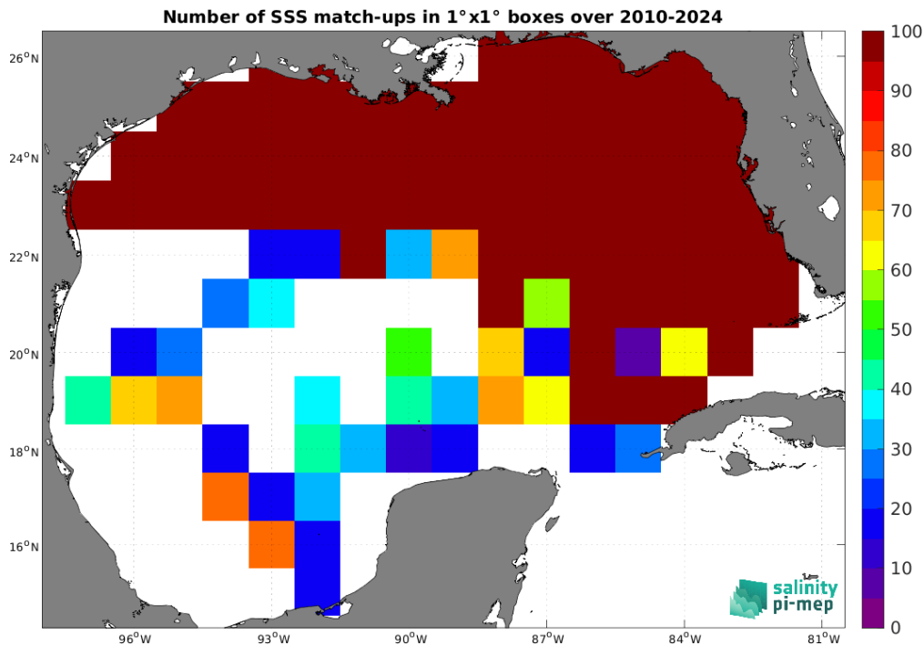
Figure 5: Number of SSS match-ups between TSG (SAMOS) SSS and the SMOS SSS L4 OI v346 - Weekly (CMEMS-CATDS-LOPS) SSS product for the Gulf of Mexico Pi-MEP region over 1^\circ \times 1^\circ boxes and for the full satellite product period.
