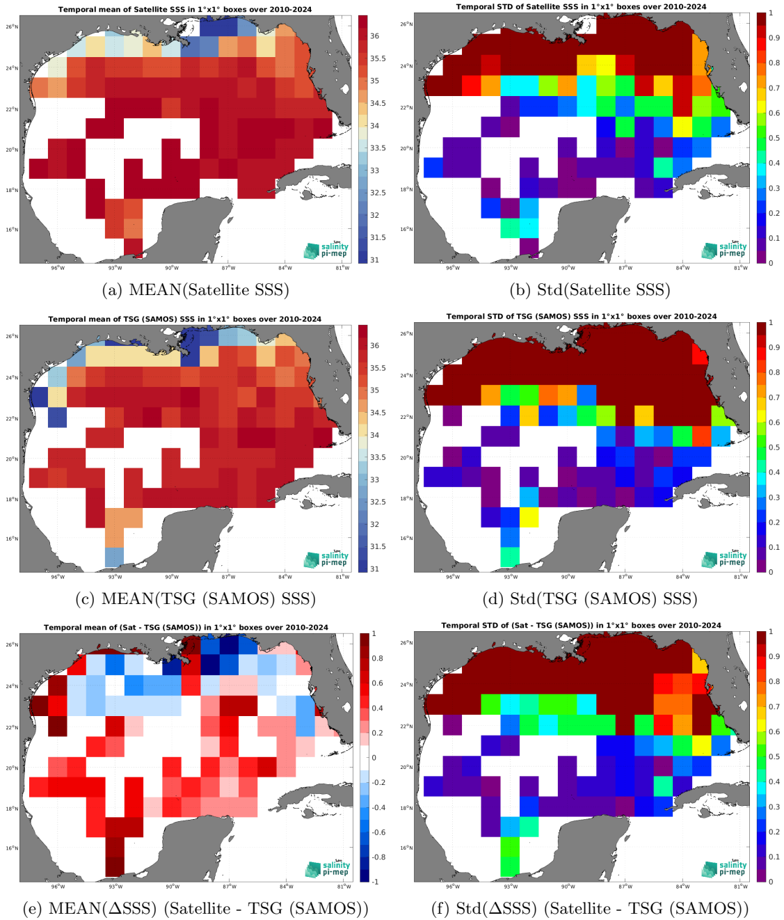
Figure 7: Temporal mean (left) and Std (right) of SSS from SMOS SSS L4 OI v346 - Weekly (CMEMS-CATDS-LOPS) (top), TSG (SAMOS) (middle), and of \Delta SSS (Satellite - TSG (SAMOS)). Only match-up pairs are used to generate these maps.
