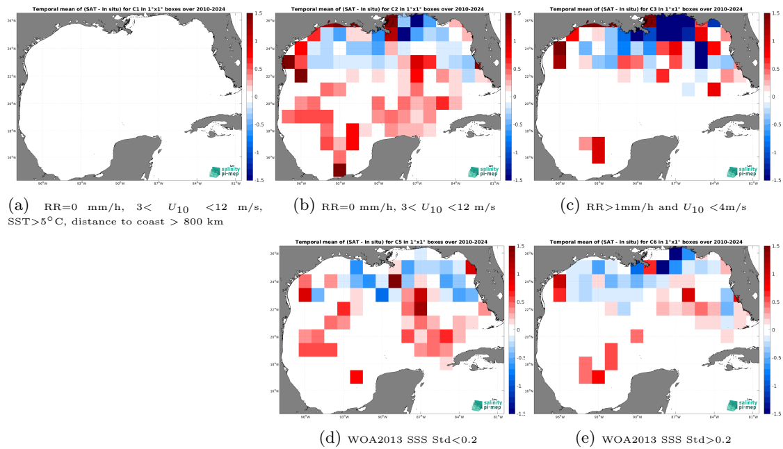
Figure 14: Temporal mean gridded over spatial boxes of size 1^\circ \times 1^\circ of \Delta SSS (SMOS SSS L4 OI v346 - Weekly (CMEMS-CATDS-LOPS) - TSG (SAMOS)) for 5 different subdatasets corresponding to:RR=0 mm/h, 3 < U_{10} < 12 m/s, SST >5^\circ\text{C} , distance to coast > 800 km (a), RR=0 mm/h, 3 < U_{10} < 12 m/s (b), RR >1 mm/h and U_{10} < 4 m/s (c), WOA2013 SSS Std <0.2 (d), WOA2013 SSS Std >0.2 (e).
