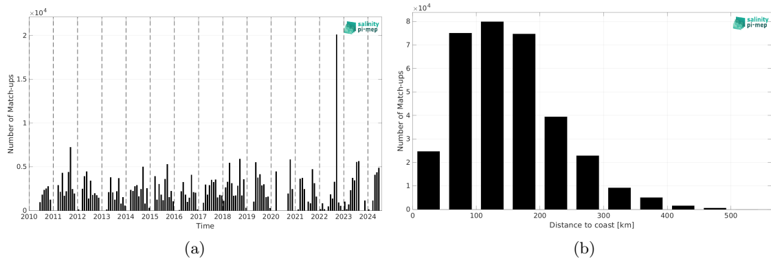
Figure 2: Number of match-ups between TSG (SAMOS) and SMOS SSS L4 OI v346 - Weekly (CMEMS-CATDS-LOPS) SSS as a function of time (a) and as function of the distance to coast (b) over the Gulf of Mexico Pi-MEP region and for the full satellite product period.
