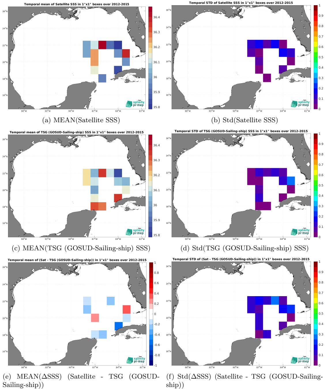
Figure 7: Temporal mean (left) and Std (right) of SSS from SMOS SSS L4 OI v346 - Weekly (CMEMS-CATDS-LOPS) (top), TSG (GOSUD-Sailing-ship) (middle), and of \Delta SSS (Satellite - TSG (GOSUD-Sailing-ship)). Only match-up pairs are used to generate these maps.
