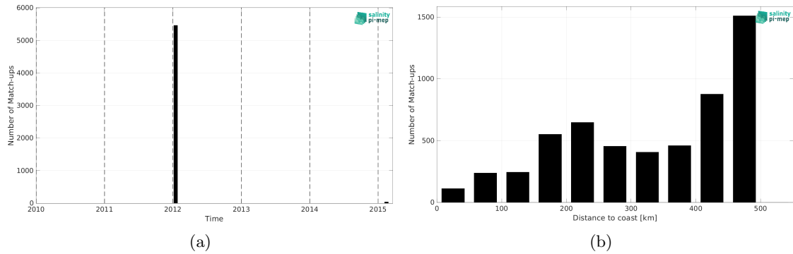
Figure 2: Number of match-ups between TSG (GOSUD-Sailing-ship) and SMOS SSS L4 OI v346 - Weekly (CMEMS-CATDS-LOPS) SSS as a function of time (a) and as function of the distance to coast (b) over the Gulf of Mexico Pi-MEP region and for the full satellite product period.
