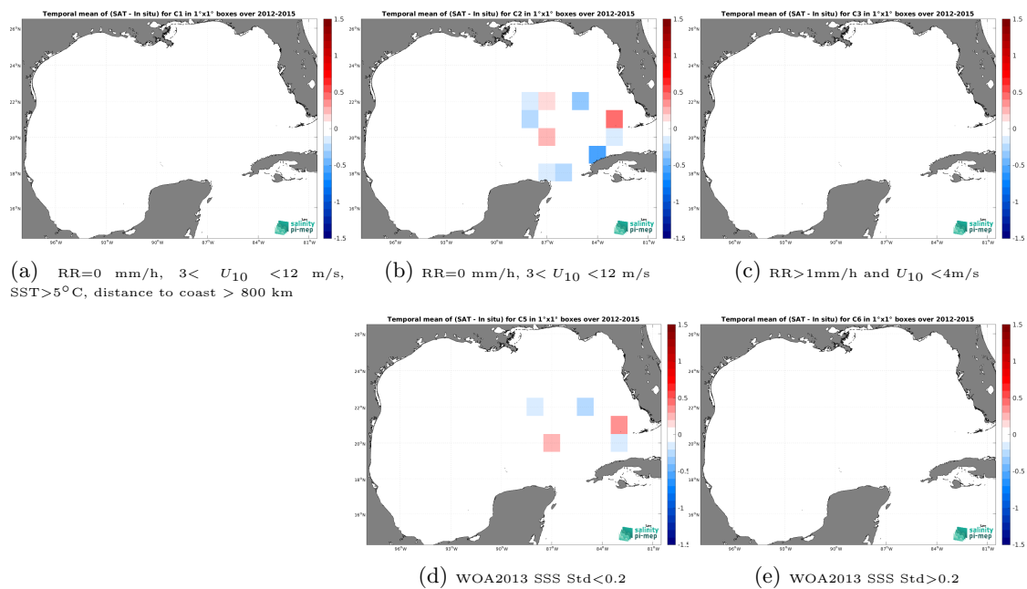
Figure 14: Temporal mean gridded over spatial boxes of size 1^\circ \times 1^\circ of \Delta SSS (SMOS SSS L4 OI v346 - Weekly (CMEMS-CATDS-LOPS) - TSG (GOSUD-Sailing-ship)) for 5 different sub-datasets corresponding to:RR=0 mm/h, 3 < U_{10} < 12 m/s, SST>5°C, distance to coast > 800 km (a), RR=0 mm/h, 3 < U_{10} < 12 m/s (b), RR>1mm/h and U_{10} < 4 m/s (c), WOA2013 SSS Std<0.2 (d), WOA2013 SSS Std>0.2 (e).
