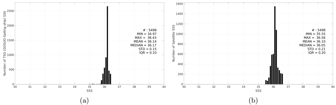
Figure 3: Histograms of SSS from TSG (GOSUD-Sailing-ship) (a) and SMOS SSS L4 OI v346 - Weekly (CMEMS-CATDS-LOPS) (b) considering all match-up pairs per bins of 0.1 over the Gulf of Mexico Pi-MEP region and for the full satellite product period.
