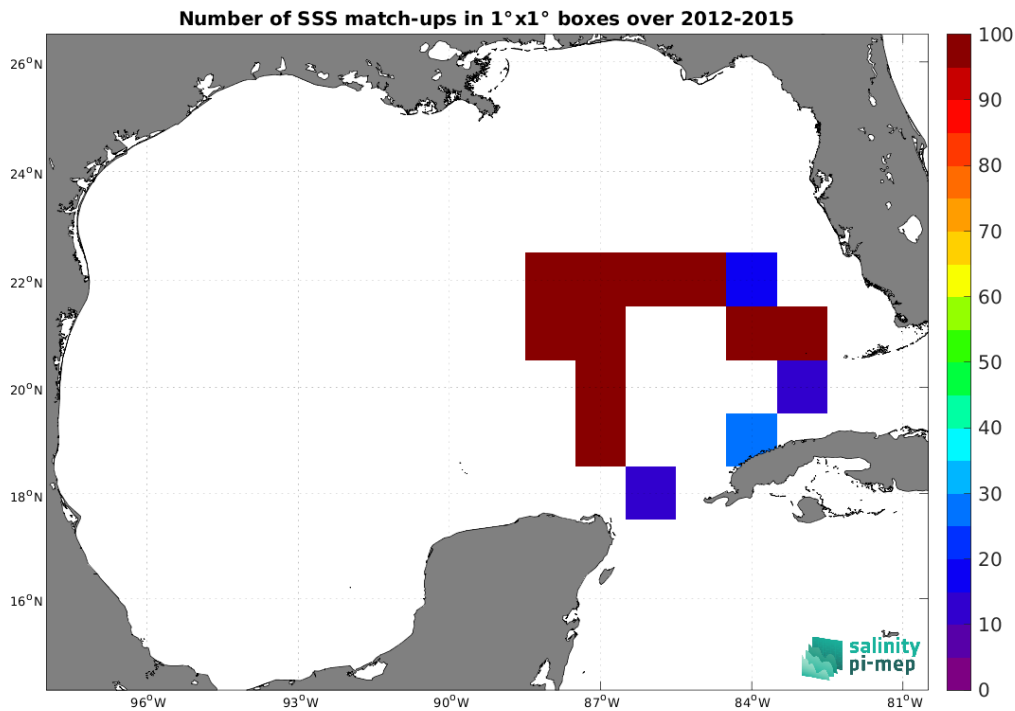
Figure 5: Number of SSS match-ups between TSG (GOSUD-Sailing-ship) SSS and the SMOS SSS L4 OI v346 - Weekly (CMEMS-CATDS-LOPS) SSS product for the Gulf of Mexico Pi-MEP region over 1^\circ \times 1^\circ boxes and for the full satellite product period.
