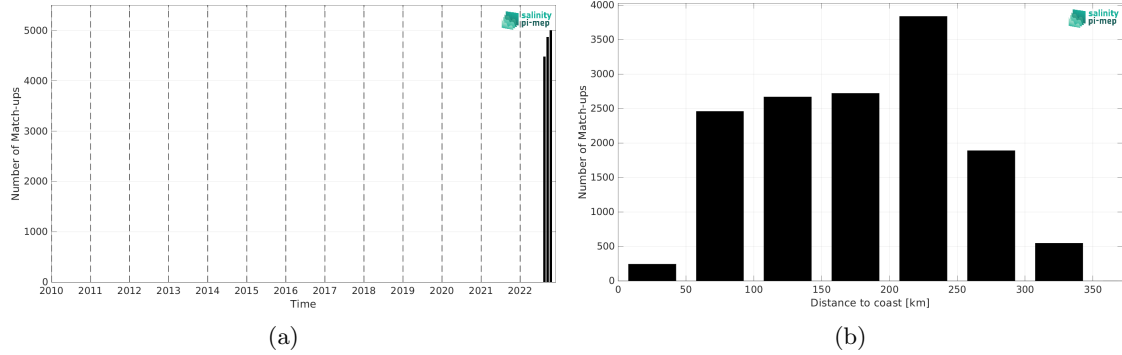
Figure 2: Number of match-ups between Saildrone and SMOS SSS L4 OI v346 - Weekly (CMEMS-CATDS-LOPS) SSS as a function of time (a) and as function of the distance to coast (b) over the Gulf of Mexico Pi-MEP region and for the full satellite product period.
