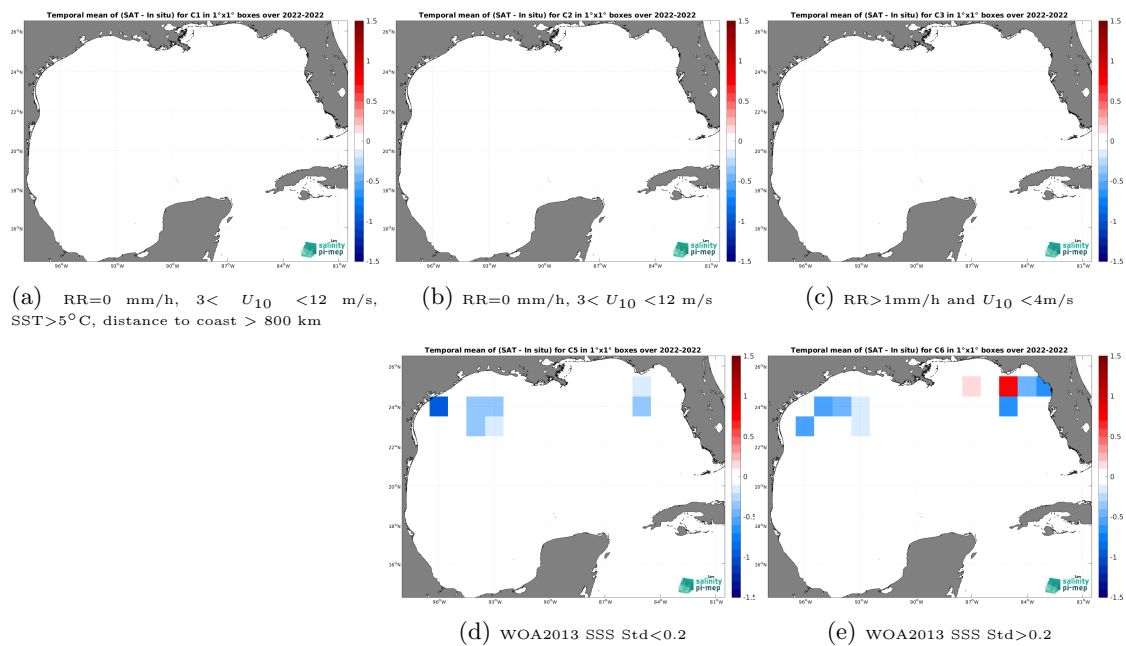
Figure 14: Temporal mean gridded over spatial boxes of size 1^\circ \times 1^\circ of \Delta SSS (SMOS SSS L4 OI v346 - Weekly (CMEMS-CATDS-LOPS) - Saildrone) for 5 different subdatasets corresponding to:RR=0 mm/h, 3 < U_{10} < 12 m/s, SST >5^\circ C, distance to coast > 800 km (a), RR=0 mm/h, 3 < U_{10} < 12 m/s (b), RR >1 mm/h and U_{10} < 4 m/s (c), WOA2013 SSS Std <0.2 (d), WOA2013 SSS Std >0.2 (e).
