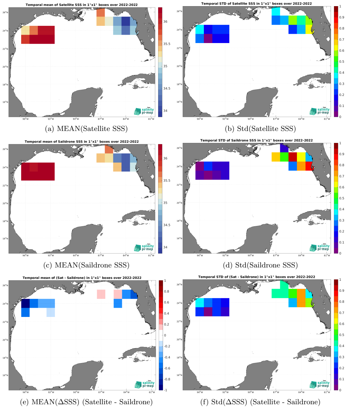
Figure 7: Temporal mean (left) and Std (right) of SSS from SMOS SSS L4 OI v346 - Weekly (CMEMS-CATDS-LOPS) (top), Saildrone (middle), and of \Delta SSS (Satellite - Saildrone). Only match-up pairs are used to generate these maps.
