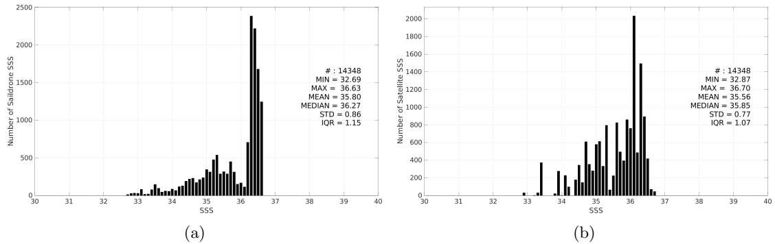
Figure 3: Histograms of SSS from Saildrone (a) and SMOS SSS L4 OI v346 - Weekly (CMEMS-CATDS-LOPS) (b) considering all match-up pairs per bins of 0.1 over the Gulf of Mexico Pi-MEP region and for the full satellite product period.
