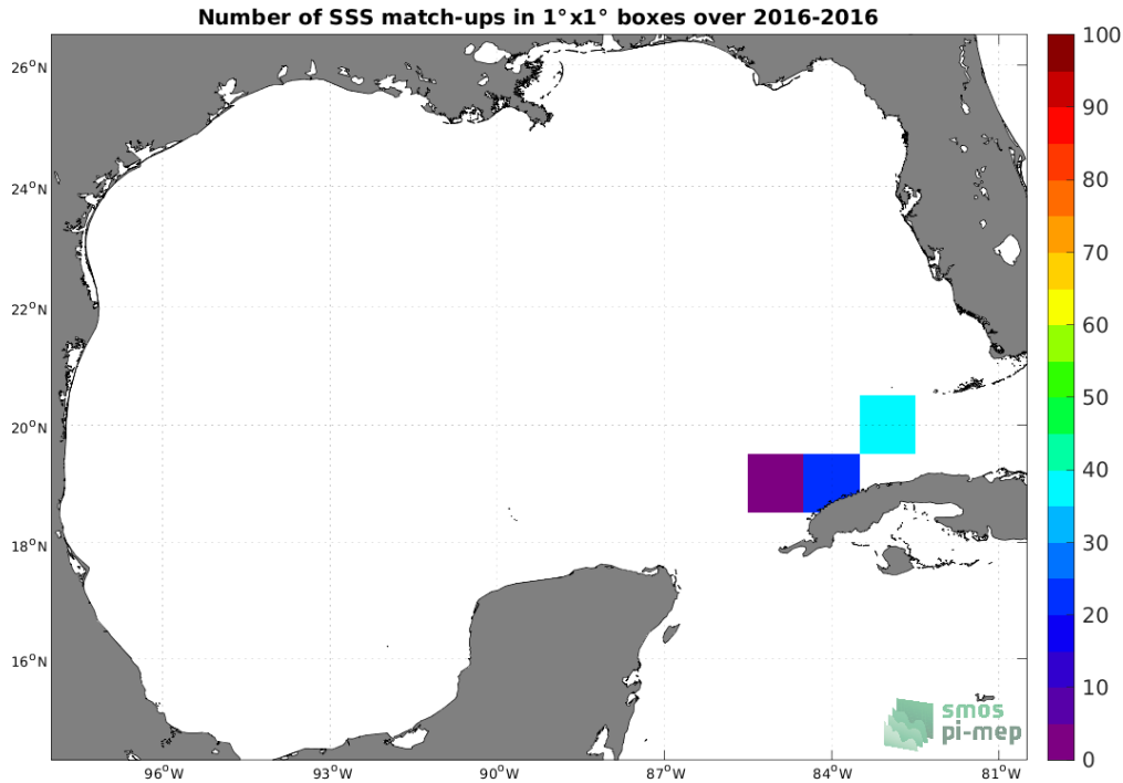
Figure 4: Number of SSS match-ups between TSG (LEGOS-DM) SSS and the SMOS SSS L4 OI v342 - Weekly (CMEMS-CATDS-LOPS) SSS product for the Gulf of Mexico Pi-MEP region over 1^\circ \times 1^\circ boxes and for the full satellite product period.
