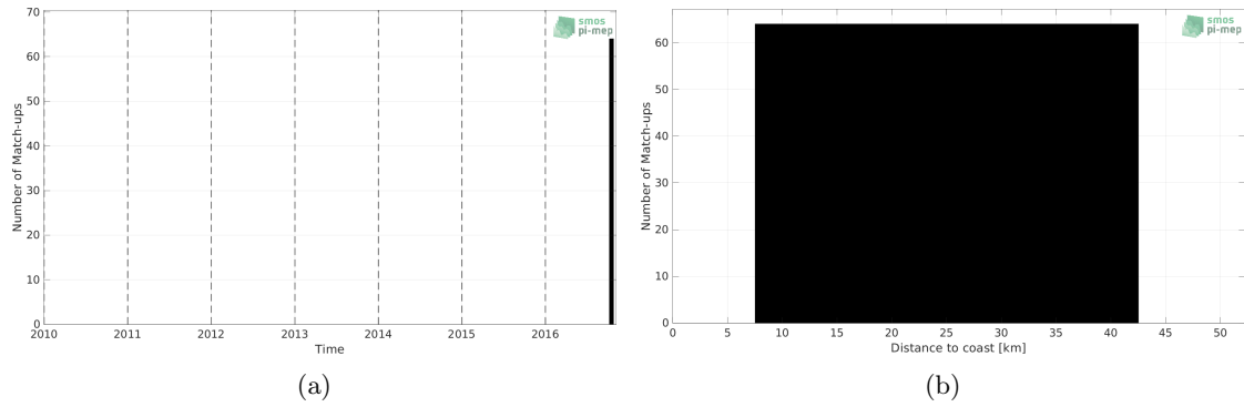
Figure 1: Number of match-ups between TSG (LEGOS-DM) and SMOS SSS L4 OI v342 - Weekly (CMEMS-CATDS-LOPS) SSS as a function of time (a) and as function of the distance to coast (b) over the Gulf of Mexico Pi-MEP region and for the full satellite product period.
