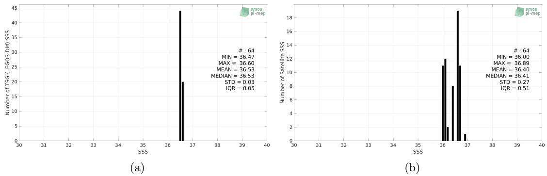
Figure 2: Histograms of SSS from TSG (LEGOS-DM) (a) and SMOS SSS L4 OI v342 - Weekly (CMEMS-CATDS-LOPS) (b) considering all match-up pairs per bins of 0.1 over the Gulf of Mexico Pi-MEP region and for the full satellite product period.
