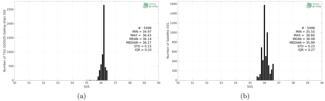
Figure 2: Histograms of SSS from TSG (GOSUD-Sailing-ship) (a) and SMOS SSS L4 OI v342 - Weekly (CMEMS-CATDS-LOPS) (b) considering all match-up pairs per bins of 0.1 over the Gulf of Mexico Pi-MEP region and for the full satellite product period.
