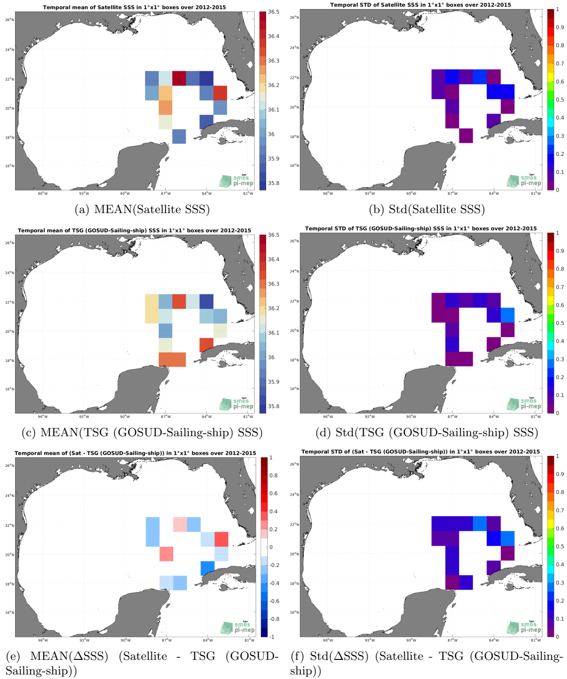
Figure 6: Temporal mean (left) and Std (right) of SSS from SMOS SSS L4 OI v342 - Weekly (CMEMS-CATDS-LOPS) (top), TSG (GOSUD-Sailing-ship) (middle), and of \Delta SSS (Satellite - TSG (GOSUD-Sailing-ship)). Only match-up pairs are used to generate these maps.
