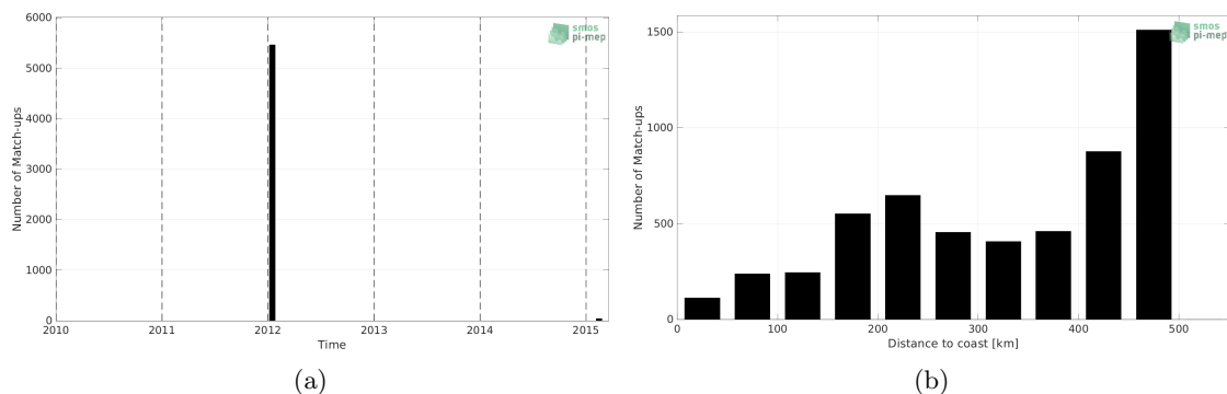
Figure 1: Number of match-ups between TSG (GOSUD-Sailing-ship) and SMOS SSS L4 OI v342 - Weekly (CMEMS-CATDS-LOPS) SSS as a function of time (a) and as function of the distance to coast (b) over the Gulf of Mexico Pi-MEP region and for the full satellite product period.
