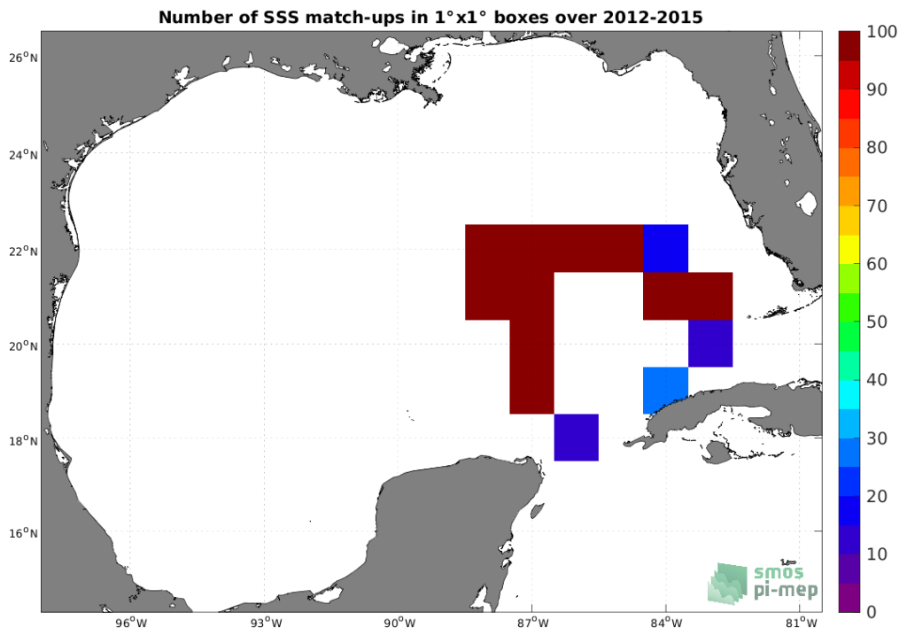
Figure 4: Number of SSS match-ups between TSG (GOSUD-Sailing-ship) SSS and the SMOS SSS L4 OI v342 - Weekly (CMEMS-CATDS-LOPS) SSS product for the Gulf of Mexico Pi-MEP region over 1^\circ \times 1^\circ boxes and for the full satellite product period.
