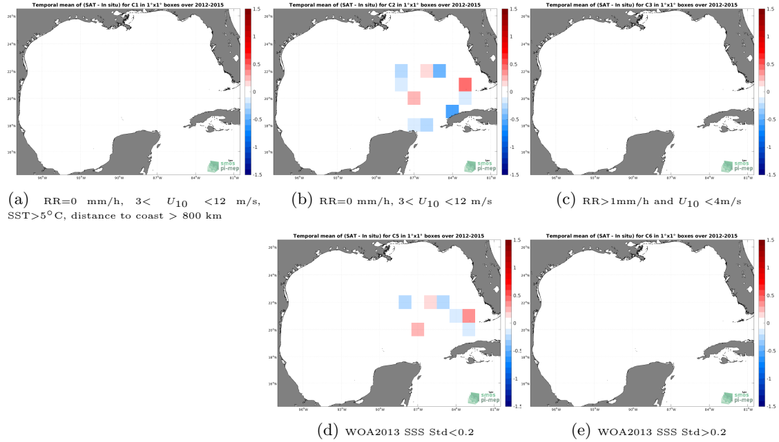
Figure 12: Temporal mean gridded over spatial boxes of size 1^\circ \times 1^\circ of \Delta SSS (SMOS SSS L4 OI v342 - Weekly (CMEMS-CATDS-LOPS) - TSG (GOSUD-Sailing-ship)) for 5 different sub-datasets corresponding to:RR=0 mm/h, 3 < U_{10} < 12 m/s, SST >5^\circ\text{C} , distance to coast > 800 km (a), RR=0 mm/h, 3 < U_{10} < 12 m/s (b), RR >1 mm/h and U_{10} < 4 m/s (c), WOA2013 SSS Std <0.2 (d), WOA2013 SSS Std >0.2 (e).
