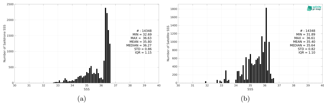
Figure 2: Histograms of SSS from Saildrone (a) and SMOS SSS L4 OI v342 - Weekly (CMEMS-CATDS-LOPS) (b) considering all match-up pairs per bins of 0.1 over the Gulf of Mexico Pi-MEP region and for the full satellite product period.
