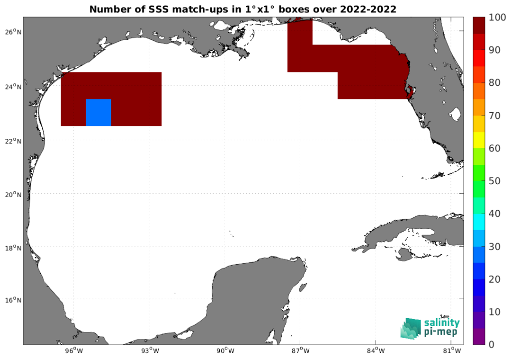
Figure 4: Number of SSS match-ups between Saildrone SSS and the SMOS SSS L4 OI v342 - Weekly (CMEMS-CATDS-LOPS) SSS product for the Gulf of Mexico Pi-MEP region over 1^\circ \times 1^\circ boxes and for the full satellite product period.
