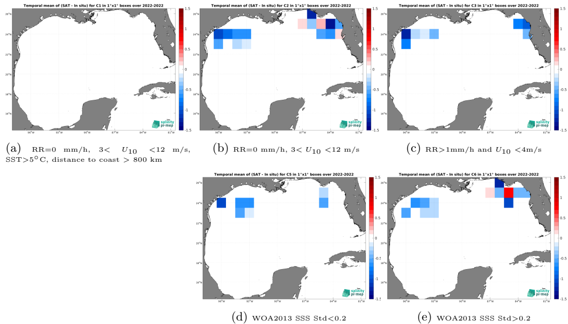
Figure 12: Temporal mean gridded over spatial boxes of size 1^{\circ}\times 1^{\circ} of \Delta\text{SSS} (SMOS SSS L4 OI v342 - Weekly (CMEMS-CATDS-LOPS) - Saildrone) for 5 different subdatasets corresponding to:RR=0 mm/h, 3 < U_{10} < 12 m/s, SST >5^{\circ}\text{C} , distance to coast > 800 km (a), RR=0 mm/h, 3 < U_{10} < 12 m/s (b), RR >1 mm/h and U_{10} < 4 m/s (c), WOA2013 SSS Std <0.2 (d), WOA2013 SSS Std >0.2 (e).
