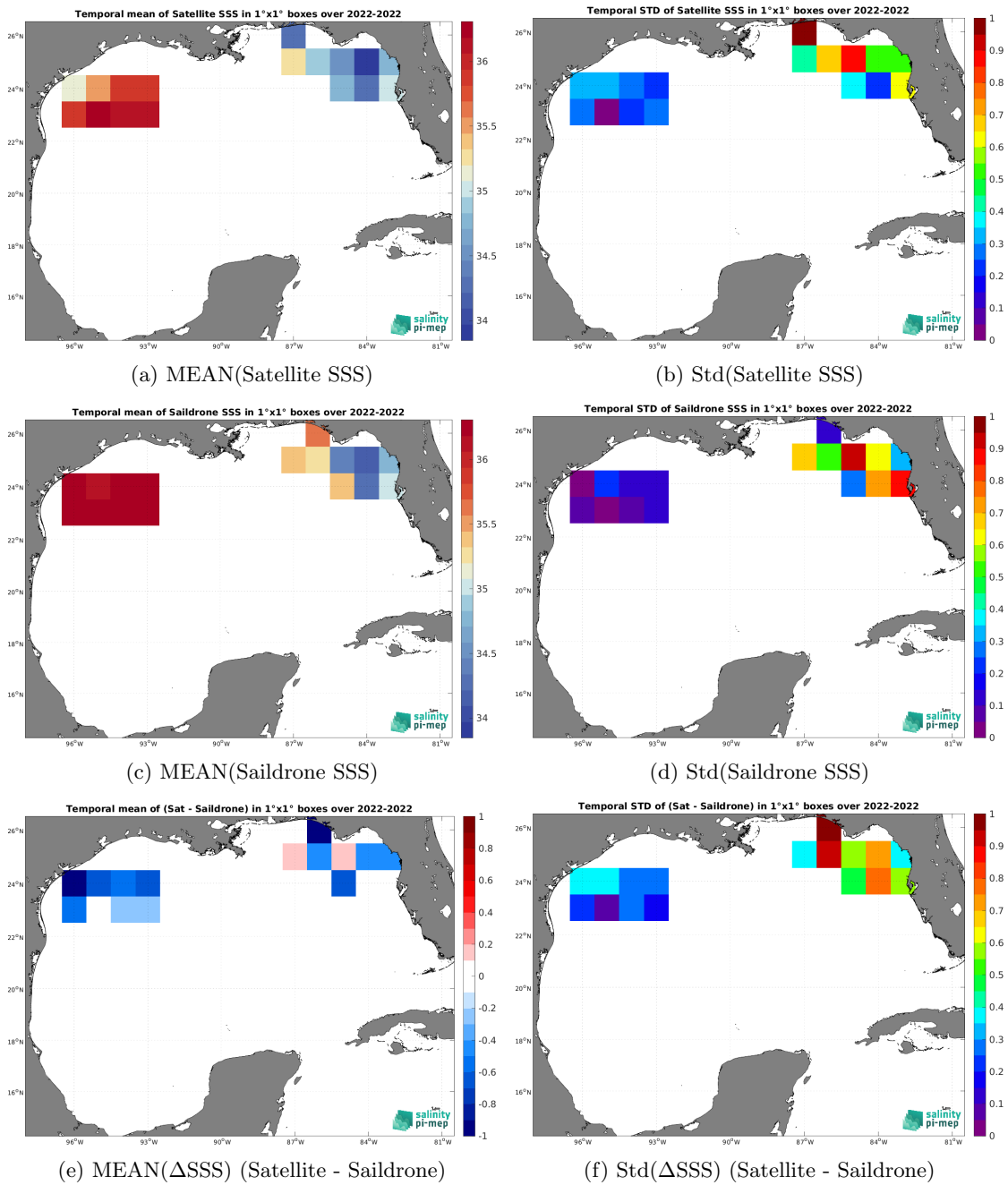
Figure 6: Temporal mean (left) and Std (right) of SSS from SMOS SSS L4 OI v342 - Weekly (CMEMS-CATDS-LOPS) (top), Saildrone (middle), and of \Delta SSS (Satellite - Saildrone). Only match-up pairs are used to generate these maps.
