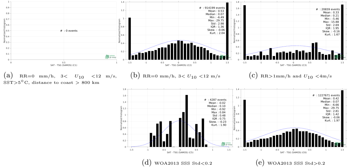
Figure 13: Normalized histogram of \Delta\text{SSS} (SMOS L4 v2 Weekly (CATDS-CECOS-IFREMER) - TSG (SAMOS)) for 5 different subdatasets corresponding to: RR=0 mm/h, 3 < U_{10} < 12 m/s, SST > 5^\circ\text{C} , distance to coast > 800 km (a), RR=0 mm/h, 3 < U_{10} < 12 m/s (b), RR > 1 mm/h and U_{10} < 4 m/s (c), WOA2013 SSS Std < 0.2 (d), WOA2013 SSS Std > 0.2 (e).
