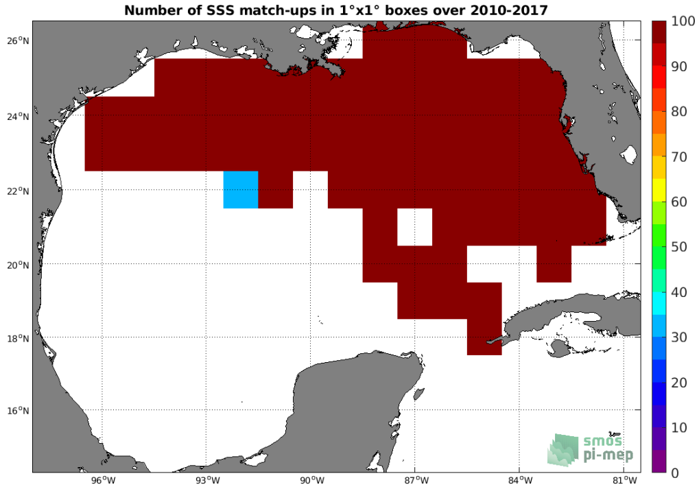
Figure 4: Number of SSS match-ups between TSG (SAMOS) SSS and the SMOS L4 v2 Weekly (CATDS-CECOS-IFREMER) SSS product for the Gulf of Mexico Pi-MEP region over 1°x1° boxes and for the full satellite product period.
