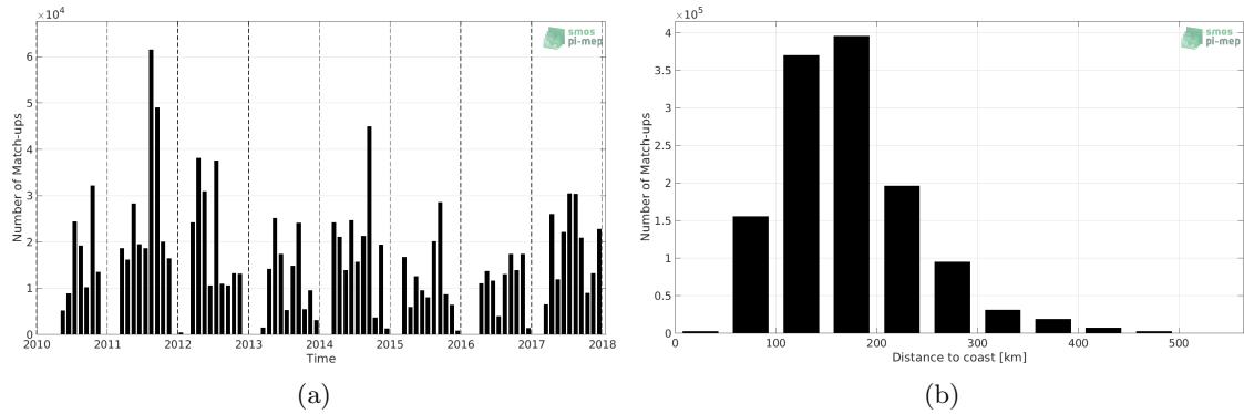
Figure 1: Number of match-ups between TSG (SAMOS) and SMOS L4 v2 Weekly (CATDS-CECOS-IFREMER) SSS as a function of time (a) and as function of the distance to coast (b) over the Gulf of Mexico Pi-MEP region and for the full satellite product period.
