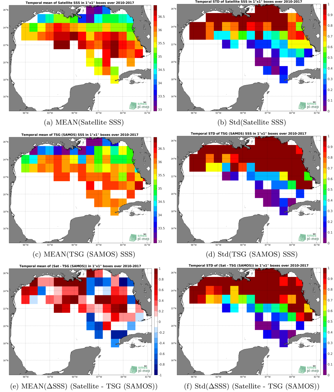
Figure 6: Temporal mean (left) and Std (right) of SSS from SMOS L4 v2 Weekly (CATDS-CECOS-IFREMER) (top), TSG (SAMOS) (middle), and of \Delta SSS (Satellite - TSG (SAMOS)). Only match-up pairs are used to generate these maps.
