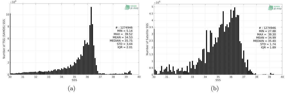
Figure 2: Histograms of SSS from TSG (SAMOS) (a) and SMOS L4 v2 Weekly (CATDS-CECOS-IFREMER) (b) considering all match-up pairs per bins of 0.1 over the Gulf of Mexico Pi-MEP region and for the full satellite product period.
