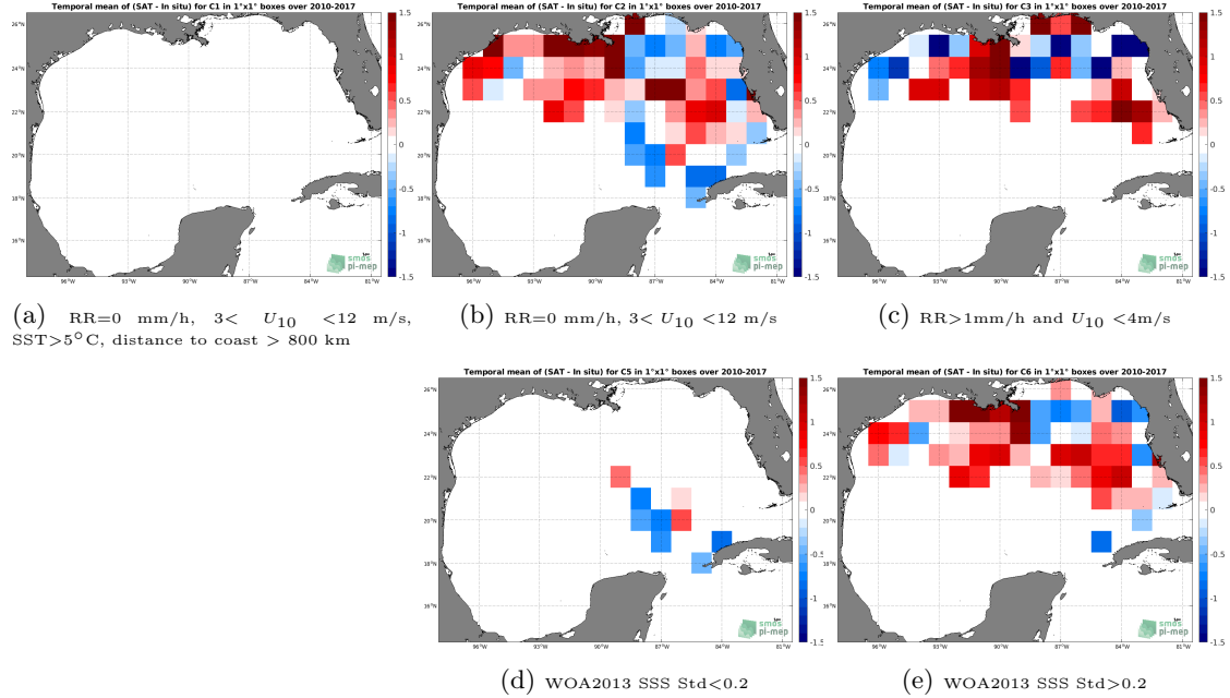
Figure 12: Temporal mean gridded over spatial boxes of size 1^{\circ}\times 1^{\circ} of \Delta\text{SSS} (SMOS L4 v2 Weekly (CATDS-CECOS-IFREMER) - TSG (SAMOS)) for 5 different subdatasets corresponding to:RR=0 mm/h, 3 < U_{10} < 12 m/s, SST >5^{\circ}\text{C} , distance to coast > 800 km (a), RR=0 mm/h, 3 < U_{10} < 12 m/s (b), RR >1 mm/h and U_{10} < 4 m/s (c), WOA2013 SSS Std <0.2 (d), WOA2013 SSS Std >0.2 (e).
