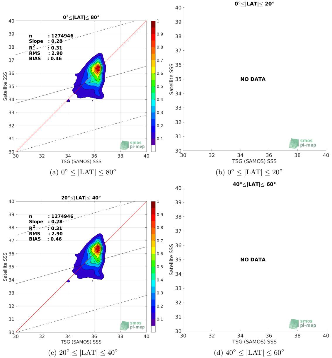
Figure 9: Contour maps of the concentration of SMOS L4 v2 Weekly (CATDS-CECOS-IFREMER) SSS (y-axis) versus TSG (SAMOS) SSS (x-axis) at match-up pairs for different latitude bands. For each plot, the red line shows x=y . The black thin and dashed lines indicate a linear fit through the data cloud and the \pm 95\% confidence levels, respectively. The number match-up pairs n , the slope and R^2 coefficient of the linear fit, the root mean square (RMS) and the mean bias between satellite and in situ data are indicated for each latitude band in each plots.
