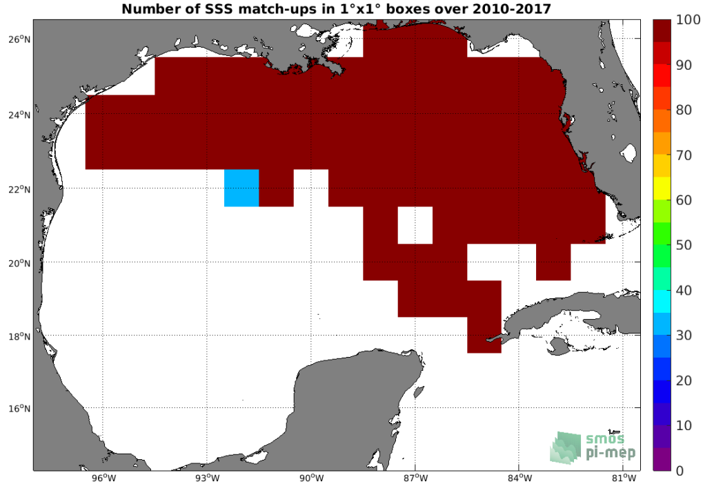
Figure 4: Number of SSS match-ups between TSG (SAMOS) SSS and the SMOS L4 v2 Weekly (CATDS-CECOS-IFREMER) SSS product for the Gulf of Mexico Pi-MEP region over 1^\circ \times 1^\circ boxes and for the full satellite product period.
