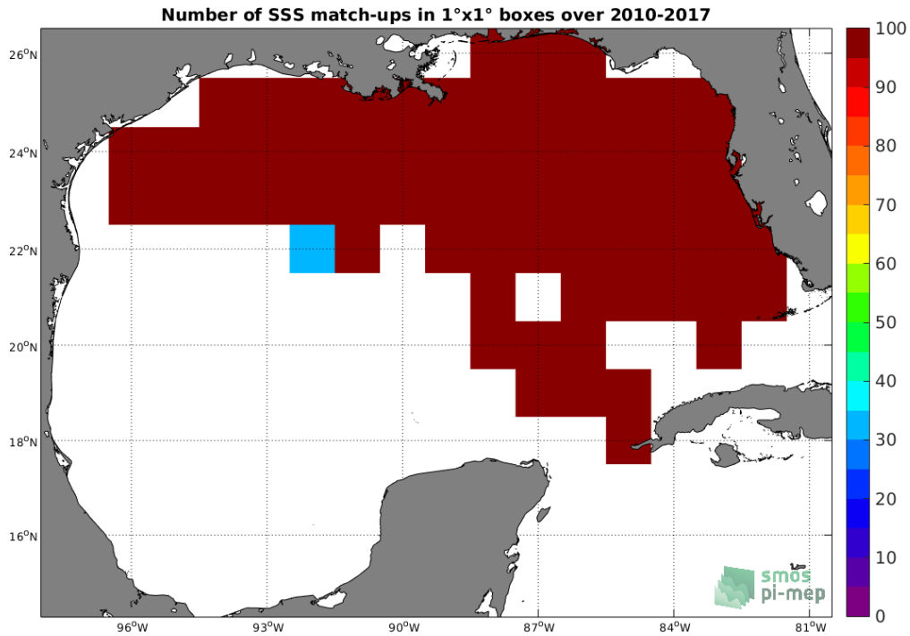
Figure 4: Number of SSS match-ups between TSG-SAMOS SSS and the SMOS-L4-CATDS-CECOS-IFREMER-V2-WEEKLY-0.5DEG SSS product for the Gulf of Mexico Pi-MEP region over 1^\circ \times 1^\circ boxes and for the full satellite product period.
