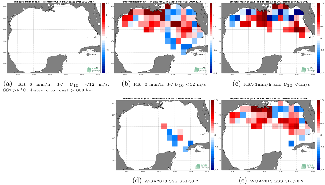
Figure 12: Temporal mean gridded over spatial boxes of size 1^{\circ}\times 1^{\circ} of \Delta\text{SSS} (SMOS-L4-CATDS-CECOS-IFREMER-V2-WEEKLY-0.5DEG - TSG-SAMOS) for 5 different subdatasets corresponding to:RR=0 mm/h, 3 < U_{10} < 12 m/s, SST >5^{\circ}\text{C} , distance to coast > 800 km (a), RR=0 mm/h, 3 < U_{10} < 12 m/s (b), RR >1 mm/h and U_{10} < 4 m/s (c), WOA2013 SSS Std <0.2 (d), WOA2013 SSS Std >0.2 (e).
