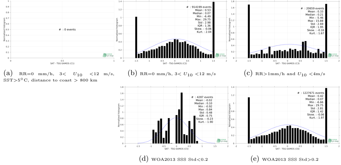
Figure 13: Normalized histogram of \Delta SSS (SMOS-L4-CATDS-CECOS-IFREMER-V2-WEEKLY-0.5DEG - TSG-SAMOS) for 5 different subdatasets corresponding to: RR=0 mm/h, 3 < U_{10} < 12 m/s, SST > 5^\circ C , distance to coast > 800 km (a), RR=0 mm/h, 3 < U_{10} < 12 m/s (b), RR > 1 mm/h and U_{10} < 4 m/s (c), WOA2013 SSS Std < 0.2 (d), WOA2013 SSS Std > 0.2 (e).
