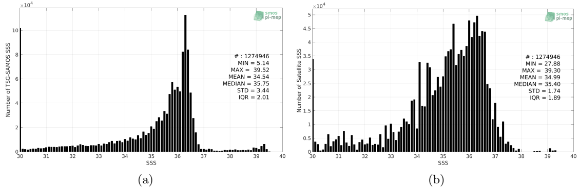
Figure 2: Histograms of SSS from TSG-SAMOS (a) and SMOS-L4-CATDS-CECOS-IFREMER-V2-WEEKLY-0.5DEG (b) considering all match-up pairs per bins of 0.1 over the Gulf of Mexico Pi-MEP region and for the full satellite product period.
