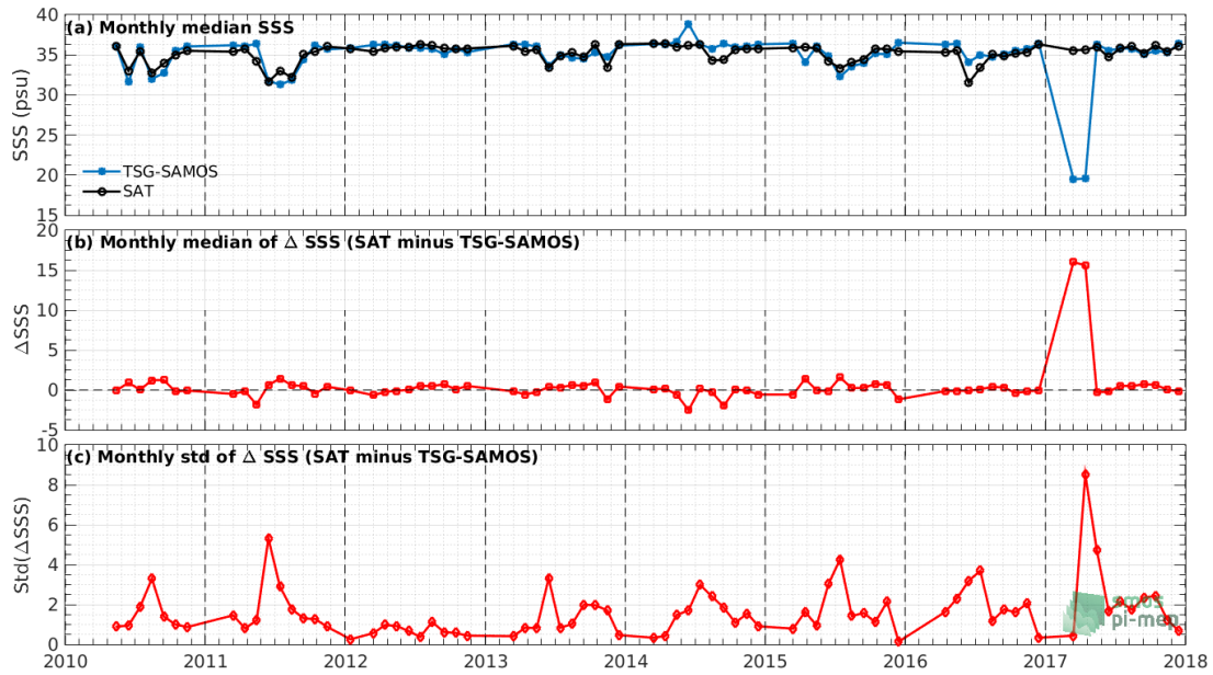
Figure 7: Time series of the monthly median SSS (top), median of \Delta SSS (Satellite - TSG-SAMOS) and Std of \Delta SSS (Satellite - TSG-SAMOS) over the Gulf of Mexico Pi-MEP region considering all match-ups collected by the Pi-MEP.
