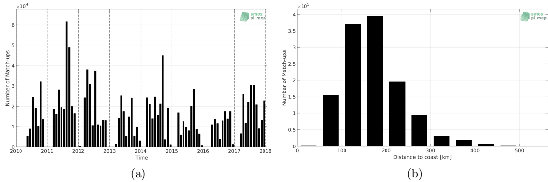
Figure 1: Number of match-ups between TSG-SAMOS and SMOS-L4-CATDS-CECOS-IFREMER-V2-WEEKLY-0.5DEG SSS as a function of time (a) and as function of the distance to coast (b) over the Gulf of Mexico Pi-MEP region and for the full satellite product period.
