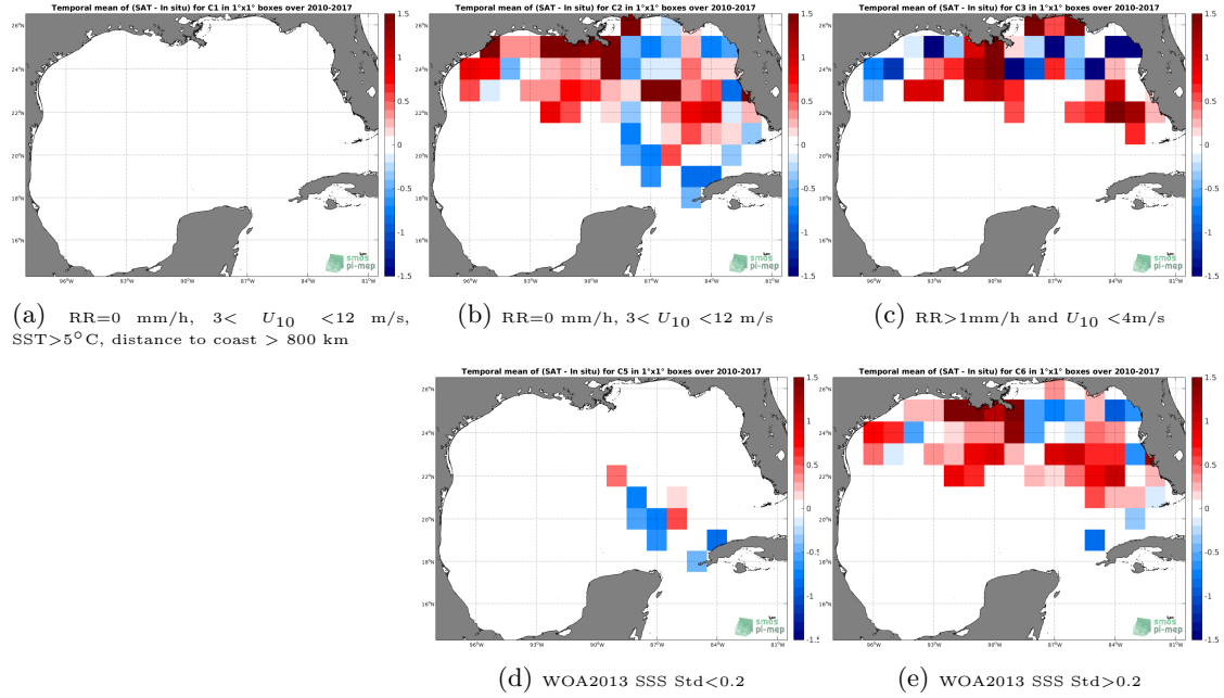
Figure 12: Temporal mean gridded over spatial boxes of size 1^\circ \times 1^\circ of \Delta SSS (SMOS-L4-CATDS-CECOS-IFREMER-V2-WEEKLY-0.5DEG - TSG-SAMOS) for 5 different subdatasets corresponding to: RR=0 mm/h, 3 < U_{10} < 12 m/s, SST >5^\circ C, distance to coast > 800 km (a), RR=0 mm/h, 3 < U_{10} < 12 m/s (b), RR >1 mm/h and U_{10} < 4 m/s (c), WOA2013 SSS Std <0.2 (d), WOA2013 SSS Std >0.2 (e).
