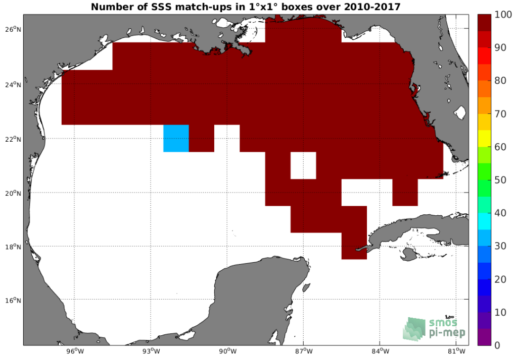
Figure 4: Number of SSS match-ups between TSG-SAMOS SSS and the SMOS-L4-CATDS-CECOS-IFREMER-V2-WEEKLY-0.5DEG SSS product for the Gulf of Mexico Pi-MEP region over 1°x1° boxes and for the full satellite product period.
