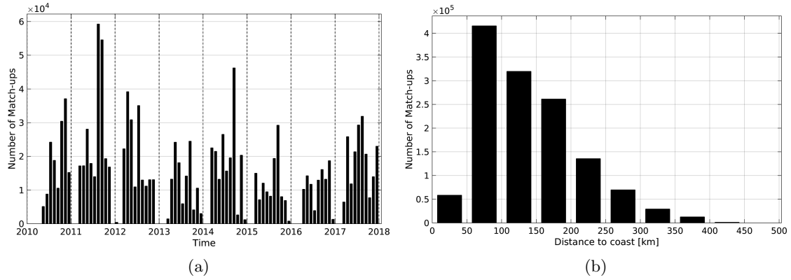
Figure 1: Number of match-ups between TSG-SAMOS and SMOS-L4-CATDS-CECOS-IFREMER-V2-WEEKLY-0.5DEG SSS as a function of time (a) and as function of the distance to coast (b) over the Gulf of Mexico Pi-MEP region and for the full satellite product period.
