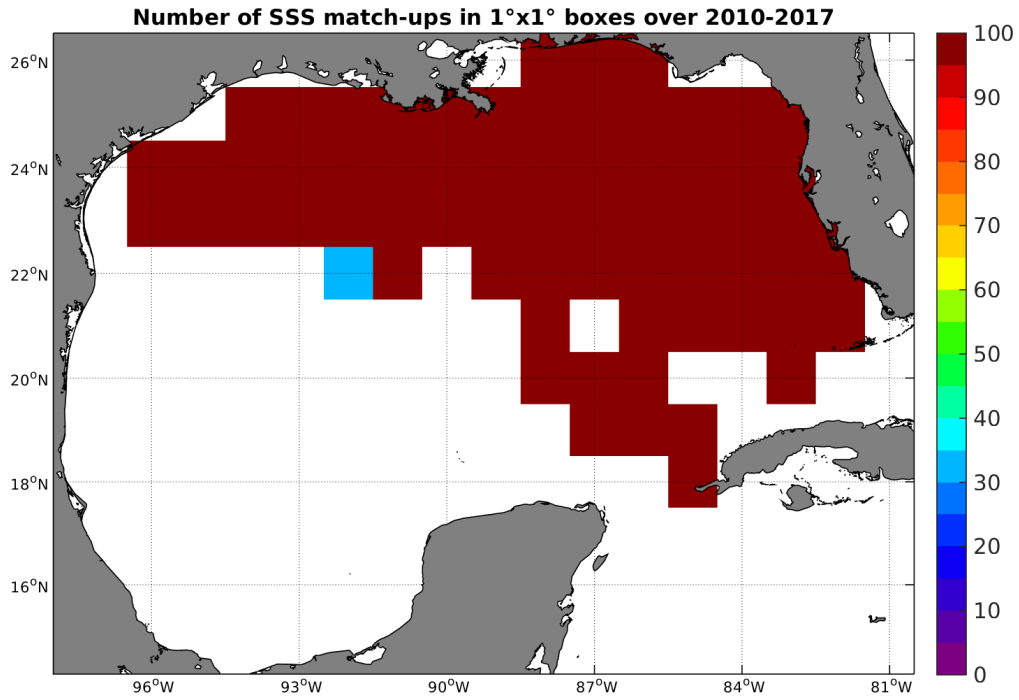
Figure 4: Number of SSS match-ups between TSG-SAMOS SSS and the SMOS-L4-CATDS-CECOS-IFREMER-V2-WEEKLY-0.5DEG SSS product for the Gulf of Mexico Pi-MEP region over 1^\circ \times 1^\circ boxes and for the full satellite product period.
