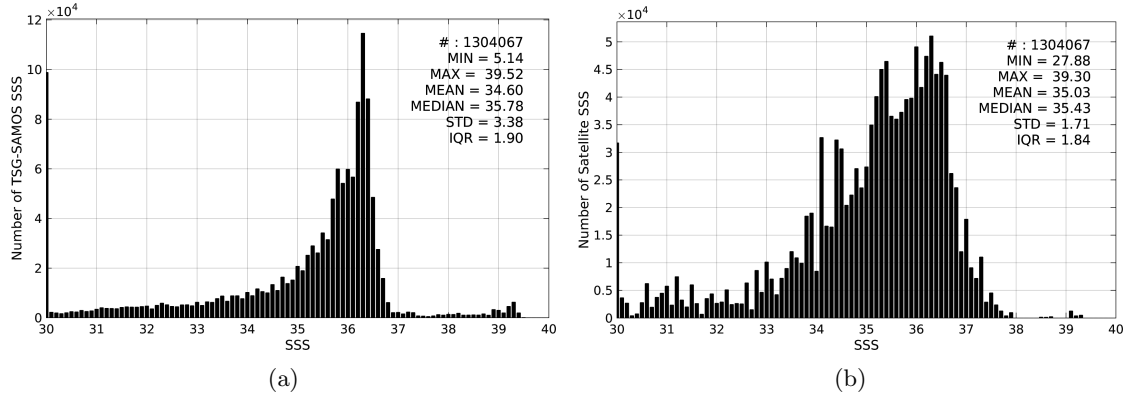
Figure 2: Histograms of SSS from TSG-SAMOS (a) and SMOS-L4-CATDS-CECOS-IFREMER-V2-WEEKLY-0.5DEG (b) considering all match-up pairs per bins of 0.1 over the Gulf of Mexico Pi-MEP region and for the full satellite product period.
