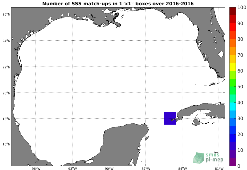
Figure 4: Number of SSS match-ups between TSG (LEGOS-DM) SSS and the SMOS L4 v2 Weekly (CATDS-CECOS-IFREMER) SSS product for the Gulf of Mexico Pi-MEP region over 1°x1° boxes and for the full satellite product period.
