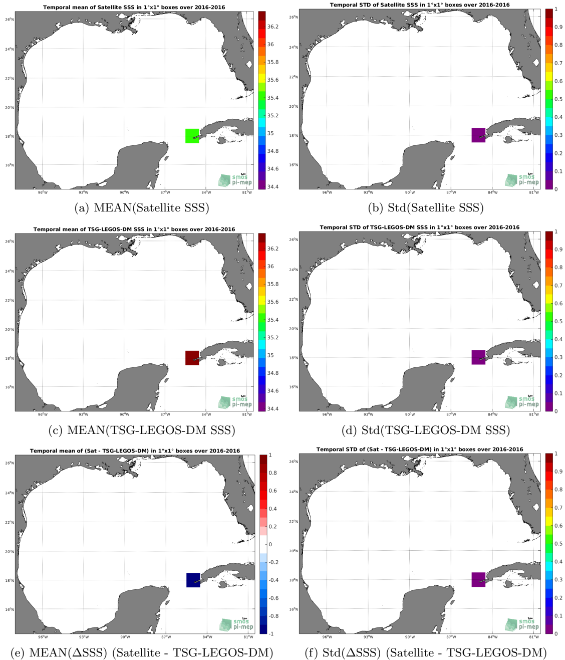
Figure 6: Temporal mean (left) and Std (right) of SSS from SMOS-L4-CATDS-CECOS-IFREMER-V2-WEEKLY-0.5DEG (top), TSG-LEGOS-DM (middle), and of \Delta SSS (Satellite - TSG-LEGOS-DM). Only match-up pairs are used to generate these maps.
