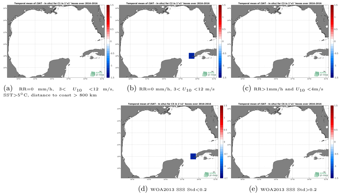
Figure 12: Temporal mean gridded over spatial boxes of size 1^{\circ}\times 1^{\circ} of \Delta\text{SSS} (SMOS-L4-CATDS-CECOS-IFREMER-V2-WEEKLY-0.5DEG - TSG-LEGOS-DM) for 5 different subdatasets corresponding to:RR=0 mm/h, 3 < U_{10} < 12 m/s, SST >5^{\circ}\text{C} , distance to coast > 800 km (a), RR=0 mm/h, 3 < U_{10} < 12 m/s (b), RR >1 mm/h and U_{10} < 4 m/s (c), WOA2013 SSS Std <0.2 (d), WOA2013 SSS Std >0.2 (e).
