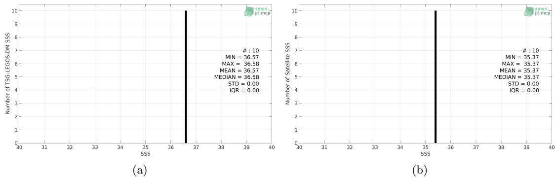
Figure 2: Histograms of SSS from TSG-LEGOS-DM (a) and SMOS-L4-CATDS-CECOS-IFREMER-V2-WEEKLY-0.5DEG (b) considering all match-up pairs per bins of 0.1 over the Gulf of Mexico Pi-MEP region and for the full satellite product period.
