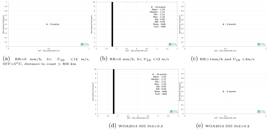
Figure 13: Normalized histogram of \Delta\text{SSS} (SMOS-L4-CATDS-CECOS-IFREMER-V2-WEEKLY-0.5DEG - TSG-LEGOS-DM) for 5 different subdatasets corresponding to: RR=0 mm/h, 3 < U_{10} < 12 m/s, SST > 5^\circ\text{C} , distance to coast > 800 km (a), RR=0 mm/h, 3 < U_{10} < 12 m/s (b), RR > 1\text{mm/h} and U_{10} < 4\text{m/s} (c), WOA2013 SSS Std < 0.2 (d), WOA2013 SSS Std > 0.2 (e).
