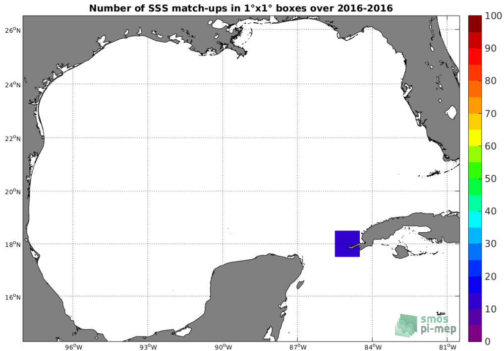
Figure 4: Number of SSS match-ups between TSG-LEGOS-DM SSS and the SMOS-L4-CATDS-CECOS-IFREMER-V2-WEEKLY-0.5DEG SSS product for the Gulf of Mexico Pi-MEP region over 1°x1° boxes and for the full satellite product period.
