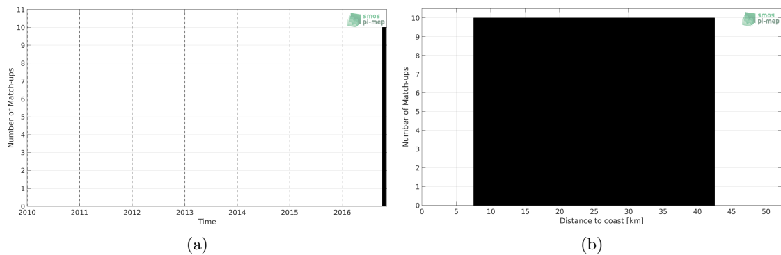
Figure 1: Number of match-ups between TSG-LEGOS-DM and SMOS-L4-CATDS-CECOS-IFREMER-V2-WEEKLY-0.5DEG SSS as a function of time (a) and as function of the distance to coast (b) over the Gulf of Mexico Pi-MEP region and for the full satellite product period.
