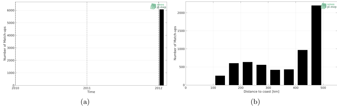
Figure 1: Number of match-ups between TSG (GOSUD-Sailing-ship) and SMOS L4 v2 Weekly (CATDS-CECOS-IFREMER) SSS as a function of time (a) and as function of the distance to coast (b) over the Gulf of Mexico Pi-MEP region and for the full satellite product period.
