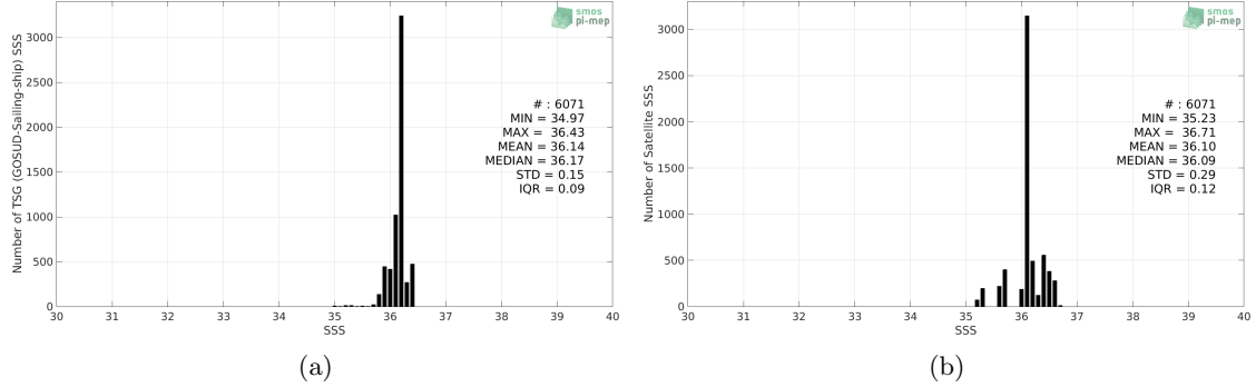
Figure 2: Histograms of SSS from TSG (GOSUD-Sailing-ship) (a) and SMOS L4 v2 Weekly (CATDS-CECOS-IFREMER) (b) considering all match-up pairs per bins of 0.1 over the Gulf of Mexico Pi-MEP region and for the full satellite product period.
