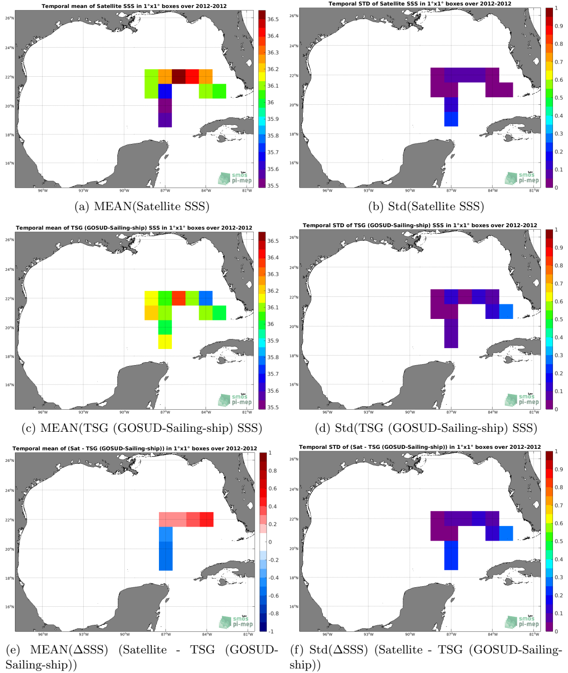
Figure 6: Temporal mean (left) and Std (right) of SSS from SMOS L4 v2 Weekly (CATDS-CECOS-IFREMER) (top), TSG (GOSUD-Sailing-ship) (middle), and of \Delta SSS (Satellite - TSG (GOSUD-Sailing-ship)). Only match-up pairs are used to generate these maps.
