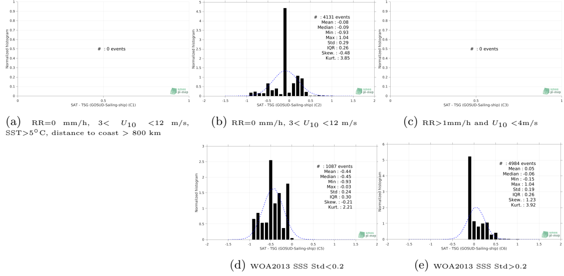
Figure 13: Normalized histogram of \Delta\text{SSS} (SMOS L4 v2 Weekly (CATDS-CECOS-IFREMER) - TSG (GOSUD-Sailing-ship)) for 5 different subdatasets corresponding to: RR=0 mm/h, 3 < U_{10} < 12 m/s, SST > 5^\circ\text{C} , distance to coast > 800 km (a), RR=0 mm/h, 3 < U_{10} < 12 m/s (b), RR > 1\text{mm/h} and U_{10} < 4\text{m/s} (c), WOA2013 SSS Std < 0.2 (d), WOA2013 SSS Std > 0.2 (e).
