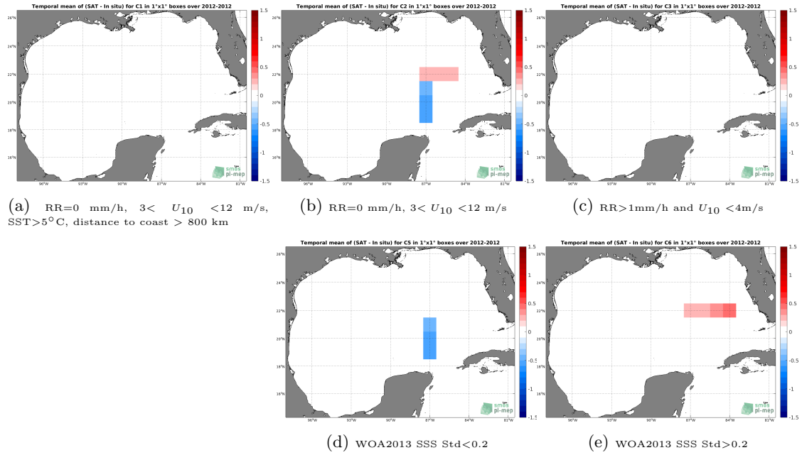
Figure 12: Temporal mean gridded over spatial boxes of size 1^\circ \times 1^\circ of \Delta SSS (SMOS L4 v2 Weekly (CATDS-CECOS-IFREMER) - TSG (GOSUD-Sailing-ship)) for 5 different subdatasets corresponding to: RR=0 mm/h, 3 < U_{10} < 12 m/s, SST >5^\circ\text{C} , distance to coast > 800 km (a), RR=0 mm/h, 3 < U_{10} < 12 m/s (b), RR >1 mm/h and U_{10} < 4 m/s (c), WOA2013 SSS Std <0.2 (d), WOA2013 SSS Std >0.2 (e).
