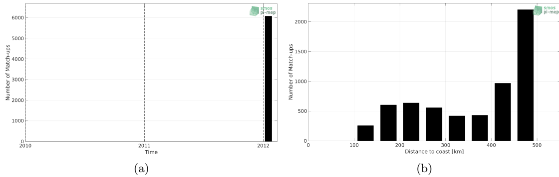
Figure 1: Number of match-ups between TSG-GOSUD-Sailing-ship and SMOS-L4-CATDS-CECOS-IFREMER-V2-WEEKLY-0.5DEG SSS as a function of time (a) and as function of the distance to coast (b) over the Gulf of Mexico Pi-MEP region and for the full satellite product period.
