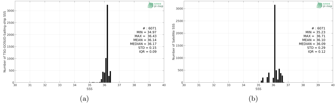
Figure 2: Histograms of SSS from TSG-GOSUD-Sailing-ship (a) and SMOS-L4-CATDS-CECOS-IFREMER-V2-WEEKLY-0.5DEG (b) considering all match-up pairs per bins of 0.1 over the Gulf of Mexico Pi-MEP region and for the full satellite product period.
