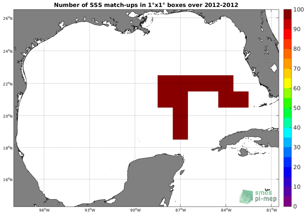
Figure 4: Number of SSS match-ups between TSG-GOSUD-Sailing-ship SSS and the SMOS-L4-CATDS-CECOS-IFREMER-V2-WEEKLY-0.5DEG SSS product for the Gulf of Mexico Pi-MEP region over 1°x1° boxes and for the full satellite product period.
