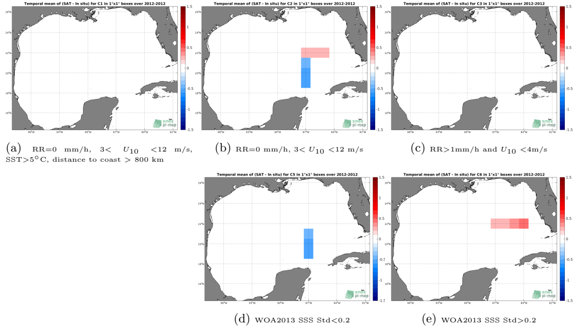
Figure 12: Temporal mean gridded over spatial boxes of size 1^\circ \times 1^\circ of \Delta SSS (SMOS-L4-CATDS-CECOS-IFREMER-V2-WEEKLY-0.5DEG - TSG-GOSUD-Sailing-ship) for 5 different subdatasets corresponding to:RR=0 mm/h, 3 < U_{10} < 12 m/s, SST >5^\circ\text{C} , distance to coast > 800 km (a), RR=0 mm/h, 3 < U_{10} < 12 m/s (b), RR >1 mm/h and U_{10} < 4 m/s (c), WOA2013 SSS Std <0.2 (d), WOA2013 SSS Std >0.2 (e).
