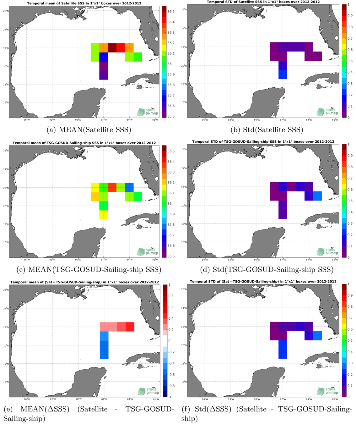
Figure 6: Temporal mean (left) and Std (right) of SSS from SMOS-L4-CATDS-CECOS-IFREMER-V2-WEEKLY-0.5DEG (top), TSG-GOSUD-Sailing-ship (middle), and of \Delta SSS (Satellite - TSG-GOSUD-Sailing-ship). Only match-up pairs are used to generate these maps.
