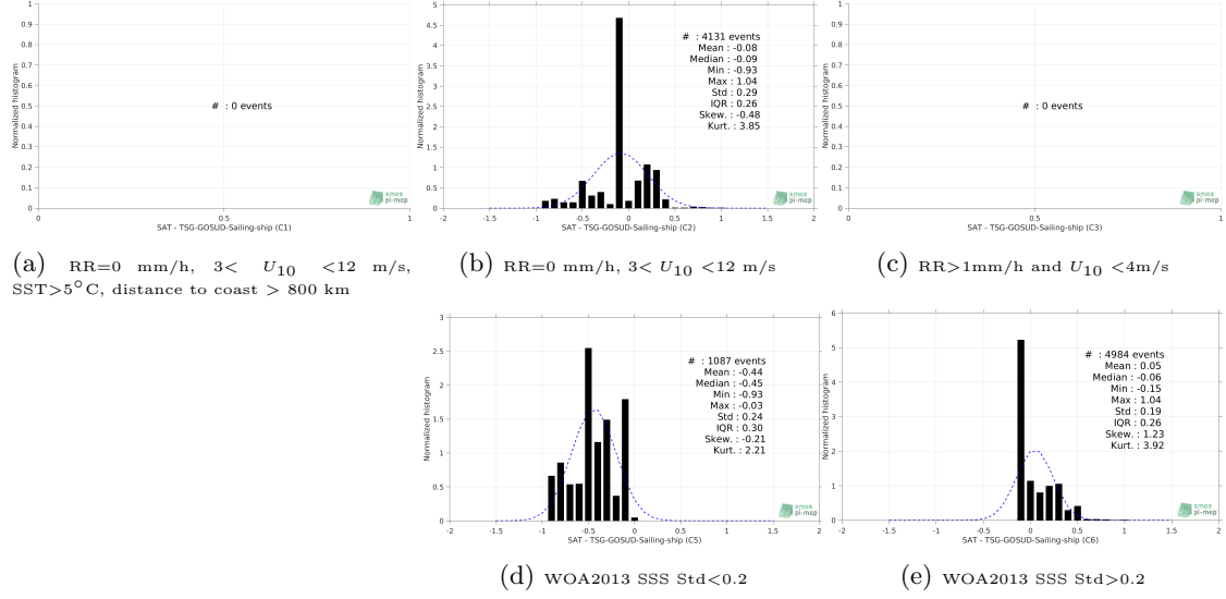
Figure 13: Normalized histogram of \Delta\text{SSS} (SMOS-L4-CATDS-CECOS-IFREMER-V2-WEEKLY-0.5DEG - TSG-GOSUD-Sailing-ship) for 5 different subdatasets corresponding to: RR=0 mm/h, 3 < U_{10} < 12 m/s, SST > 5^{\circ}\text{C} , distance to coast > 800 km (a), RR=0 mm/h, 3 < U_{10} < 12 m/s (b), RR > 1\text{mm/h} and U_{10} < 4\text{m/s} (c), WOA2013 SSS Std < 0.2 (d), WOA2013 SSS Std > 0.2 (e).
