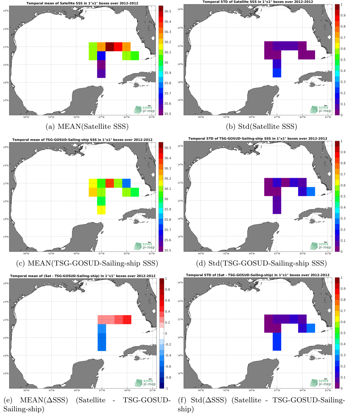
Figure 6: Temporal mean (left) and Std (right) of SSS from SMOS-L4-CATDS-CECOS-IFREMER-V2-WEEKLY-0.5DEG (top), TSG-GOSUD-Sailing-ship (middle), and of \Delta SSS (Satellite - TSG-GOSUD-Sailing-ship). Only match-up pairs are used to generate these maps.
