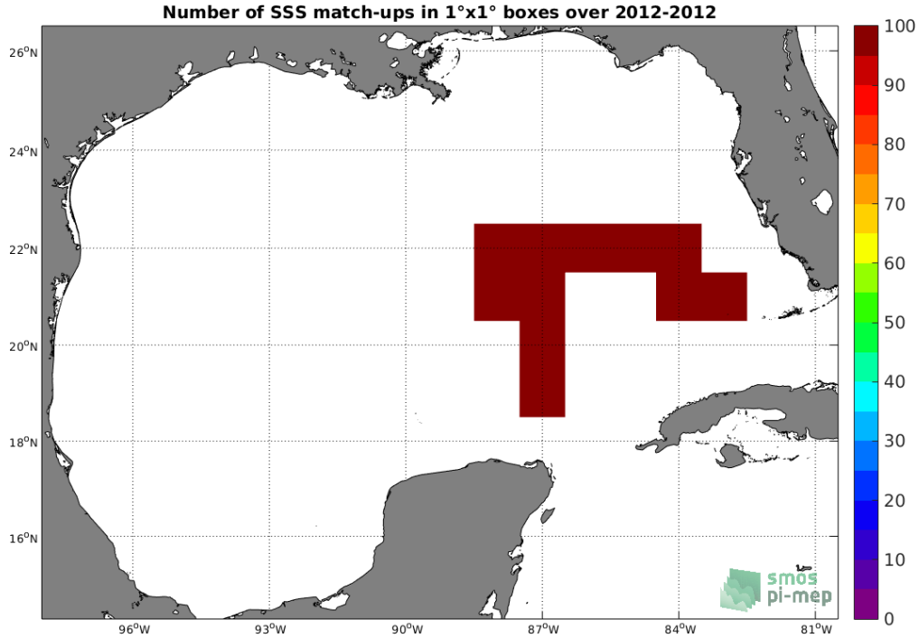
Figure 4: Number of SSS match-ups between TSG-GOSUD-Sailing-ship SSS and the SMOS-L4-CATDS-CECOS-IFREMER-V2-WEEKLY-0.5DEG SSS product for the Gulf of Mexico Pi-MEP region over 1^\circ \times 1^\circ boxes and for the full satellite product period.
