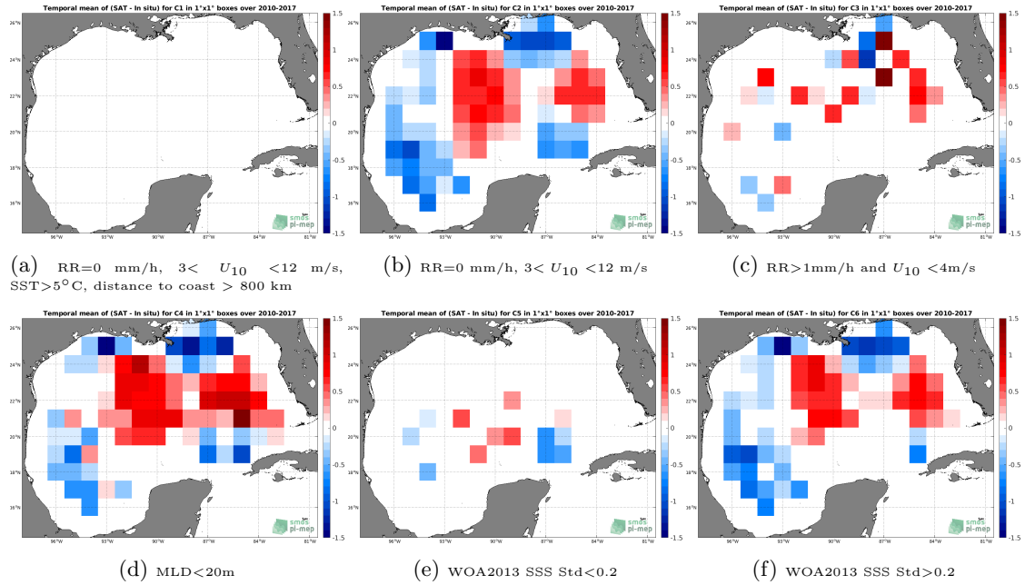
Figure 12: Temporal mean gridded over spatial boxes of size 1^\circ \times 1^\circ of \Delta SSS (SMOS L4 v2 Weekly (CATDS-CECOS-IFREMER) - Argo) for 6 different subdatasets corresponding to:RR=0 mm/h, 3 < U_{10} < 12 m/s, SST >5^\circ\text{C} , distance to coast > 800 km (a), RR=0 mm/h, 3 < U_{10} < 12 m/s (b), RR >1 mm/h and U_{10} < 4 m/s (c),MLD <20 m (d),WOA2013 SSS Std <0.2 (e),WOA2013 SSS Std >0.2 (f).
