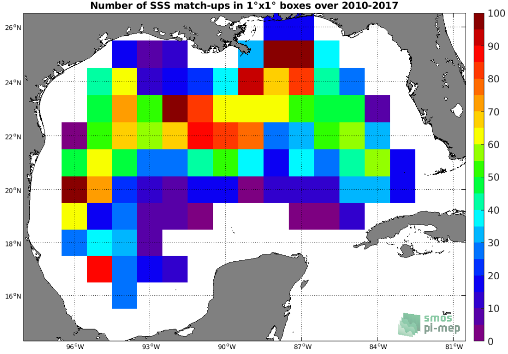
Figure 4: Number of SSS match-ups between Argo SSS and the SMOS L4 v2 Weekly (CATDS-CECOS-IFREMER) SSS product for the Gulf of Mexico Pi-MEP region over 1°x1° boxes and for the full satellite product period.
