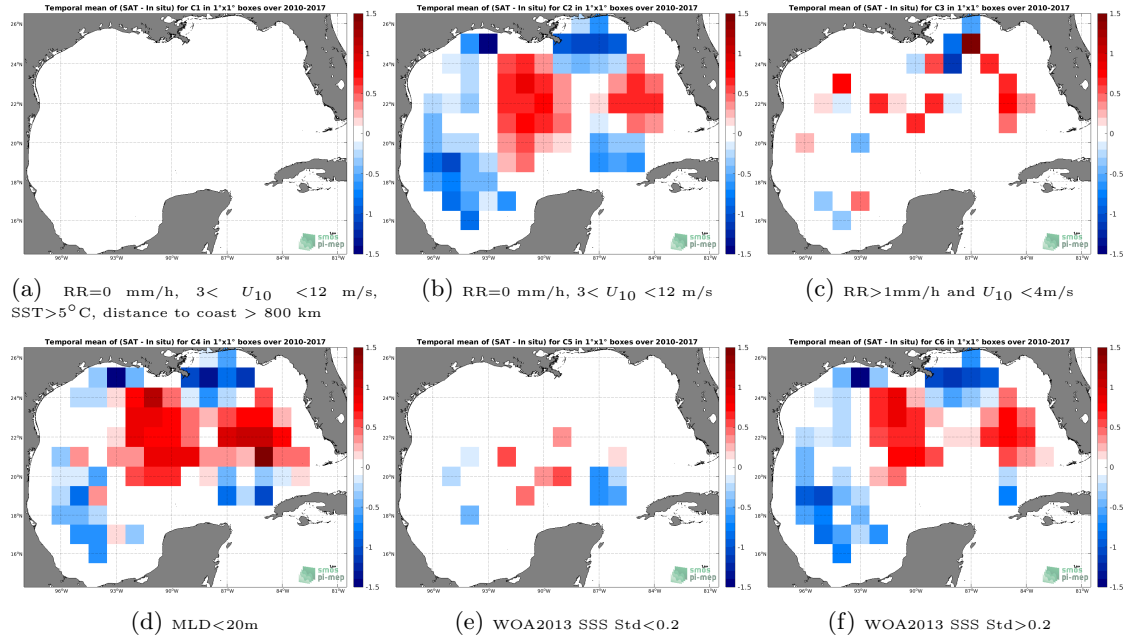
Figure 12: Temporal mean gridded over spatial boxes of size 1^\circ \times 1^\circ of \Delta SSS (SMOS L4 v2 Weekly (CATDS-CECOS-IFREMER) - Argo) for 6 different subdatasets corresponding to: RR=0 mm/h, 3 < U_{10} < 12 m/s, SST > 5^\circ C , distance to coast > 800 km (a), RR=0 mm/h, 3 < U_{10} < 12 m/s (b), RR > 1 mm/h and U_{10} < 4 m/s (c), MLD < 20 m (d), WOA2013 SSS Std < 0.2 (e), WOA2013 SSS Std > 0.2 (f).
