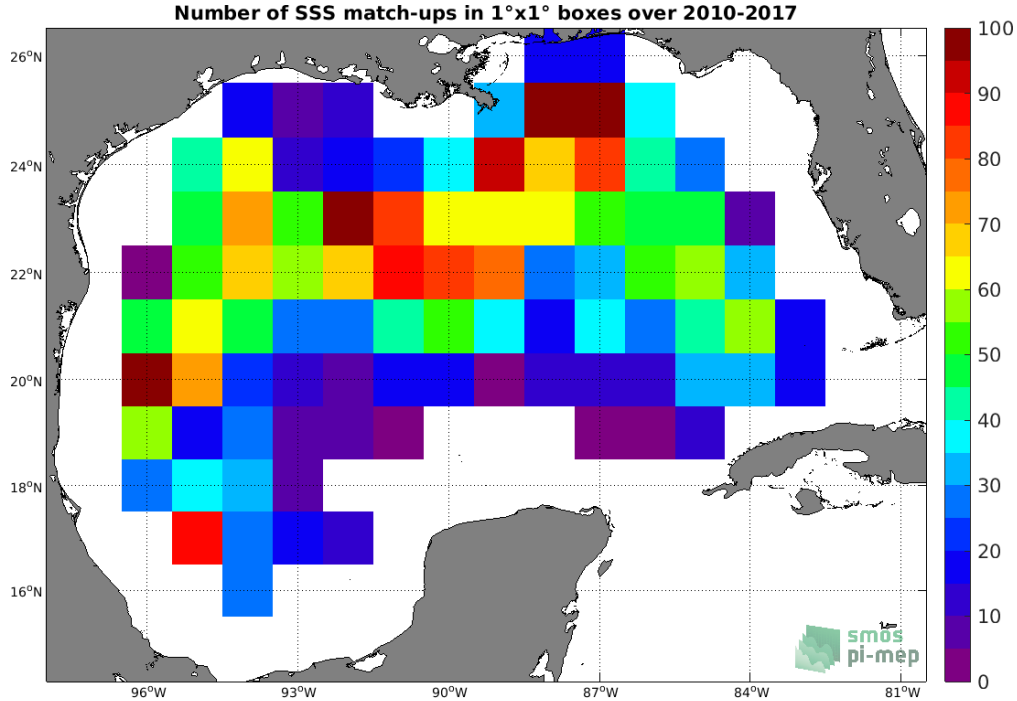
Figure 4: Number of SSS match-ups between Argo SSS and the SMOS L4 v2 Weekly (CATDS-CECOS-IFREMER) SSS product for the Gulf of Mexico Pi-MEP region over 1^\circ \times 1^\circ boxes and for the full satellite product period.
