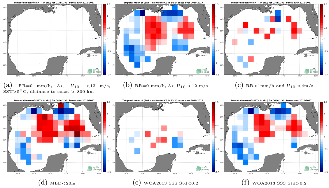
Figure 12: Temporal mean gridded over spatial boxes of size 1^\circ \times 1^\circ of \Delta SSS (SMOS-L4-CATDS-CECOS-IFREMER-V2-WEEKLY-0.5DEG - Argo) for 6 different subdatasets corresponding to: RR=0 mm/h, 3 < U_{10} < 12 m/s, SST >5^\circ C, distance to coast > 800 km (a), RR=0 mm/h, 3 < U_{10} < 12 m/s (b), RR >1 mm/h and U_{10} < 4 m/s (c),MLD <20 m (d),WOA2013 SSS Std <0.2 (e),WOA2013 SSS Std >0.2 (f).
