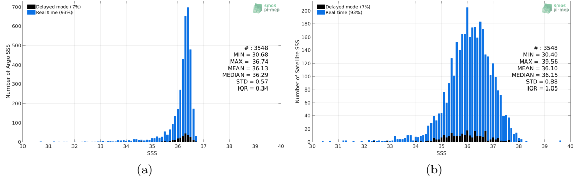
Figure 2: Histograms of SSS from Argo (a) and SMOS-L4-CATDS-CECOS-IFREMER-V2-WEEKLY-0.5DEG (b) considering all match-up pairs per bins of 0.1 over the Gulf of Mexico Pi-MEP region and for the full satellite product period.
