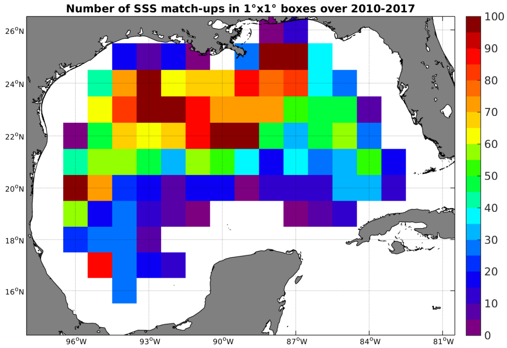
Figure 4: Number of SSS match-ups between Argo SSS and the SMOS-L4-CATDS-CECOS-IFREMER-V2-WEEKLY-0.5DEG SSS product for the Gulf of Mexico Pi-MEP region over 1^\circ \times 1^\circ boxes and for the full satellite product period.
