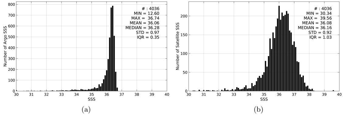
Figure 2: Histograms of SSS from Argo (a) and SMOS-L4-CATDS-CECOS-IFREMER-V2-WEEKLY-0.5DEG (b) considering all match-up pairs per bins of 0.1 over the Gulf of Mexico Pi-MEP region and for the full satellite product period.
