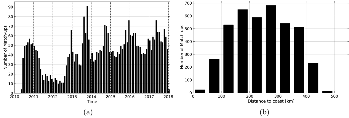
Figure 1: Number of match-ups between Argo and SMOS-L4-CATDS-CECOS-IFREMER-V2-WEEKLY-0.5DEG SSS as a function of time (a) and as function of the distance to coast (b) over the Gulf of Mexico Pi-MEP region and for the full satellite product period.
