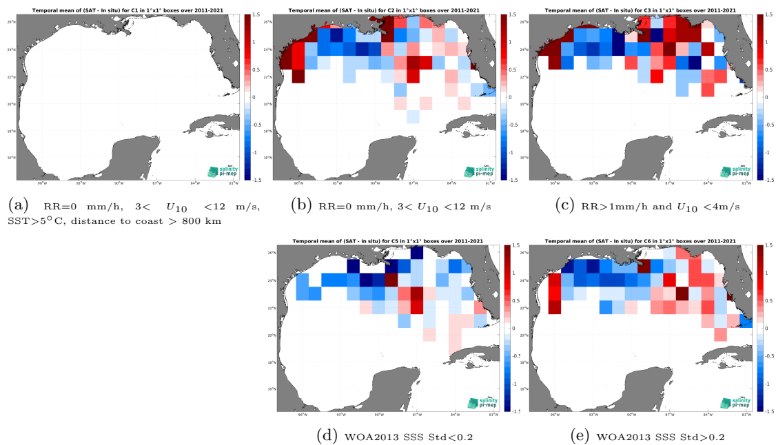
Figure 14: Temporal mean gridded over spatial boxes of size 1^\circ \times 1^\circ of \Delta SSS (SMOS SSS L4 v2 - Daily (BEC) - TSG (SAMOS)) for 5 different subdatasets corresponding to:RR=0 mm/h, 3 < U_{10} < 12 m/s, SST >5^\circ C, distance to coast > 800 km (a), RR=0 mm/h, 3 < U_{10} < 12 m/s (b), RR >1 mm/h and U_{10} < 4 m/s (c), WOA2013 SSS Std <0.2 (d), WOA2013 SSS Std >0.2 (e).
