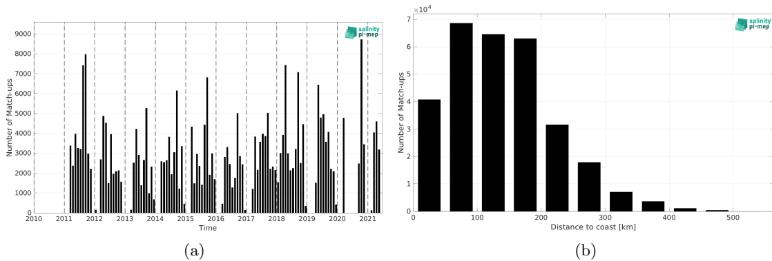
Figure 2: Number of match-ups between TSG (SAMOS) and SMOS SSS L4 v2 - Daily (BEC) SSS as a function of time (a) and as function of the distance to coast (b) over the Gulf of Mexico Pi-MEP region and for the full satellite product period.
