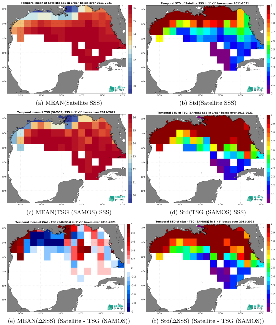
Figure 7: Temporal mean (left) and Std (right) of SSS from SMOS SSS L4 v2 - Daily (BEC) (top), TSG (SAMOS) (middle), and of \Delta SSS (Satellite - TSG (SAMOS)). Only match-up pairs are used to generate these maps.
