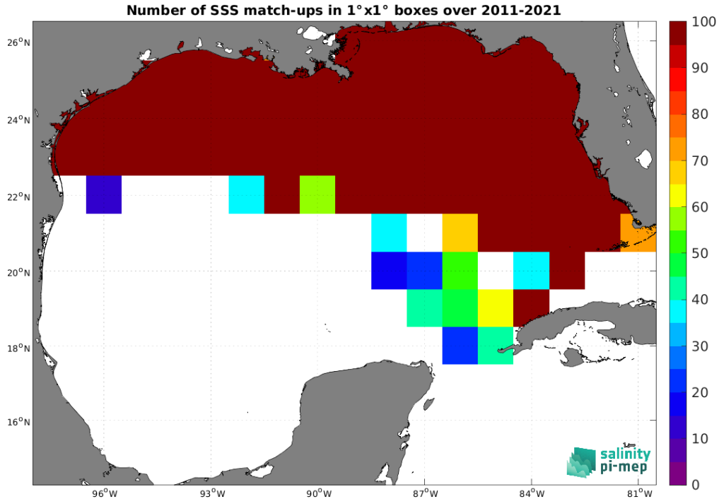
Figure 5: Number of SSS match-ups between TSG (SAMOS) SSS and the SMOS SSS L4 v2 - Daily (BEC) SSS product for the Gulf of Mexico Pi-MEP region over 1^\circ \times 1^\circ boxes and for the full satellite product period.
