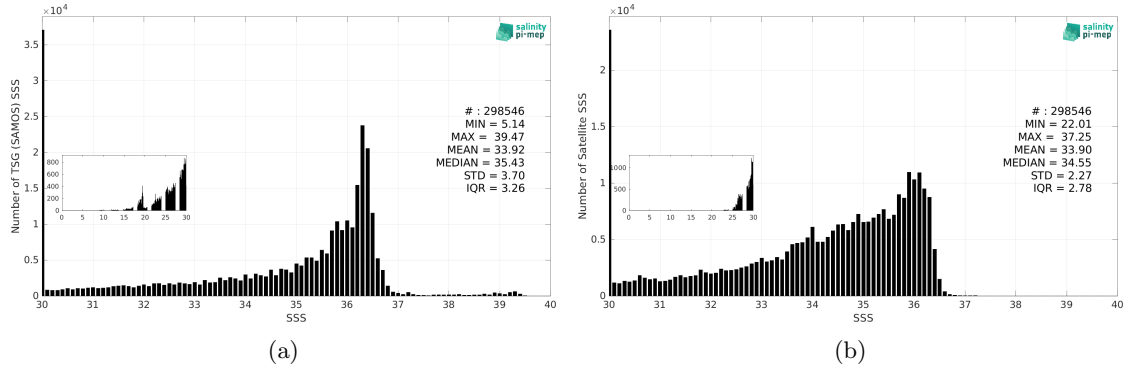
Figure 3: Histograms of SSS from TSG (SAMOS) (a) and SMOS SSS L4 v2 - Daily (BEC) (b) considering all match-up pairs per bins of 0.1 over the Gulf of Mexico Pi-MEP region and for the full satellite product period.
