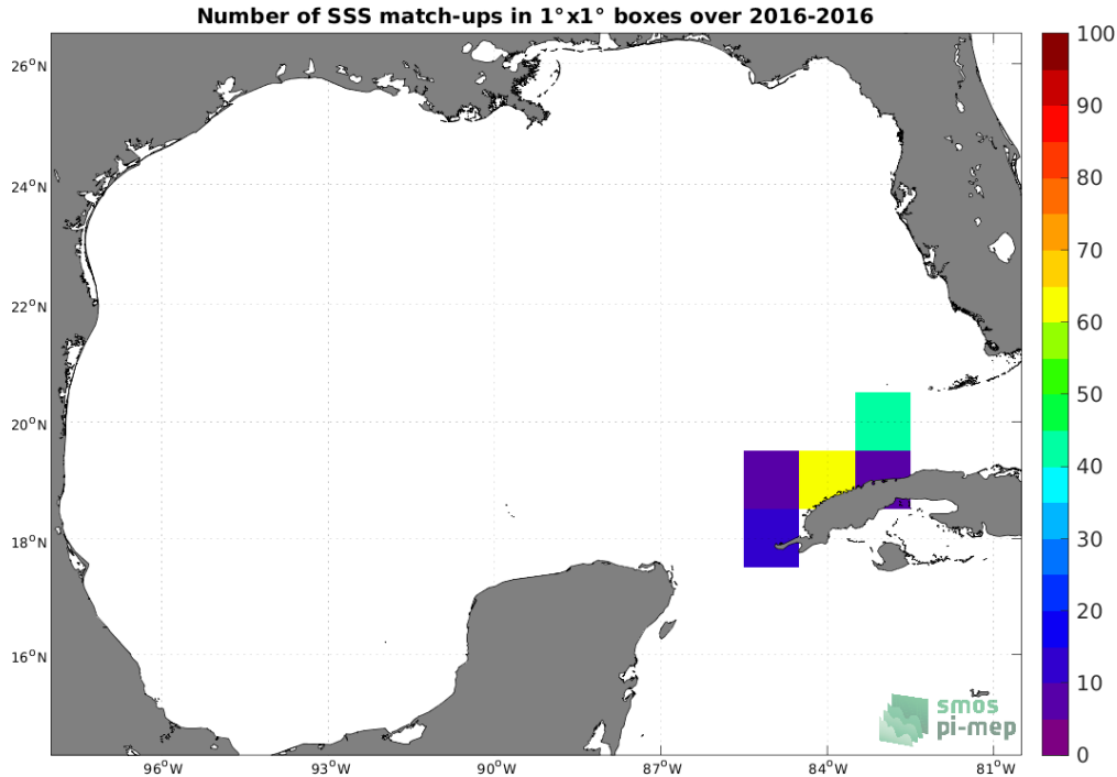
Figure 4: Number of SSS match-ups between TSG (LEGOS-DM) SSS and the SMOS SSS L4 v2 - Daily (BEC) SSS product for the Gulf of Mexico Pi-MEP region over 1^\circ \times 1^\circ boxes and for the full satellite product period.
