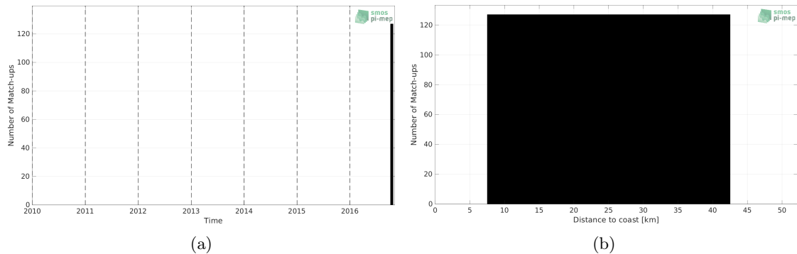
Figure 1: Number of match-ups between TSG (LEGOS-DM) and SMOS SSS L4 v2 - Daily (BEC) SSS as a function of time (a) and as function of the distance to coast (b) over the Gulf of Mexico Pi-MEP region and for the full satellite product period.
