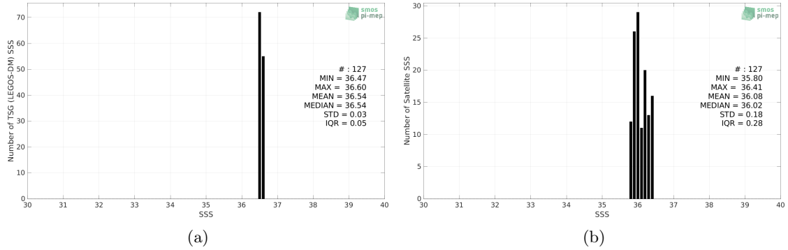
Figure 2: Histograms of SSS from TSG (LEGOS-DM) (a) and SMOS SSS L4 v2 - Daily (BEC) (b) considering all match-up pairs per bins of 0.1 over the Gulf of Mexico Pi-MEP region and for the full satellite product period.
