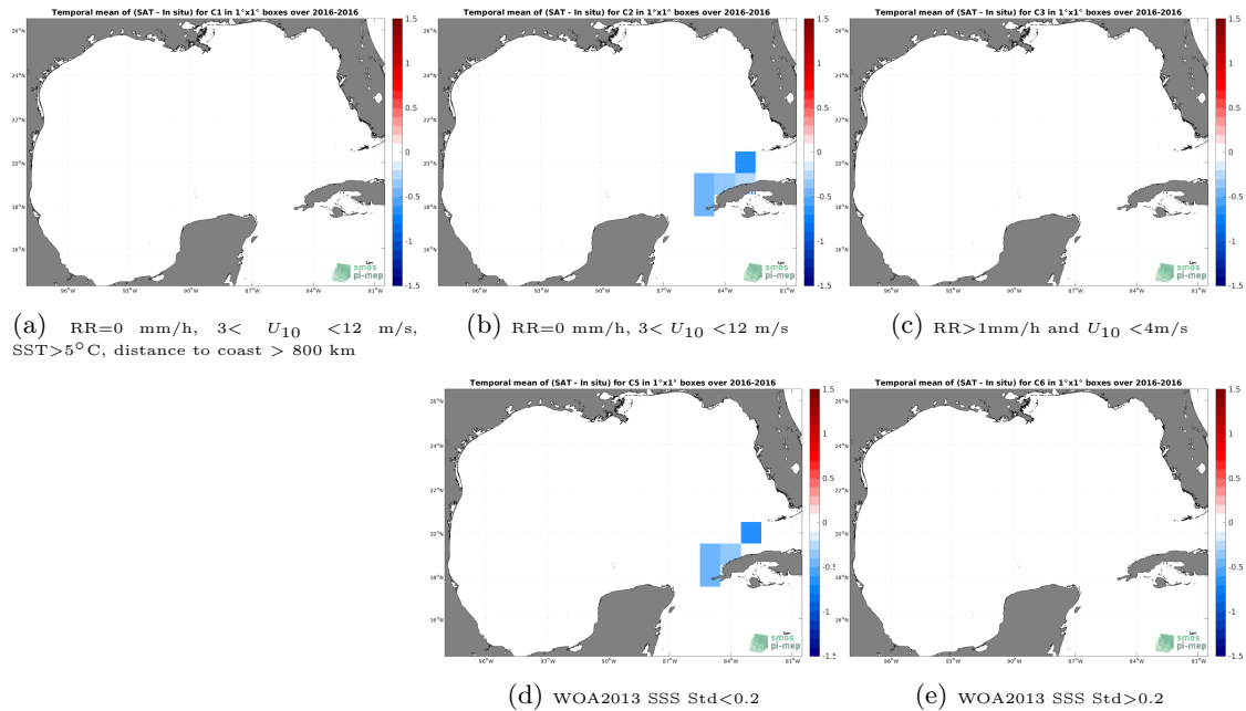
Figure 12: Temporal mean gridded over spatial boxes of size 1^{\circ}\times 1^{\circ} of \Delta\text{SSS} (SMOS SSS L4 v2 - Daily (BEC) - TSG (LEGOS-DM)) for 5 different subdatasets corresponding to:RR=0 mm/h, 3 < U_{10} < 12 m/s, SST >5^{\circ}\text{C} , distance to coast > 800 km (a), RR=0 mm/h, 3 < U_{10} < 12 m/s (b), RR >1 mm/h and U_{10} < 4 m/s (c), WOA2013 SSS Std <0.2 (d), WOA2013 SSS Std >0.2 (e).
