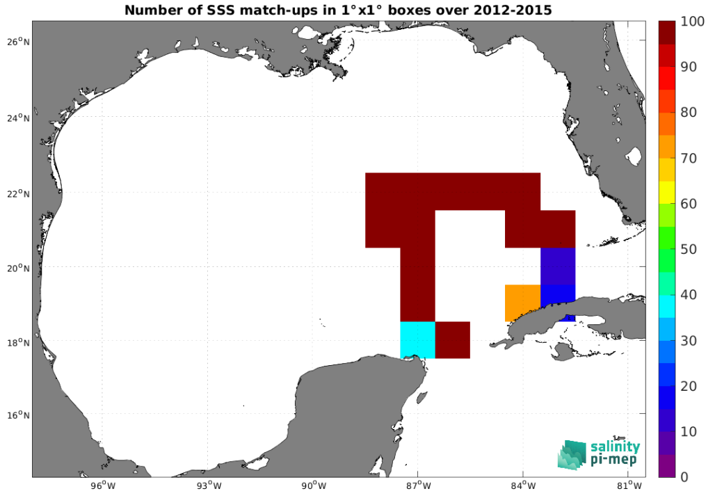
Figure 5: Number of SSS match-ups between TSG (GOSUD-Sailing-ship) SSS and the SMOS SSS L4 v2 - Daily (BEC) SSS product for the Gulf of Mexico Pi-MEP region over 1^\circ \times 1^\circ boxes and for the full satellite product period.
