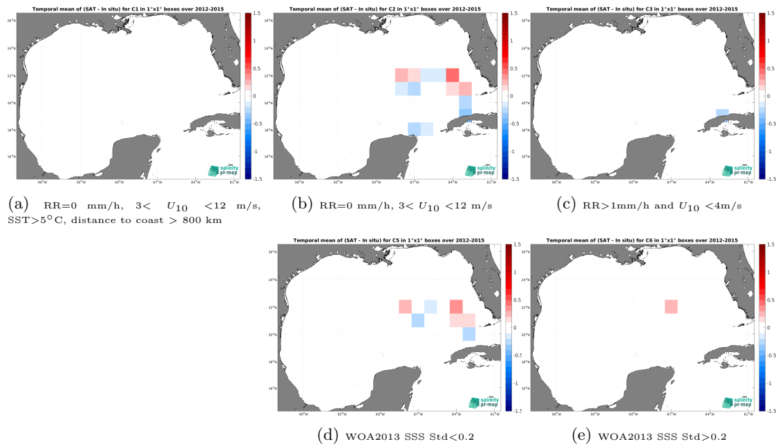
Figure 14: Temporal mean gridded over spatial boxes of size 1^\circ \times 1^\circ of \Delta SSS (SMOS SSS L4 v2 - Daily (BEC) - TSG (GOSUD-Sailing-ship)) for 5 different subdatasets corresponding to:RR=0 mm/h, 3 < U_{10} < 12 m/s, SST > 5^\circ\text{C} , distance to coast > 800 km (a), RR=0 mm/h, 3 < U_{10} < 12 m/s (b), RR > 1 mm/h and U_{10} < 4 m/s (c), WOA2013 SSS Std < 0.2 (d), WOA2013 SSS Std > 0.2 (e).
