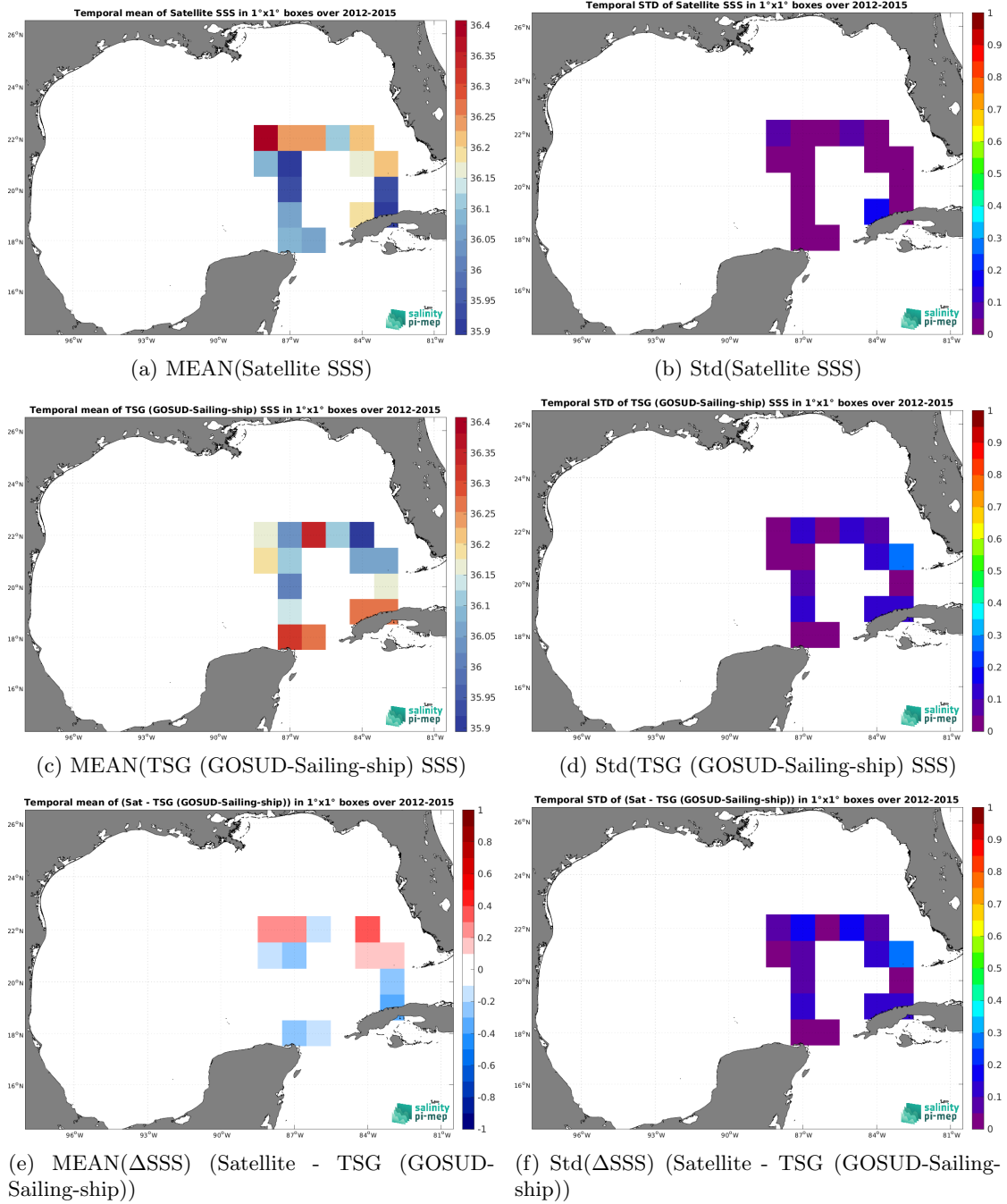
Figure 7: Temporal mean (left) and Std (right) of SSS from SMOS SSS L4 v2 - Daily (BEC) (top), TSG (GOSUD-Sailing-ship) (middle), and of \Delta SSS (Satellite - TSG (GOSUD-Sailing-ship)). Only match-up pairs are used to generate these maps.
