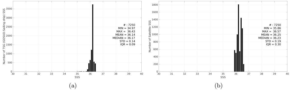
Figure 3: Histograms of SSS from TSG (GOSUD-Sailing-ship) (a) and SMOS SSS L4 v2 - Daily (BEC) (b) considering all match-up pairs per bins of 0.1 over the Gulf of Mexico Pi-MEP region and for the full satellite product period.
