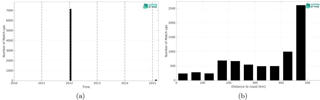
Figure 2: Number of match-ups between TSG (GOSUD-Sailing-ship) and SMOS SSS L4 v2 - Daily (BEC) SSS as a function of time (a) and as function of the distance to coast (b) over the Gulf of Mexico Pi-MEP region and for the full satellite product period.
