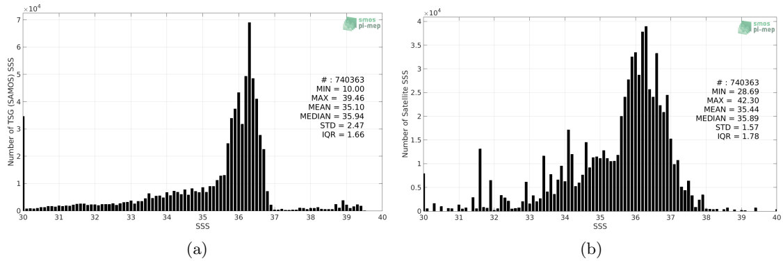
Figure 2: Histograms of SSS from TSG (SAMOS) (a) and SMOS SSS L3 v3 Monthly (ICDC) (b) considering all match-up pairs per bins of 0.1 over the Gulf of Mexico Pi-MEP region and for the full satellite product period.
