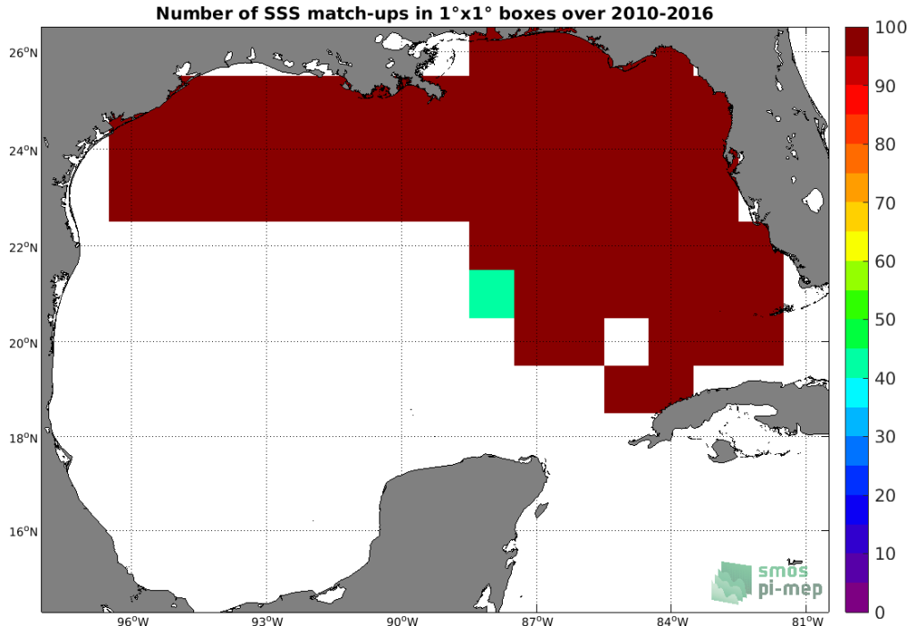
Figure 4: Number of SSS match-ups between TSG (SAMOS) SSS and the SMOS SSS L3 v3 Monthly (ICDC) SSS product for the Gulf of Mexico Pi-MEP region over 1^\circ \times 1^\circ boxes and for the full satellite product period.
