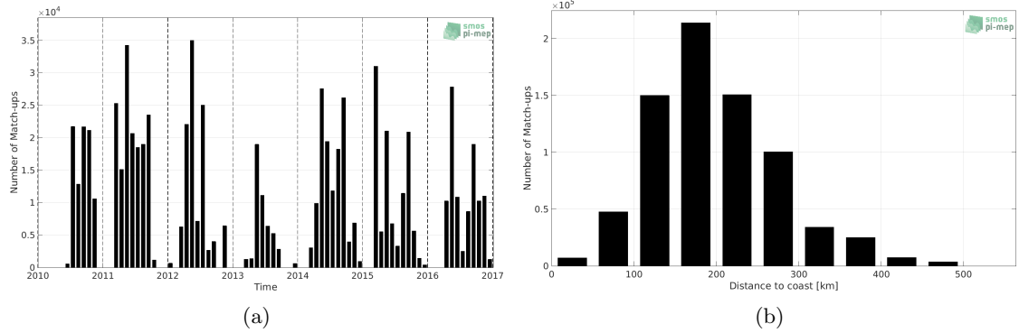
Figure 1: Number of match-ups between TSG (SAMOS) and SMOS SSS L3 v3 Monthly (ICDC) SSS as a function of time (a) and as function of the distance to coast (b) over the Gulf of Mexico Pi-MEP region and for the full satellite product period.
