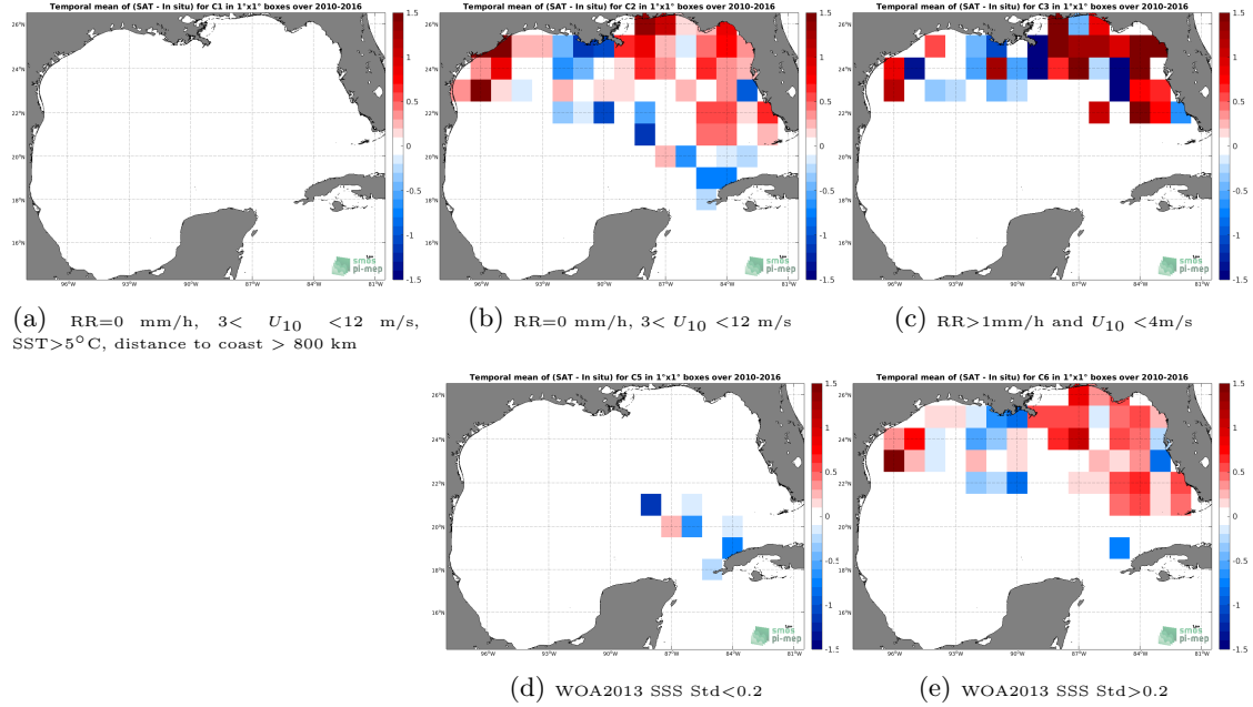
Figure 12: Temporal mean gridded over spatial boxes of size 1^{\circ}\times 1^{\circ} of \Delta\text{SSS} (SMOS SSS L3 v3 Monthly (ICDC) - TSG (SAMOS)) for 5 different subdatasets corresponding to:RR=0 mm/h, 3 < U_{10} < 12 m/s, SST >5^{\circ}\text{C} , distance to coast > 800 km (a), RR=0 mm/h, 3 < U_{10} < 12 m/s (b), RR >1 mm/h and U_{10} < 4 m/s (c), WOA2013 SSS Std <0.2 (d), WOA2013 SSS Std >0.2 (e).
