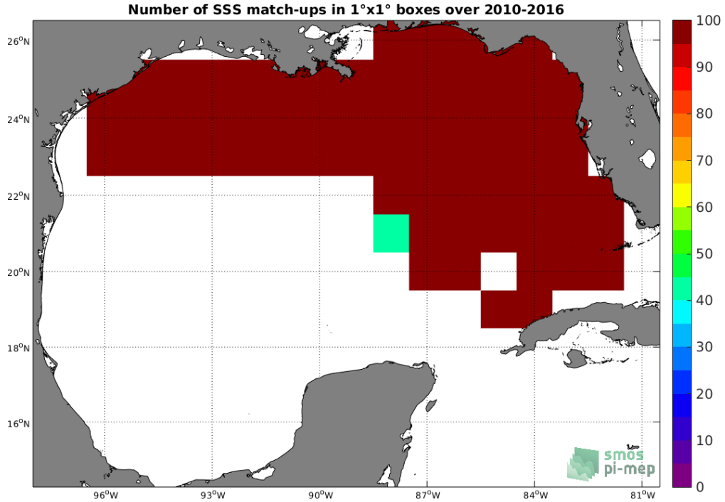
Figure 4: Number of SSS match-ups between TSG-SAMOS SSS and the SMOS-L3-ICDC-V3-MONTHLY-0.5DEG SSS product for the Gulf of Mexico Pi-MEP region over 1^\circ \times 1^\circ boxes and for the full satellite product period.
