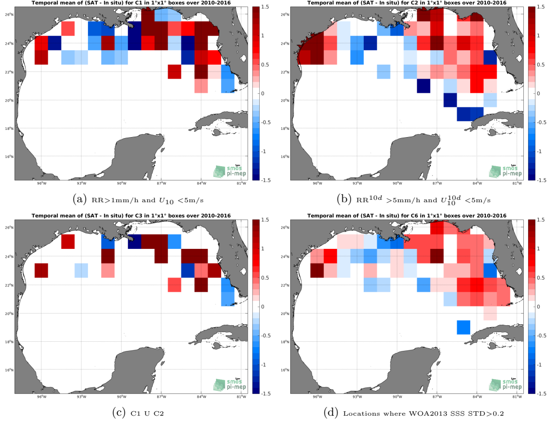
Figure 12: Temporal mean gridded over spatial boxes of size 1^\circ \times 1^\circ of \Delta SSS (SMOS-L3-ICDC-V3-MONTHLY-0.5DEG - TSG-SAMOS) for 4 different subdatasets corresponding to: RR > 1mm/h and U_{10} < 5\text{m/s} (a), RR^{10d} > 5\text{mm/h} and U_{10}^{10d} < 5\text{m/s} (b), C1 U C2 (c), Locations where WOA2013 SSS STD > 0.2 (d).
