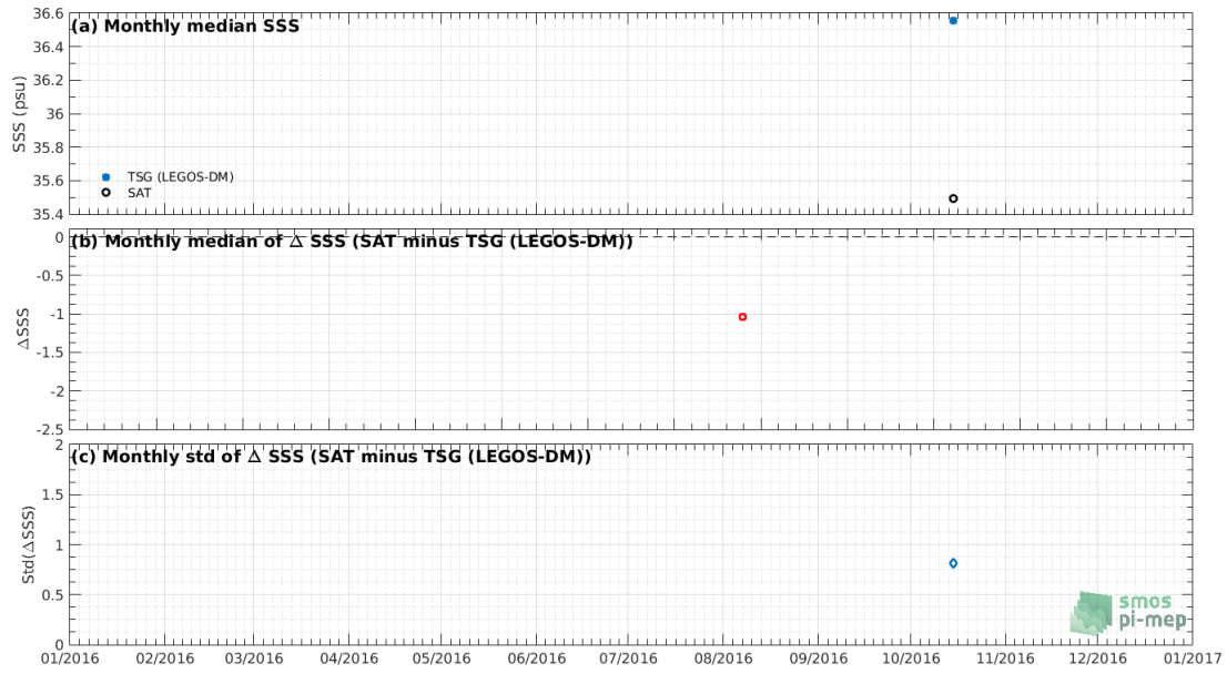
Figure 7: Time series of the monthly median SSS (top), median of \Delta SSS (Satellite - TSG (LEGOS-DM)) and Std of \Delta SSS (Satellite - TSG (LEGOS-DM)) over the Gulf of Mexico Pi-MEP region considering all match-ups collected by the Pi-MEP.
