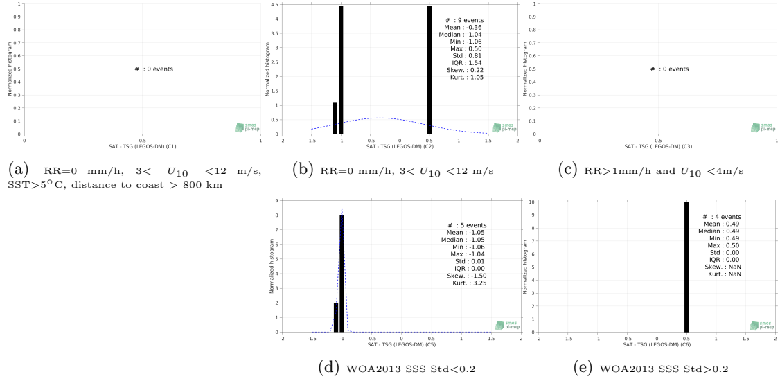
Figure 13: Normalized histogram of \Delta\text{SSS} (SMOS SSS L3 v3 Monthly (ICDC) - TSG (LEGOS-DM)) for 5 different subdatasets corresponding to: RR=0 mm/h, 3 < U_{10} < 12 m/s, SST > 5^\circ\text{C} , distance to coast > 800 km (a), RR=0 mm/h, 3 < U_{10} < 12 m/s (b), RR > 1\text{mm/h} and U_{10} < 4\text{m/s} (c), WOA2013 SSS Std < 0.2 (d), WOA2013 SSS Std > 0.2 (e).
