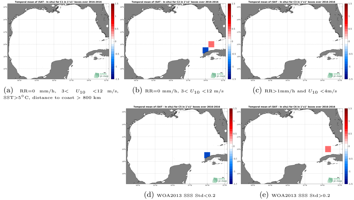
Figure 12: Temporal mean gridded over spatial boxes of size 1^{\circ}\times 1^{\circ} of \Delta\text{SSS} (SMOS SSS L3 v3 Monthly (ICDC) - TSG (LEGOS-DM)) for 5 different subdatasets corresponding to:RR=0 mm/h, 3 < U_{10} < 12 m/s, SST >5^{\circ}\text{C} , distance to coast > 800 km (a), RR=0 mm/h, 3 < U_{10} < 12 m/s (b), RR >1 mm/h and U_{10} < 4 m/s (c), WOA2013 SSS Std <0.2 (d), WOA2013 SSS Std >0.2 (e).
