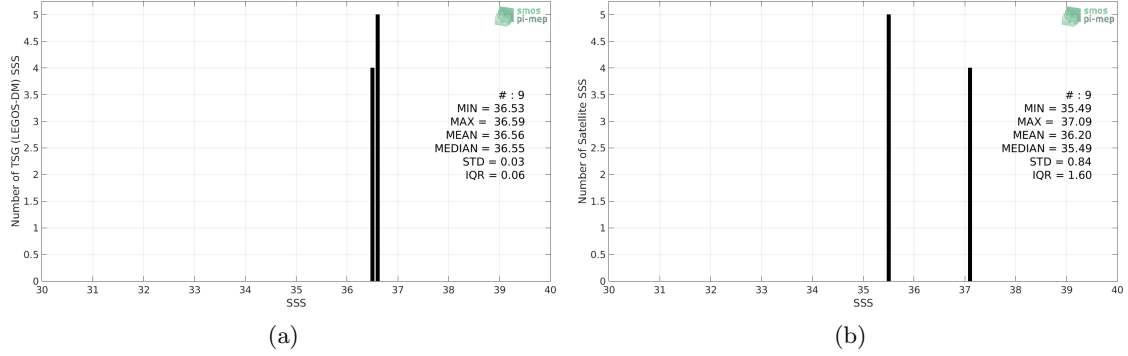
Figure 2: Histograms of SSS from TSG (LEGOS-DM) (a) and SMOS SSS L3 v3 Monthly (ICDC) (b) considering all match-up pairs per bins of 0.1 over the Gulf of Mexico Pi-MEP region and for the full satellite product period.
