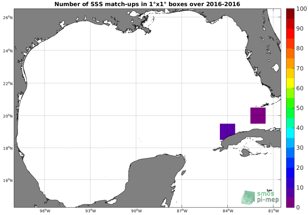
Figure 4: Number of SSS match-ups between TSG (LEGOS-DM) SSS and the SMOS SSS L3 v3 Monthly (ICDC) SSS product for the Gulf of Mexico Pi-MEP region over 1^\circ \times 1^\circ boxes and for the full satellite product period.
