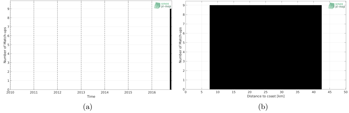
Figure 1: Number of match-ups between TSG (LEGOS-DM) and SMOS SSS L3 v3 Monthly (ICDC) SSS as a function of time (a) and as function of the distance to coast (b) over the Gulf of Mexico Pi-MEP region and for the full satellite product period.
