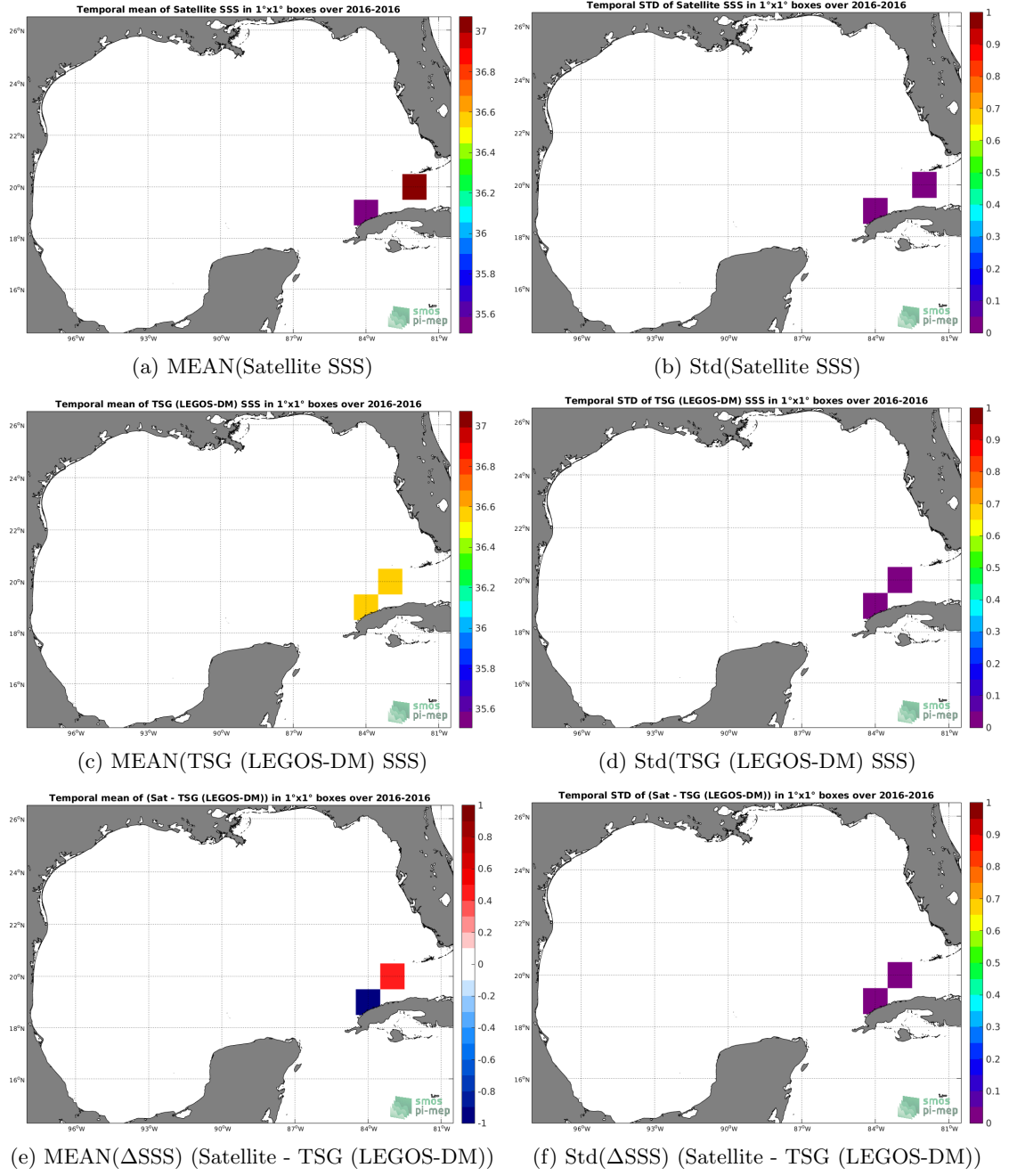
Figure 6: Temporal mean (left) and Std (right) of SSS from SMOS SSS L3 v3 Monthly (ICDC) (top), TSG (LEGOS-DM) (middle), and of \Delta SSS (Satellite - TSG (LEGOS-DM)). Only match-up pairs are used to generate these maps.
