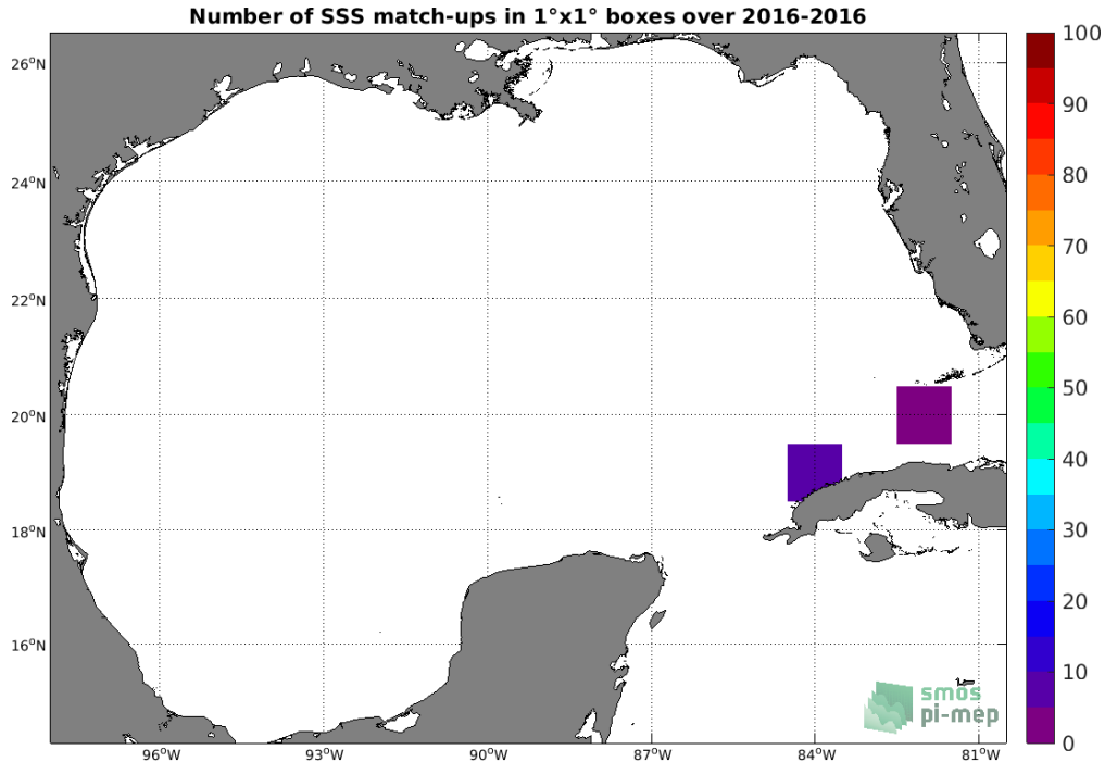
Figure 4: Number of SSS match-ups between TSG (LEGOS-DM) SSS and the SMOS SSS L3 v3 Monthly (ICDC) SSS product for the Gulf of Mexico Pi-MEP region over 1°x1° boxes and for the full satellite product period.
