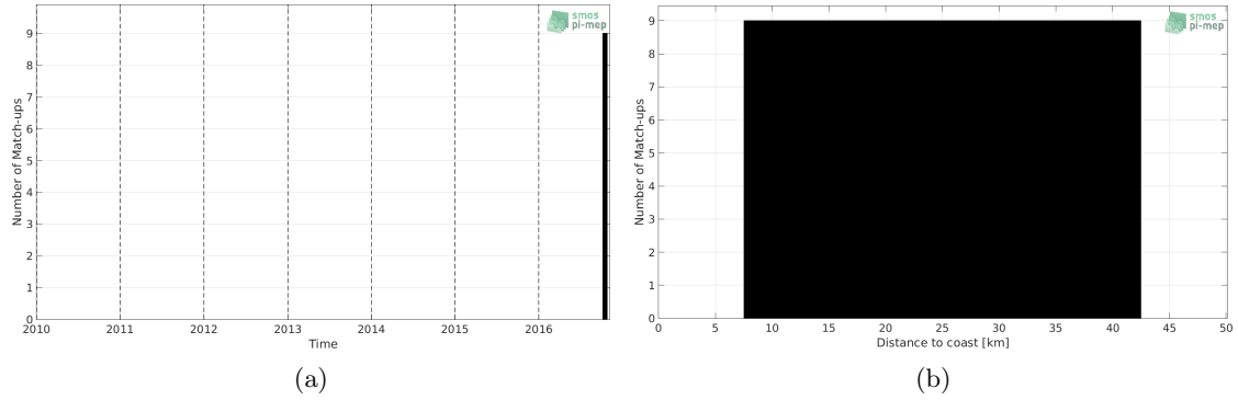
Figure 1: Number of match-ups between TSG-LEGOS-DM and SMOS-L3-ICDC-V3-MONTHLY-0.5DEG SSS as a function of time (a) and as function of the distance to coast (b) over the Gulf of Mexico Pi-MEP region and for the full satellite product period.
