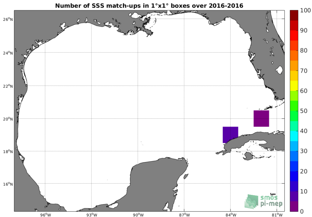
Figure 4: Number of SSS match-ups between TSG-LEGOS-DM SSS and the SMOS-L3-ICDC-V3-MONTHLY-0.5DEG SSS product for the Gulf of Mexico Pi-MEP region over 1°x1° boxes and for the full satellite product period.
