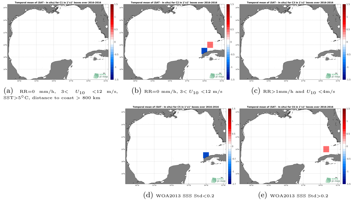
Figure 12: Temporal mean gridded over spatial boxes of size 1^{\circ}\times 1^{\circ} of \Delta\text{SSS} (SMOS-L3-ICDC-V3-MONTHLY-0.5DEG - TSG-LEGOS-DM) for 5 different subdatasets corresponding to: \text{RR}=0 mm/h, 3 < U_{10} < 12 m/s, \text{SST} > 5^{\circ}\text{C} , distance to coast > 800 km (a), \text{RR}=0 mm/h, 3 < U_{10} < 12 m/s (b), \text{RR} > 1 mm/h and U_{10} < 4 m/s (c), WOA2013 SSS Std < 0.2 (d), WOA2013 SSS Std > 0.2 (e).
