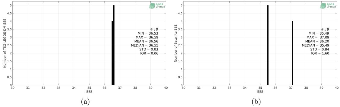
Figure 2: Histograms of SSS from TSG-LEGOS-DM (a) and SMOS-L3-ICDC-V3-MONTHLY-0.5DEG (b) considering all match-up pairs per bins of 0.1 over the Gulf of Mexico Pi-MEP region and for the full satellite product period.
