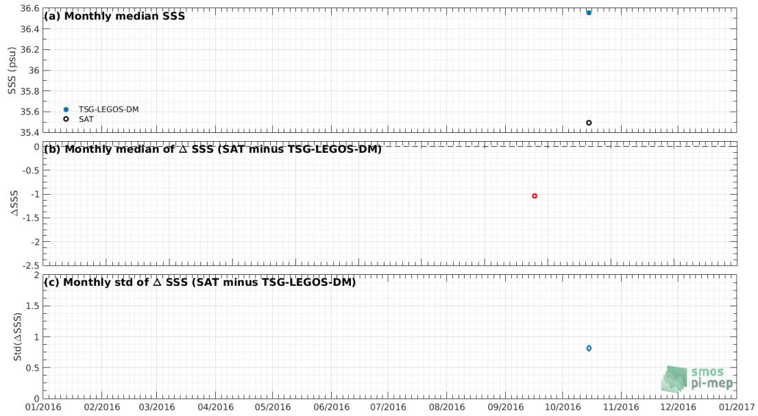
Figure 7: Time series of the monthly median SSS (top), median of \Delta SSS (Satellite - TSG-LEGOS-DM) and Std of \Delta SSS (Satellite - TSG-LEGOS-DM) over the Gulf of Mexico Pi-MEP region considering all match-ups collected by the Pi-MEP.
