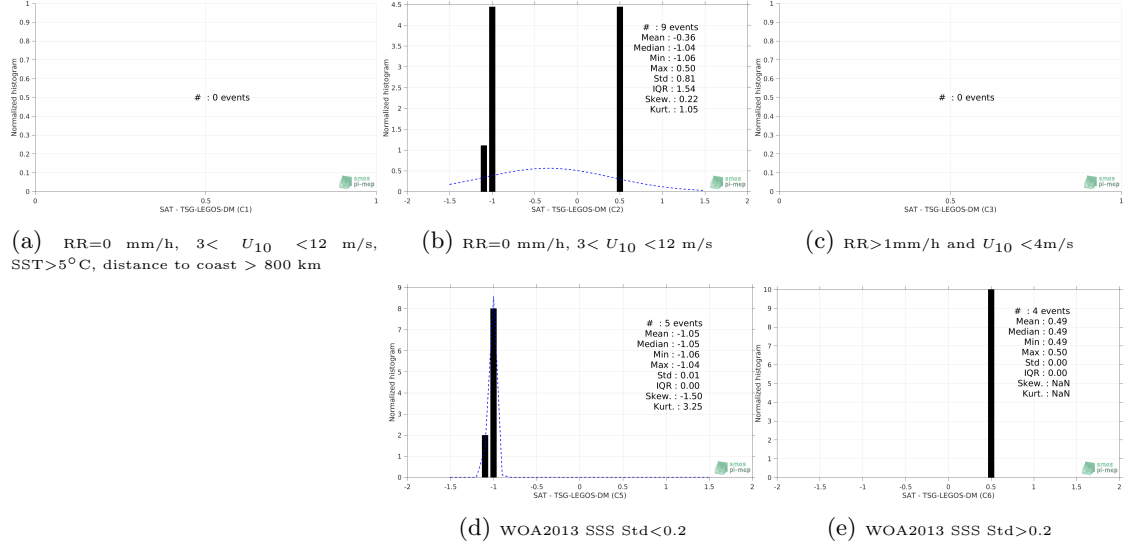
Figure 13: Normalized histogram of \Delta SSS (SMOS-L3-ICDC-V3-MONTHLY-0.5DEG - TSG-LEGOS-DM) for 5 different subdatasets corresponding to: RR=0 mm/h, 3 < U_{10} < 12 m/s, SST>5°C, distance to coast > 800 km (a), RR=0 mm/h, 3 < U_{10} < 12 m/s (b), RR>1mm/h and U_{10} < 4 m/s (c), WOA2013 SSS Std<0.2 (d), WOA2013 SSS Std>0.2 (e).
