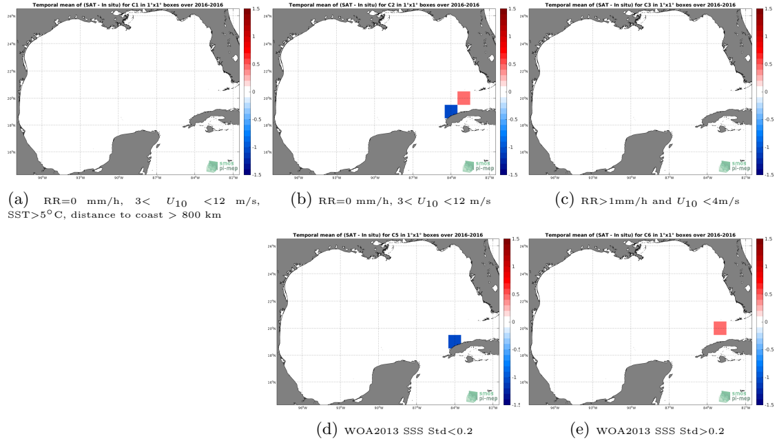
Figure 12: Temporal mean gridded over spatial boxes of size 1^\circ \times 1^\circ of \Delta SSS (SMOS-L3-ICDC-V3-MONTHLY-0.5DEG - TSG-LEGOS-DM) for 5 different subdatasets corresponding to:RR=0 mm/h, 3 < U_{10} < 12 m/s, SST >5^\circ\text{C} , distance to coast > 800 km (a), RR=0 mm/h, 3 < U_{10} < 12 m/s (b), RR >1 mm/h and U_{10} < 4 m/s (c), WOA2013 SSS Std <0.2 (d), WOA2013 SSS Std >0.2 (e).
