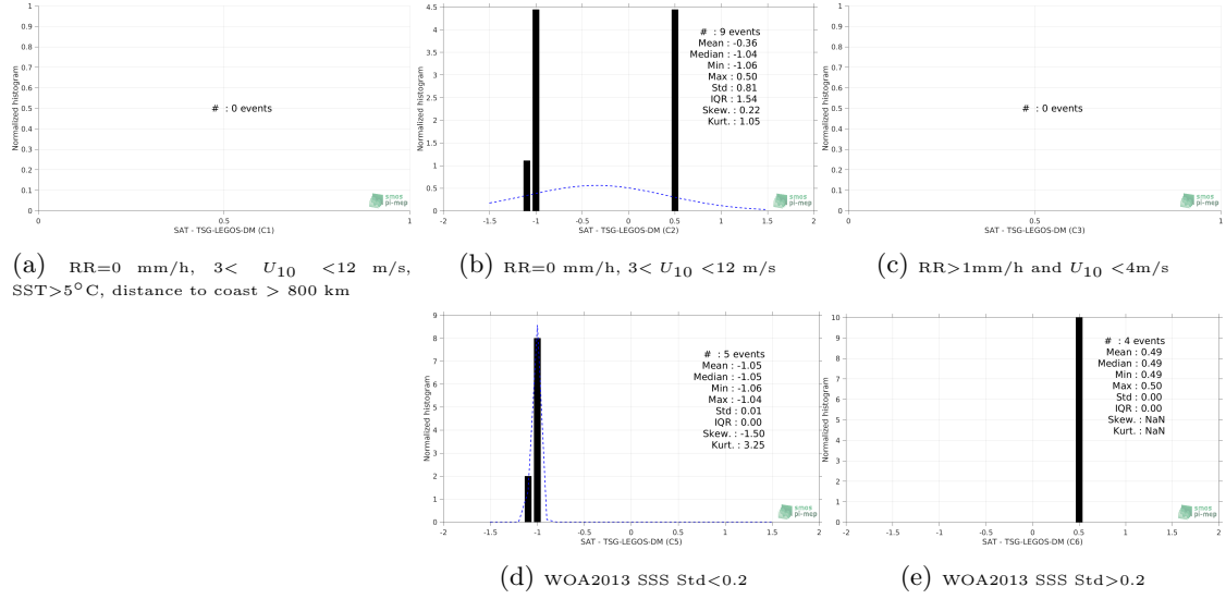
Figure 13: Normalized histogram of \Delta\text{SSS} (SMOS-L3-ICDC-V3-MONTHLY-0.5DEG - TSG-LEGOS-DM) for 5 different subdatasets corresponding to: RR=0 mm/h, 3 < U_{10} < 12 m/s, SST > 5^{\circ}\text{C} , distance to coast > 800 km (a), RR=0 mm/h, 3 < U_{10} < 12 m/s (b), RR > 1\text{mm/h} and U_{10} < 4\text{m/s} (c), WOA2013 SSS Std < 0.2 (d), WOA2013 SSS Std > 0.2 (e).
