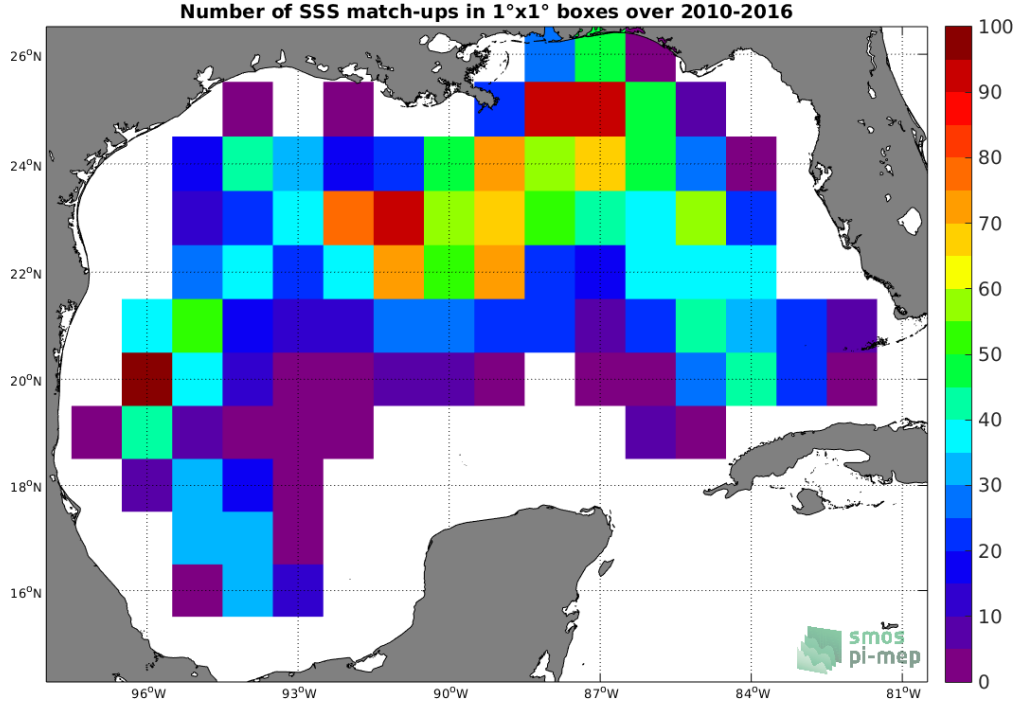
Figure 4: Number of SSS match-ups between Argo SSS and the SMOS SSS L3 v3 Monthly (ICDC) SSS product for the Gulf of Mexico Pi-MEP region over 1^\circ \times 1^\circ boxes and for the full satellite product period.
