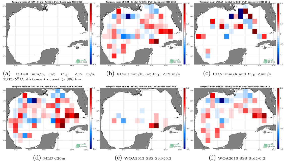
Figure 12: Temporal mean gridded over spatial boxes of size 1^\circ \times 1^\circ of \Delta SSS (SMOS SSS L3 v3 Monthly (ICDC) - Argo) for 6 different subdatasets corresponding to: RR=0 mm/h, 3 < U_{10} < 12 m/s, SST >5^\circ\text{C} , distance to coast > 800 km (a), RR=0 mm/h, 3 < U_{10} < 12 m/s (b), RR >1 mm/h and U_{10} < 4 m/s (c), MLD <20 m (d), WOA2013 SSS Std <0.2 (e), WOA2013 SSS Std >0.2 (f).
