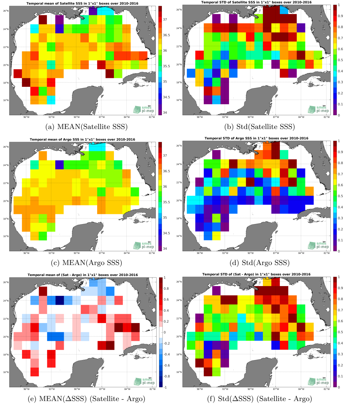
Figure 6: Temporal mean (left) and Std (right) of SSS from SMOS SSS L3 v3 Monthly (ICDC') (top), Argo (middle), and of \Delta SSS (Satellite - Argo). Only match-up pairs are used to generate these maps.
