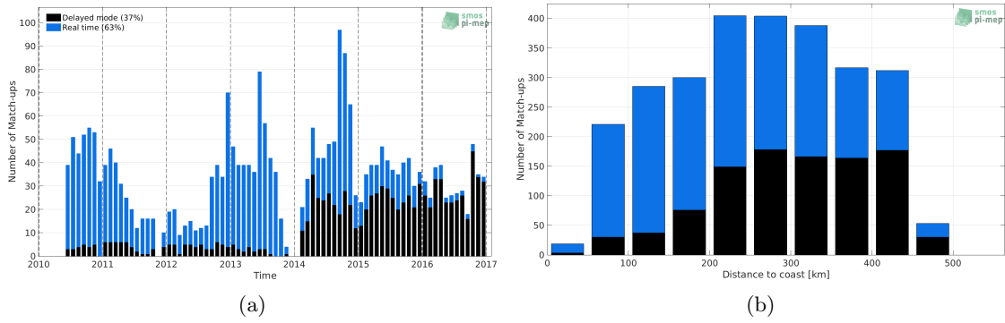
Figure 1: Number of match-ups between Argo and SMOS SSS L3 v3 Monthly (ICDC) SSS as a function of time (a) and as function of the distance to coast (b) over the Gulf of Mexico Pi-MEP region and for the full satellite product period.
