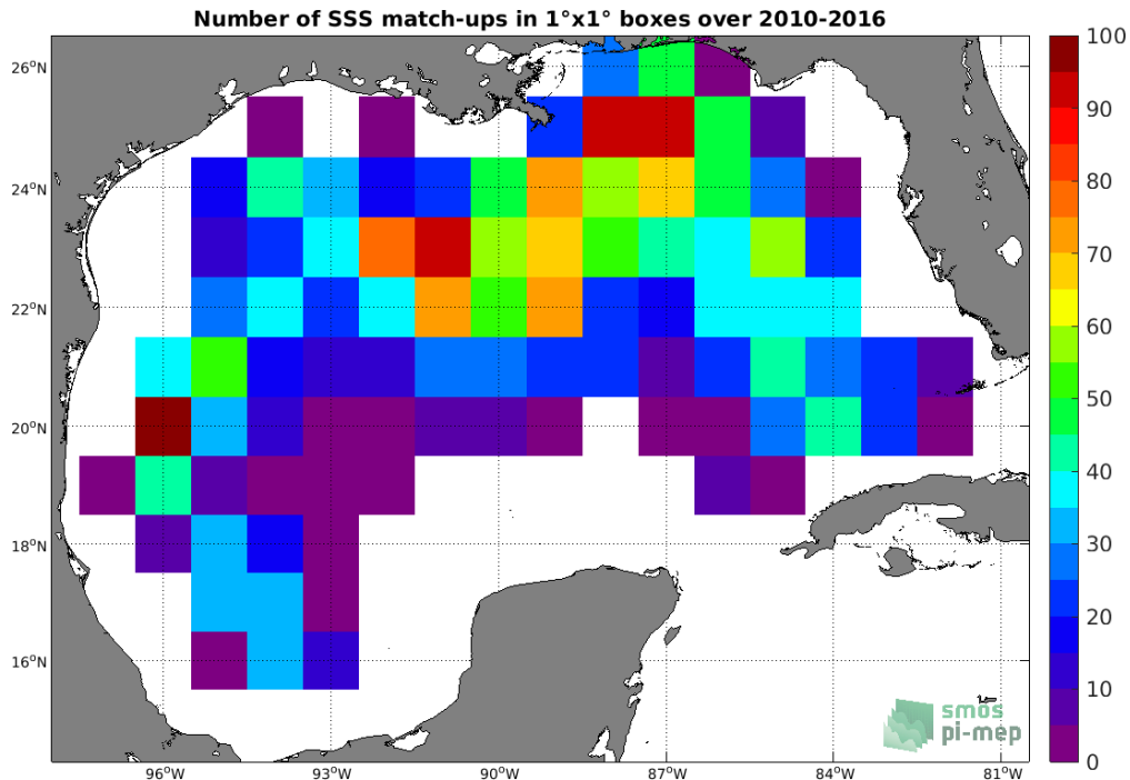
Figure 4: Number of SSS match-ups between Argo SSS and the SMOS SSS L3 v3 Monthly (ICDC) SSS product for the Gulf of Mexico Pi-MEP region over 1°x1° boxes and for the full satellite product period.
