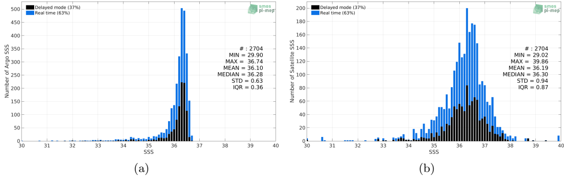
Figure 2: Histograms of SSS from Argo (a) and SMOS SSS L3 v3 Monthly (ICDC) (b) considering all match-up pairs per bins of 0.1 over the Gulf of Mexico Pi-MEP region and for the full satellite product period.
