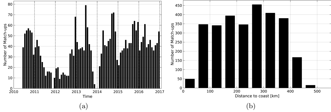
Figure 1: Number of match-ups between Argo and SMOS-L3-ICDC-V3-MONTHLY-0.5DEG SSS as a function of time (a) and as function of the distance to coast (b) over the Gulf of Mexico Pi-MEP region and for the full satellite product period.
