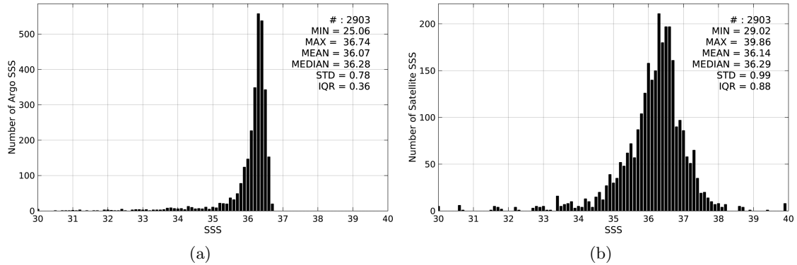
Figure 2: Histograms of SSS from Argo (a) and SMOS-L3-ICDC-V3-MONTHLY-0.5DEG (b) considering all match-up pairs per bins of 0.1 over the Gulf of Mexico Pi-MEP region and for the full satellite product period.
