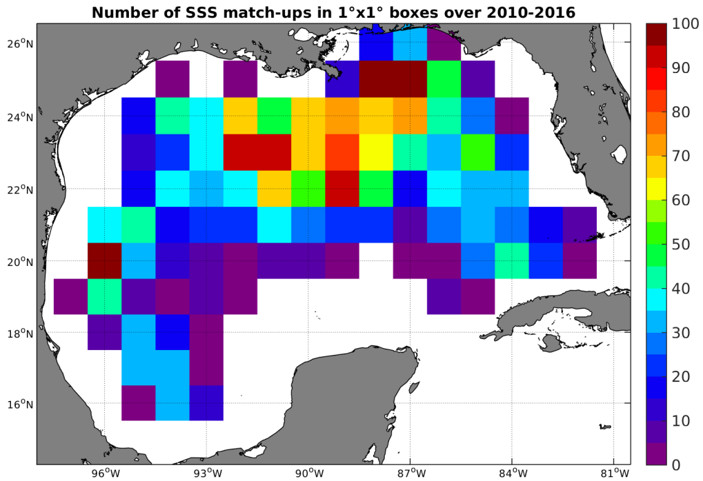
Figure 4: Number of SSS match-ups between Argo SSS and the SMOS-L3-ICDC-V3-MONTHLY-0.5DEG SSS product for the Gulf of Mexico Pi-MEP region over 1^\circ \times 1^\circ boxes and for the full satellite product period.
