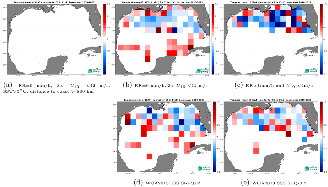
Figure 12: Temporal mean gridded over spatial boxes of size 1^{\circ}\times 1^{\circ} of \Delta\text{SSS} (SMOS SSS L2Q v331 - With FLAG (CMEMS-CATDS-CPDC) - TSG (SAMOS)) for 5 different subdatasets corresponding to:RR=0 mm/h, 3 < U_{10} < 12 m/s, SST >5^{\circ}\text{C} , distance to coast > 800 km (a), RR=0 mm/h, 3 < U_{10} < 12 m/s (b), RR >1 mm/h and U_{10} < 4 m/s (c), WOA2013 SSS Std <0.2 (d), WOA2013 SSS Std >0.2 (e).
