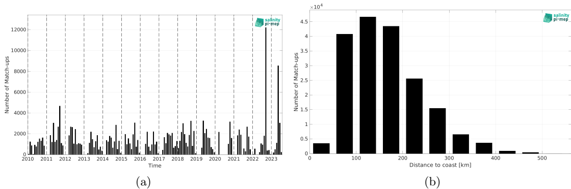
Figure 1: Number of match-ups between TSG (SAMOS) and SMOS SSS L2Q v331 - With FLAG (CMEMS-CATDS-CPDC) SSS as a function of time (a) and as function of the distance to coast (b) over the Gulf of Mexico Pi-MEP region and for the full satellite product period.
