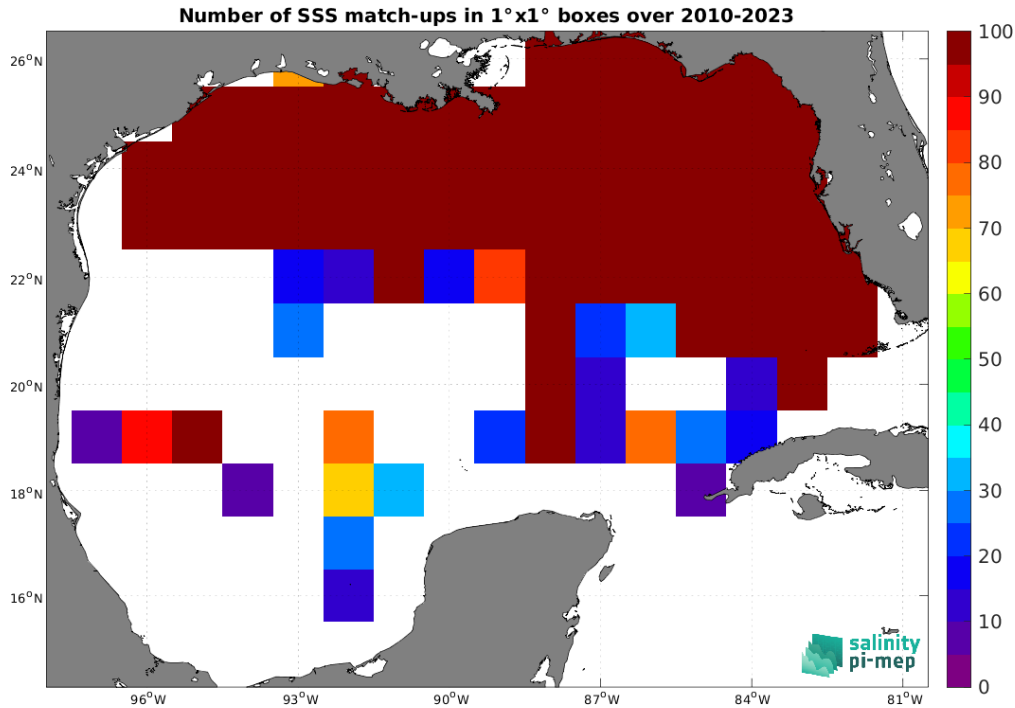
Figure 4: Number of SSS match-ups between TSG (SAMOS) SSS and the SMOS SSS L2Q v331 - With FLAG (CMEMS-CATDS-CPDC) SSS product for the Gulf of Mexico Pi-MEP region over 1^\circ \times 1^\circ boxes and for the full satellite product period.
