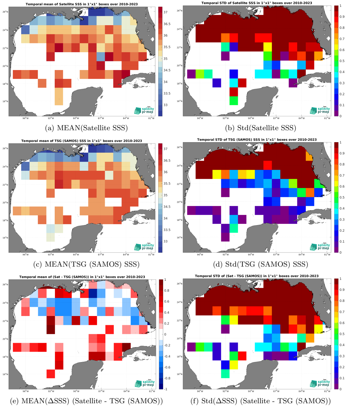
Figure 6: Temporal mean (left) and Std (right) of SSS from SMOS SSS L2Q v331 - With FLAG (CMEMS-CATDS-CPDC) (top), TSG (SAMOS) (middle), and of \Delta SSS (Satellite - TSG (SAMOS)). Only match-up pairs are used to generate these maps.
