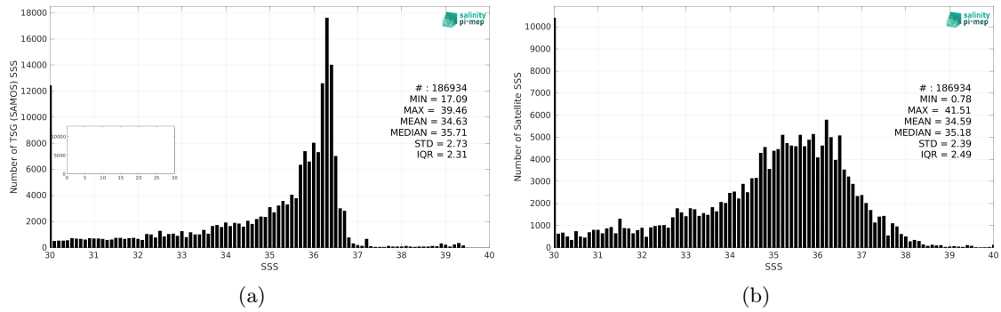
Figure 2: Histograms of SSS from TSG (SAMOS) (a) and SMOS SSS L2Q v331 - With FLAG (CMEMS-CATDS-CPDC) (b) considering all match-up pairs per bins of 0.1 over the Gulf of Mexico Pi-MEP region and for the full satellite product period.
