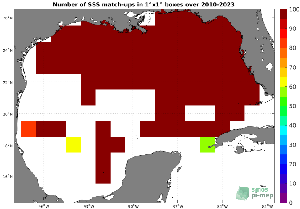
Figure 4: Number of SSS match-ups between TSG (SAMOS) SSS and the SMOS SSS L2Q v331 - With FLAG (CMEMS-CATDS-CPDC) SSS product for the Gulf of Mexico Pi-MEP region over 1°×1° boxes and for the full satellite product period.
