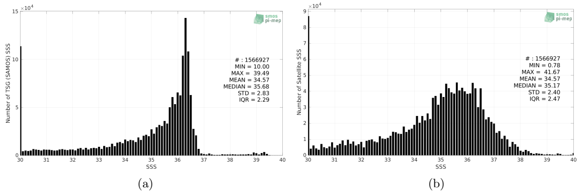
Figure 2: Histograms of SSS from TSG (SAMOS) (a) and SMOS SSS L2Q v331 - With FLAG (CMEMS-CATDS-CPDC) (b) considering all match-up pairs per bins of 0.1 over the Gulf of Mexico Pi-MEP region and for the full satellite product period.
