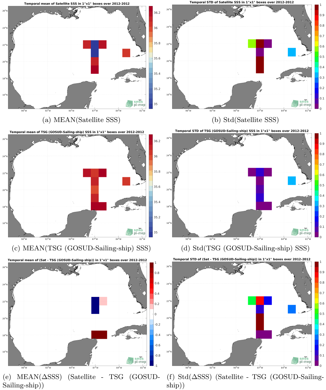
Figure 6: Temporal mean (left) and Std (right) of SSS from SMOS SSS L2Q v331 - With FLAG (CMEMS-CATDS-CPDC) (top), TSG (GOSUD-Sailing-ship) (middle), and of \Delta SSS (Satellite - TSG (GOSUD-Sailing-ship)). Only match-up pairs are used to generate these maps.
