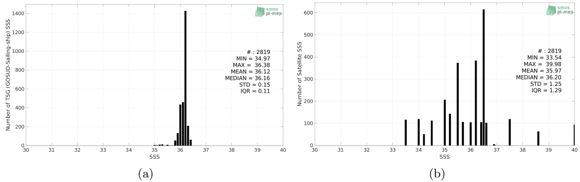
Figure 2: Histograms of SSS from TSG (GOSUD-Sailing-ship) (a) and SMOS SSS L2Q v331 - With FLAG (CMEMS-CATDS-CPDC) (b) considering all match-up pairs per bins of 0.1 over the Gulf of Mexico Pi-MEP region and for the full satellite product period.
