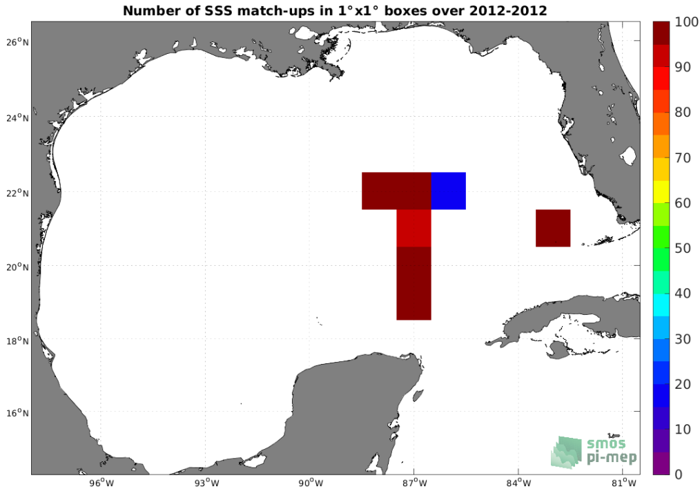
Figure 4: Number of SSS match-ups between TSG (GOSUD-Sailing-ship) SSS and the SMOS SSS L2Q v331 - With FLAG (CMEMS-CATDS-CPDC) SSS product for the Gulf of Mexico Pi-MEP region over 1^\circ \times 1^\circ boxes and for the full satellite product period.
