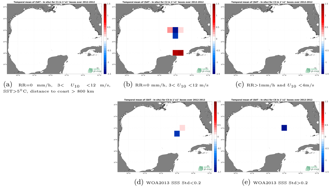
Figure 12: Temporal mean gridded over spatial boxes of size 1^\circ \times 1^\circ of \Delta SSS (SMOS SSS L2Q v331 - With FLAG (CMEMS-CATDS-CPDC) - TSG (GOSUD-Sailing-ship)) for 5 different subdatasets corresponding to:RR=0 mm/h, 3 < U_{10} < 12 m/s, SST >5^\circ\text{C} , distance to coast > 800 km (a), RR=0 mm/h, 3 < U_{10} < 12 m/s (b), RR >1 mm/h and U_{10} < 4 m/s (c), WOA2013 SSS Std <0.2 (d), WOA2013 SSS Std >0.2 (e).
