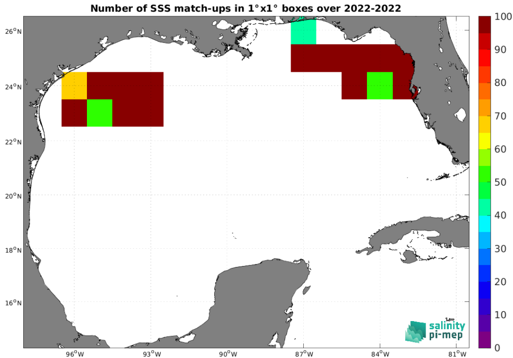
Figure 5: Number of SSS match-ups between Saildrone SSS and the SMOS SSS L2Q v331 - With FLAG (CMEMS-CATDS-CPDC) SSS product for the Gulf of Mexico Pi-MEP region over 1^\circ \times 1^\circ boxes and for the full satellite product period.
