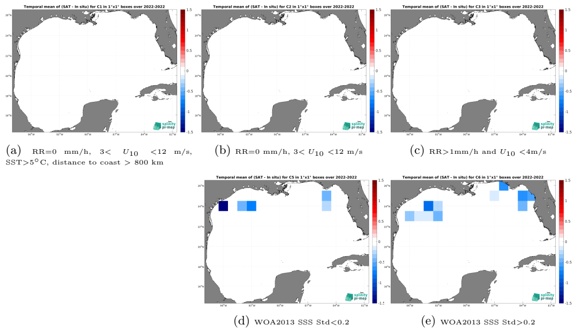
Figure 14: Temporal mean gridded over spatial boxes of size 1^\circ \times 1^\circ of \Delta\text{SSS} (SMOS SSS L2Q v331 - With FLAG (CMEMS-CATDS-CPDC) - Saildrone) for 5 different subdatasets corresponding to:RR=0 mm/h, 3 < U_{10} < 12 m/s, SST >5^\circ\text{C} , distance to coast > 800 km (a), RR=0 mm/h, 3 < U_{10} < 12 m/s (b), RR >1 mm/h and U_{10} < 4 m/s (c), WOA2013 SSS Std <0.2 (d), WOA2013 SSS Std >0.2 (e).
