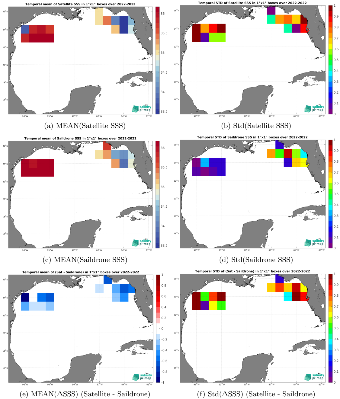
Figure 7: Temporal mean (left) and Std (right) of SSS from SMOS SSS L2Q v331 - With FLAG (CMEMS-CATDS-CPDC) (top), Saildrone (middle), and of \Delta SSS (Satellite - Saildrone). Only match-up pairs are used to generate these maps.
