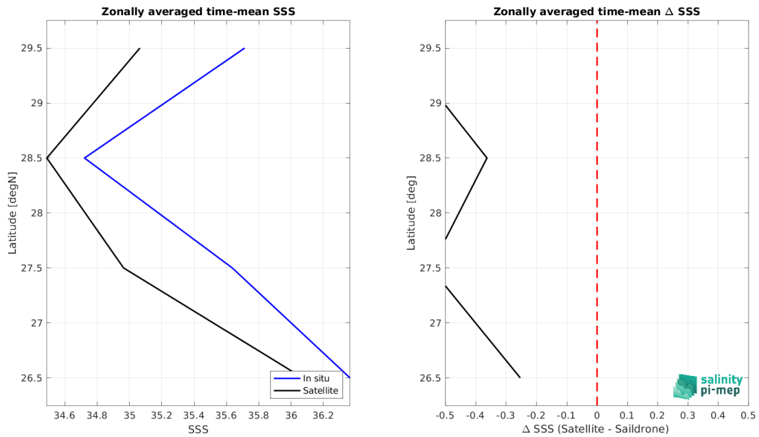
Figure 9: Left panel: Zonal mean SSS from SMOS SSS L2Q v331 - With FLAG (CMEMS-CATDS-CPDC) satellite product (black) and from Sairdrone (blue). Right panel: Zonal mean of \Delta SSS (Satellite - Sairdrone) for all the collected Pi-MEP match-up pairs estimated over the full satellite product period.
