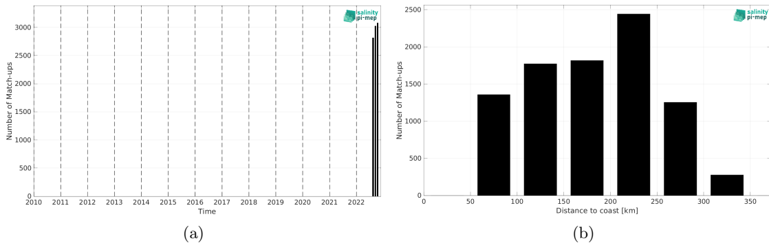
Figure 2: Number of match-ups between Saildrone and SMOS SSS L2Q v331 - With FLAG (CMEMS-CATDS-CPDC) SSS as a function of time (a) and as function of the distance to coast (b) over the Gulf of Mexico Pi-MEP region and for the full satellite product period.
