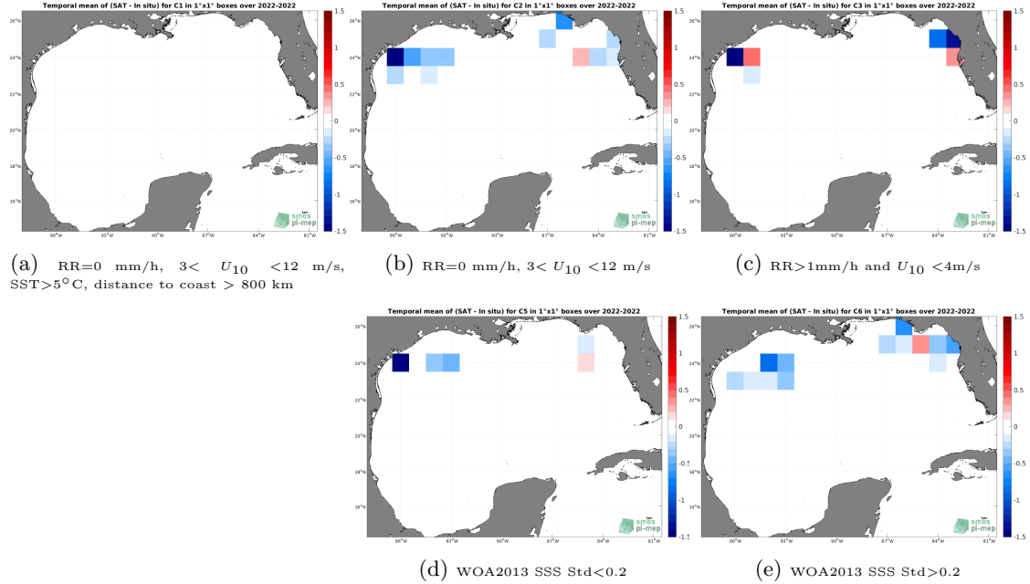
Figure 12: Temporal mean gridded over spatial boxes of size 1^{\circ}\times 1^{\circ} of \Delta\text{SSS} (SMOS SSS L2Q v331 - With FLAG (CMEMS-CATDS-CPDC) - Saildrone) for 5 different subdatasets corresponding to:RR=0 mm/h, 3 < U_{10} < 12 m/s, SST >5^{\circ}\text{C} , distance to coast > 800 km (a), RR=0 mm/h, 3 < U_{10} < 12 m/s (b), RR >1 mm/h and U_{10} < 4 m/s (c), WOA2013 SSS Std <0.2 (d), WOA2013 SSS Std >0.2 (e).
