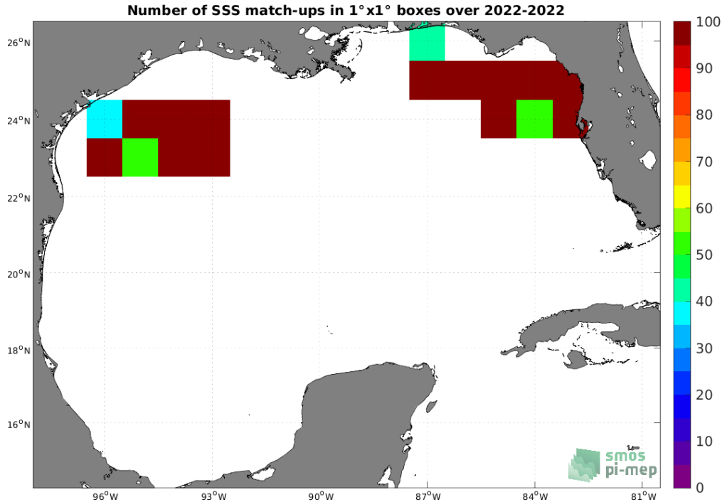
Figure 4: Number of SSS match-ups between Saildrone SSS and the SMOS SSS L2Q v331 - With FLAG (CMEMS-CATDS-CPDC) SSS product for the Gulf of Mexico Pi-MEP region over 1^\circ \times 1^\circ boxes and for the full satellite product period.
