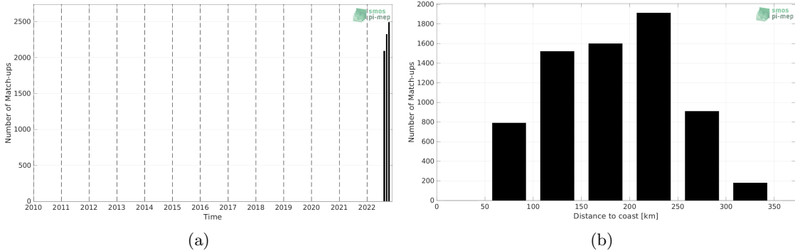
Figure 1: Number of match-ups between Saildrone and SMOS SSS L2Q v331 - With FLAG (CMEMS-CATDS-CPDC) SSS as a function of time (a) and as function of the distance to coast (b) over the Gulf of Mexico Pi-MEP region and for the full satellite product period.
