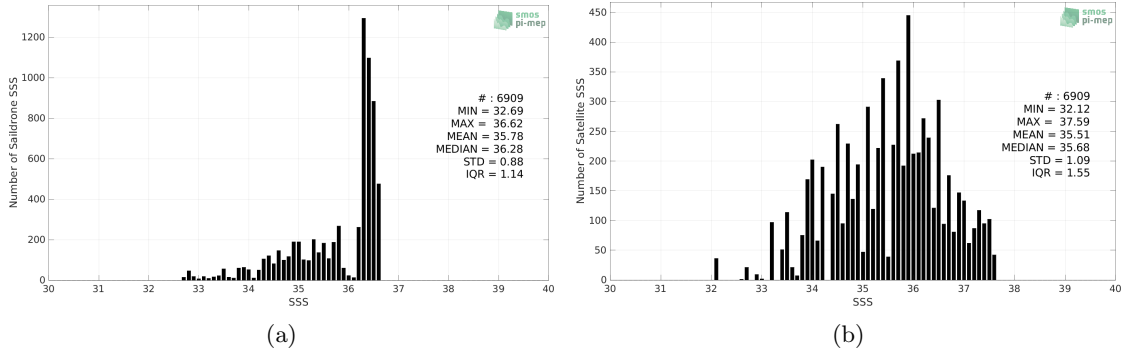
Figure 2: Histograms of SSS from Sairdrone (a) and SMOS SSS L2Q v331 - With FLAG (CMEMS-CATDS-CPDC) (b) considering all match-up pairs per bins of 0.1 over the Gulf of Mexico Pi-MEP region and for the full satellite product period.
