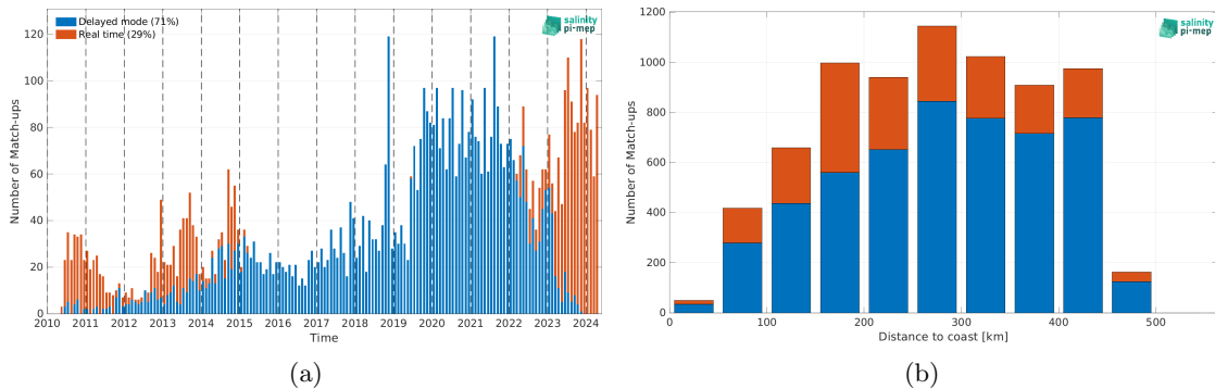
Figure 2: Number of match-ups between Argo and SMOS SSS L2Q v331 - With FLAG (CMEMS-CATDS-CPDC) SSS as a function of time (a) and as function of the distance to coast (b) over the Gulf of Mexico Pi-MEP region and for the full satellite product period.
