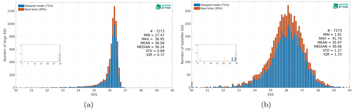
Figure 3: Histograms of SSS from Argo (a) and SMOS SSS L2Q v331 - With FLAG (CMEMS-CATDS-CPDC) (b) considering all match-up pairs per bins of 0.1 over the Gulf of Mexico Pi-MEP region and for the full satellite product period.
