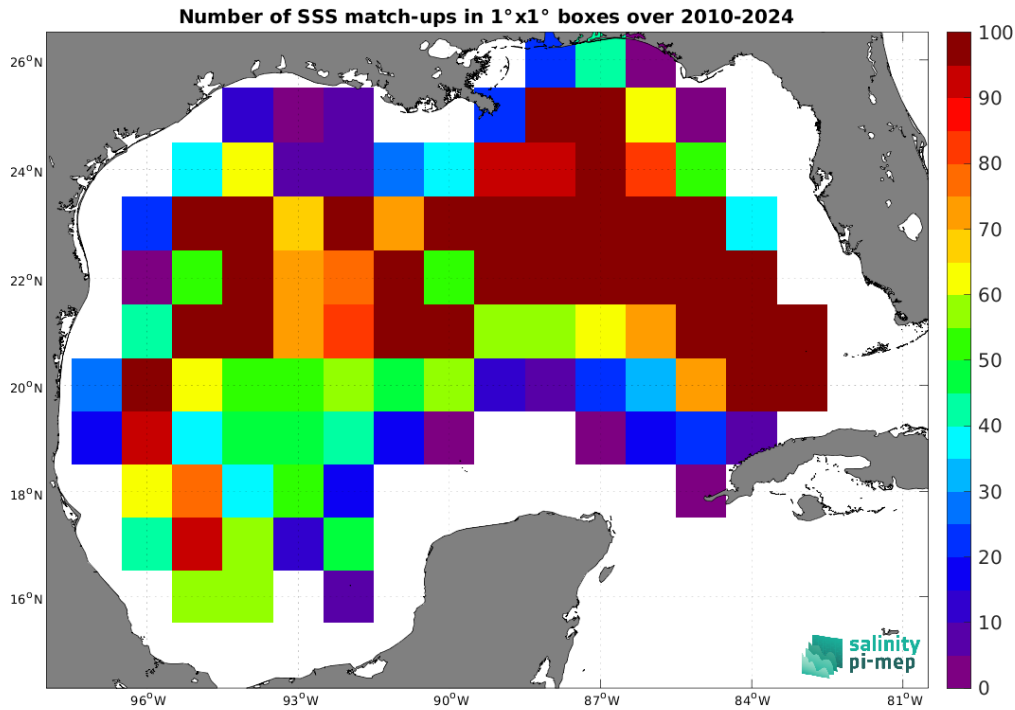
Figure 5: Number of SSS match-ups between Argo SSS and the SMOS SSS L2Q v331 - With FLAG (CMEMS-CATDS-CPDC) SSS product for the Gulf of Mexico Pi-MEP region over 1^\circ \times 1^\circ boxes and for the full satellite product period.
