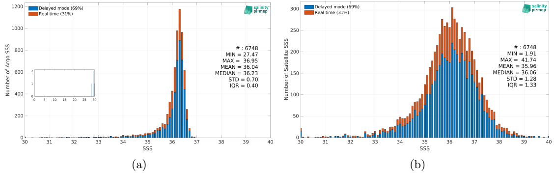
Figure 2: Histograms of SSS from Argo (a) and SMOS SSS L2Q v331 - With FLAG (CMEMS-CATDS-CPDC) (b) considering all match-up pairs per bins of 0.1 over the Gulf of Mexico Pi-MEP region and for the full satellite product period.
