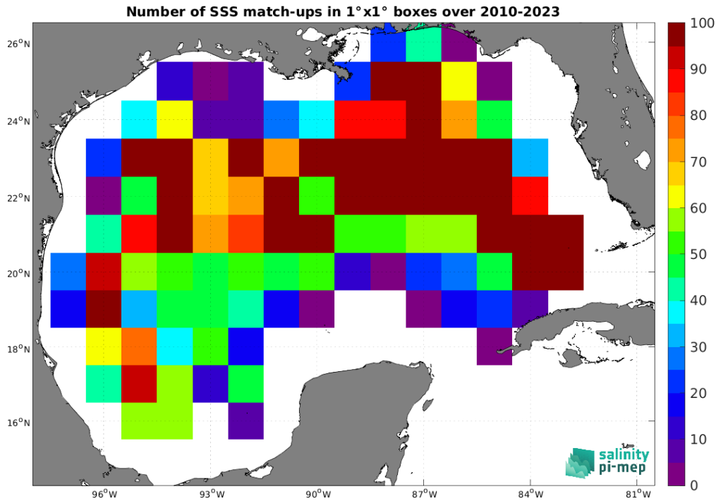
Figure 4: Number of SSS match-ups between Argo SSS and the SMOS SSS L2Q v331 - With FLAG (CMEMS-CATDS-CPDC) SSS product for the Gulf of Mexico Pi-MEP region over 1^\circ \times 1^\circ boxes and for the full satellite product period.
