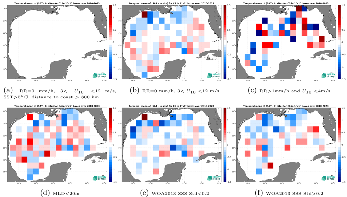
Figure 12: Temporal mean gridded over spatial boxes of size 1^\circ \times 1^\circ of \Delta SSS (SMOS SSS L2Q v331 - With FLAG (CMEMS-CATDS-CPDC) - Argo) for 6 different subdatasets corresponding to:RR=0 mm/h, 3 < U_{10} < 12 m/s, SST > 5^\circ\text{C} , distance to coast > 800 km (a), RR=0 mm/h, 3 < U_{10} < 12 m/s (b), RR > 1 mm/h and U_{10} < 4 m/s (c),MLD < 20 m (d),WOA2013 SSS Std < 0.2 (e),WOA2013 SSS Std > 0.2 (f).
