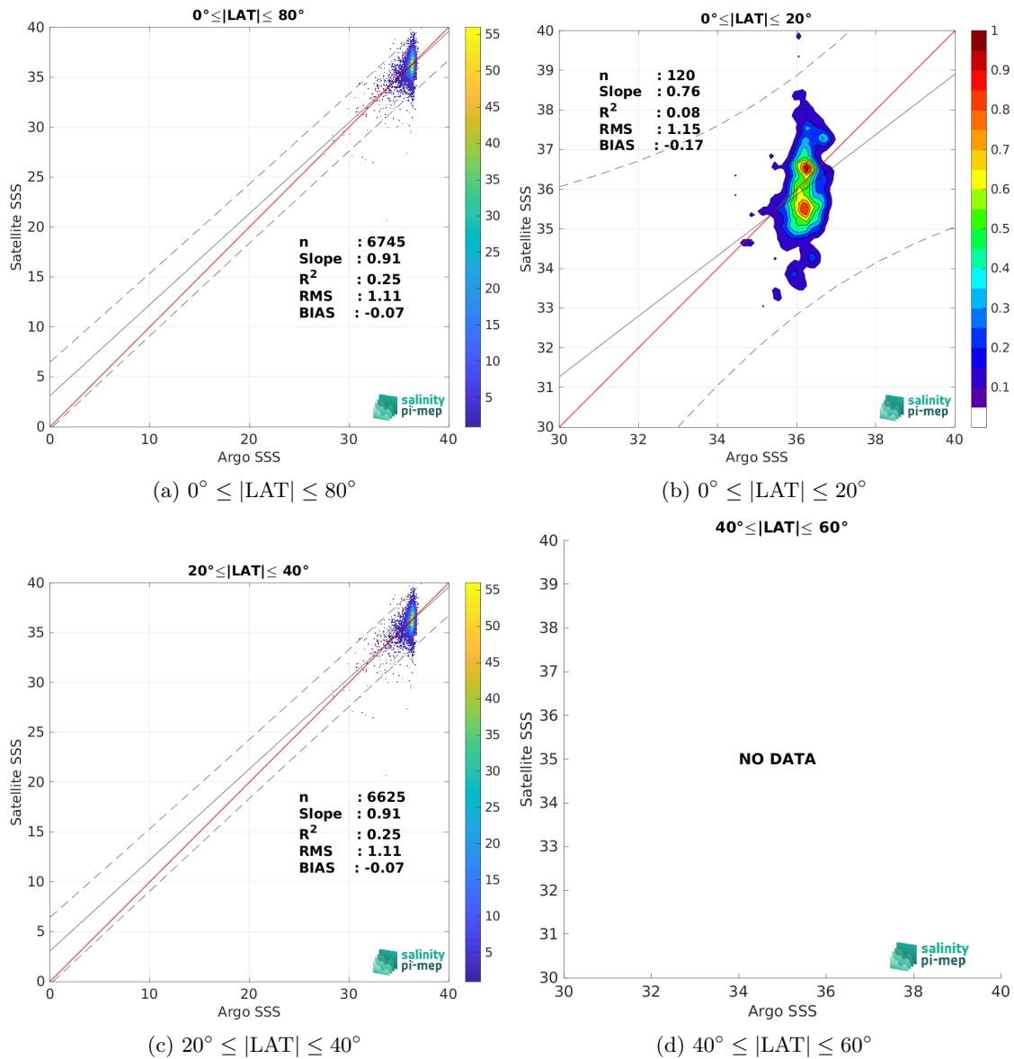
Figure 9: Contour maps of the concentration of SMOS SSS L2Q v331 - With FLAG (CMEMS-CATDS-CPDC) SSS ( y -axis) versus Argo SSS ( x -axis) at match-up pairs for different latitude bands. For each plot, the red line shows x=y . The black thin and dashed lines indicate a linear fit through the data cloud and the \pm 95\% confidence levels, respectively. The number match-up pairs n , the slope and R^2 coefficient of the linear fit, the root mean square (RMS) and the mean bias between satellite and in situ data are indicated for each latitude band in each plots.
