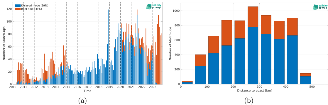
Figure 1: Number of match-ups between Argo and SMOS SSS L2Q v331 - With FLAG (CMEMS-CATDS-CPDC) SSS as a function of time (a) and as function of the distance to coast (b) over the Gulf of Mexico Pi-MEP region and for the full satellite product period.
