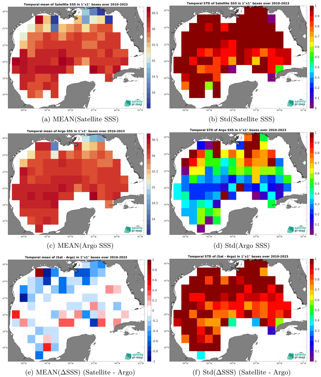
Figure 6: Temporal mean (left) and Std (right) of SSS from SMOS SSS L2Q v331 - With FLAG (CMEMS-CATDS-CPDC) (top), Argo (middle), and of \Delta SSS (Satellite - Argo). Only match-up pairs are used to generate these maps.
