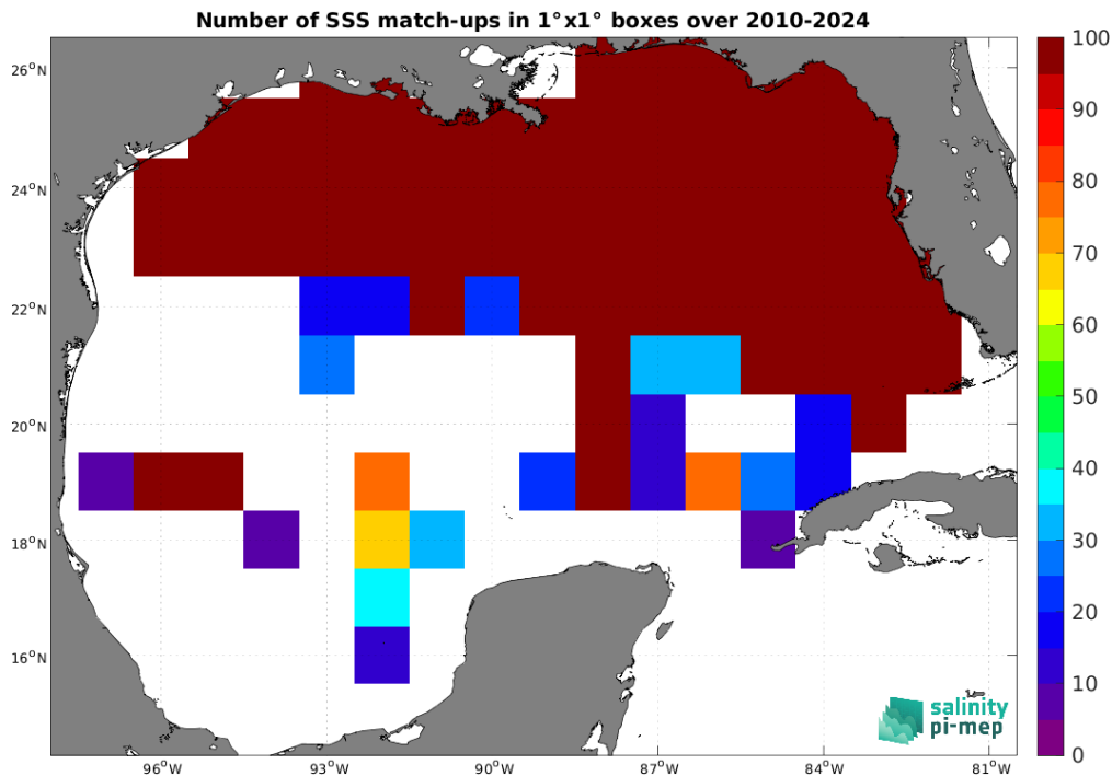
Figure 5: Number of SSS match-ups between TSG (SAMOS) SSS and the SMOS SSS L2Q v331 - No FLAG (CMEMS-CATDS-CPDC) SSS product for the Gulf of Mexico Pi-MEP region over 1^\circ \times 1^\circ boxes and for the full satellite product period.
