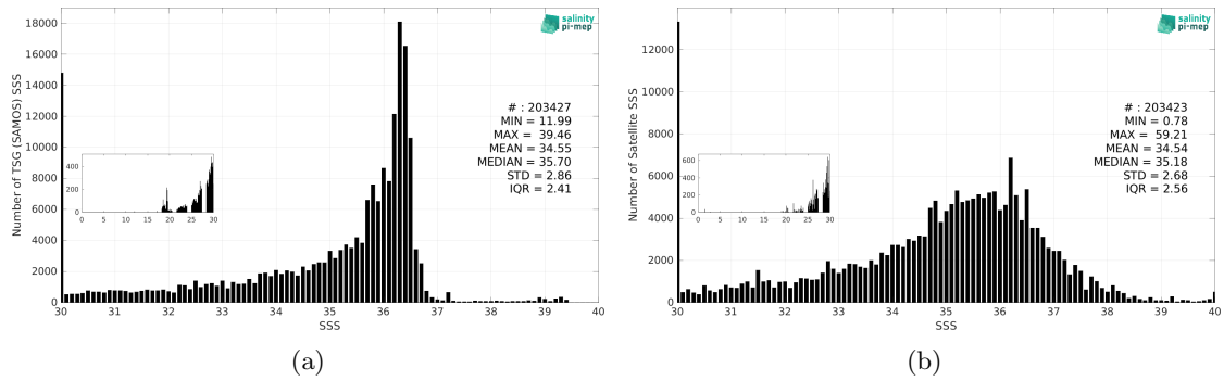
Figure 3: Histograms of SSS from TSG (SAMOS) (a) and SMOS SSS L2Q v331 - No FLAG (CMEMS-CATDS-CPDC) (b) considering all match-up pairs per bins of 0.1 over the Gulf of Mexico Pi-MEP region and for the full satellite product period.
