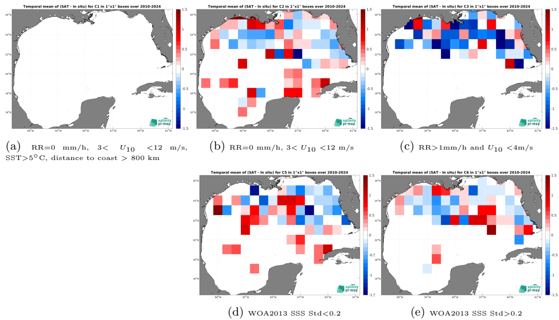
Figure 14: Temporal mean gridded over spatial boxes of size 1^\circ \times 1^\circ of \Delta SSS (SMOS SSS L2Q v331 - No FLAG (CMEMS-CATDS-CPDC) - TSG (SAMOS)) for 5 different subdatasets corresponding to:RR=0 mm/h, 3 < U_{10} < 12 m/s, SST >5^\circ\text{C} , distance to coast > 800 km (a), RR=0 mm/h, 3 < U_{10} < 12 m/s (b), RR >1 mm/h and U_{10} < 4 m/s (c), WOA2013 SSS Std <0.2 (d), WOA2013 SSS Std >0.2 (e).
