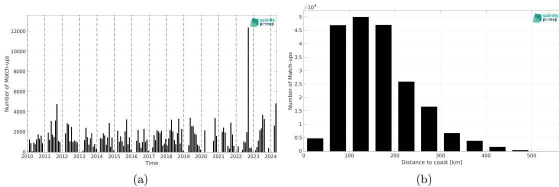
Figure 2: Number of match-ups between TSG (SAMOS) and SMOS SSS L2Q v331 - No FLAG (CMEMS-CATDS-CPDC) SSS as a function of time (a) and as function of the distance to coast (b) over the Gulf of Mexico Pi-MEP region and for the full satellite product period.
