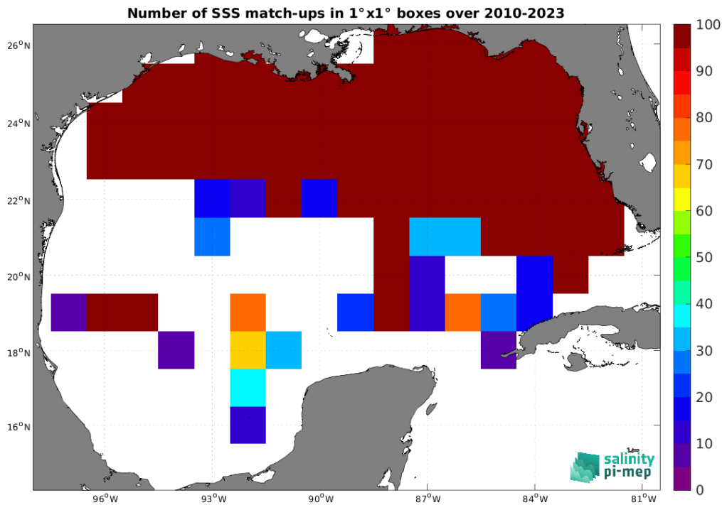
Figure 4: Number of SSS match-ups between TSG (SAMOS) SSS and the SMOS SSS L2Q v331 - No FLAG (CMEMS-CATDS-CPDC) SSS product for the Gulf of Mexico Pi-MEP region over 1°×1° boxes and for the full satellite product period.
