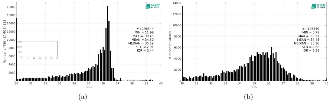
Figure 2: Histograms of SSS from TSG (SAMOS) (a) and SMOS SSS L2Q v331 - No FLAG (CMEMS-CATDS-CPDC) (b) considering all match-up pairs per bins of 0.1 over the Gulf of Mexico Pi-MEP region and for the full satellite product period.
