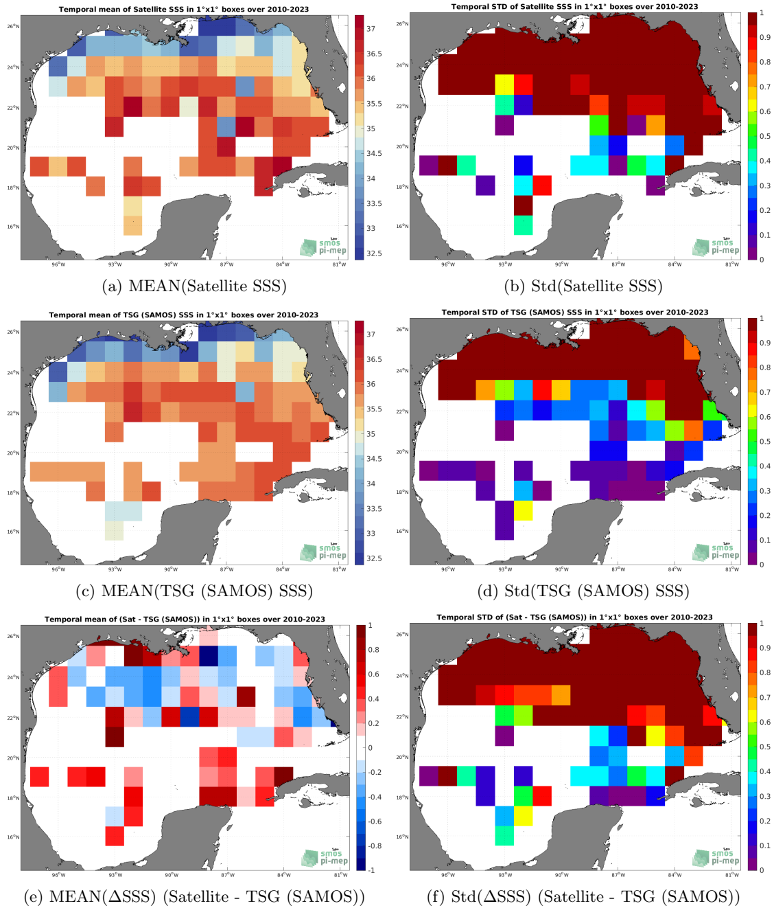
Figure 6: Temporal mean (left) and Std (right) of SSS from SMOS SSS L2Q v331 - No FLAG (CMEMS-CATDS-CPDC) (top), TSG (SAMOS) (middle), and of \Delta SSS (Satellite - TSG (SAMOS)). Only match-up pairs are used to generate these maps.
