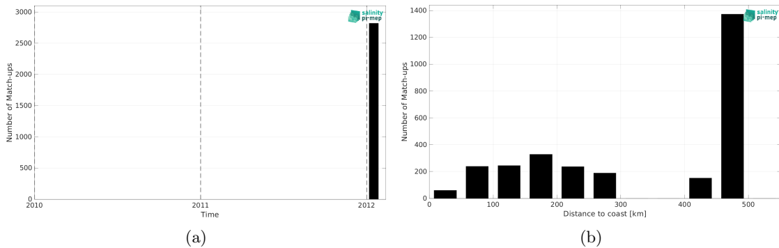
Figure 2: Number of match-ups between TSG (GOSUD-Sailing-ship) and SMOS SSS L2Q v331 - No FLAG (CMEMS-CATDS-CPDC) SSS as a function of time (a) and as function of the distance to coast (b) over the Gulf of Mexico Pi-MEP region and for the full satellite product period.
