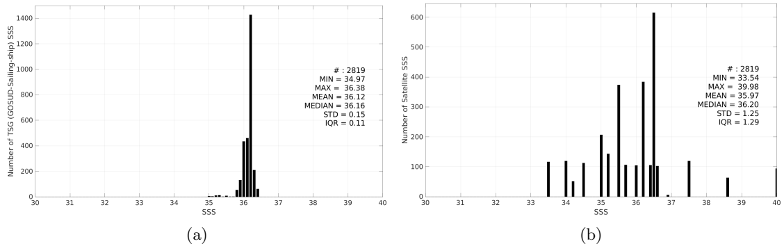
Figure 3: Histograms of SSS from TSG (GOSUD-Sailing-ship) (a) and SMOS SSS L2Q v331 - No FLAG (CMEMS-CATDS-CPDC) (b) considering all match-up pairs per bins of 0.1 over the Gulf of Mexico Pi-MEP region and for the full satellite product period.
