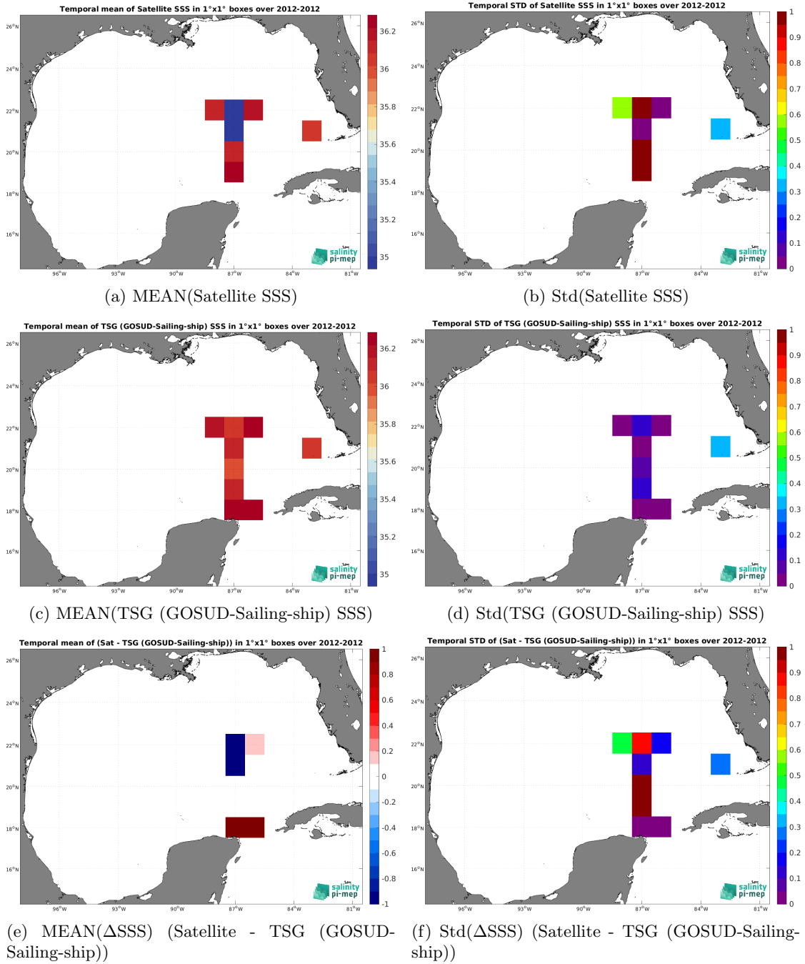
Figure 7: Temporal mean (left) and Std (right) of SSS from SMOS SSS L2Q v331 - No FLAG (CMEMS-CATDS-CPDC) (top), TSG (GOSUD-Sailing-ship) (middle), and of \Delta SSS (Satellite - TSG (GOSUD-Sailing-ship)). Only match-up pairs are used to generate these maps.
