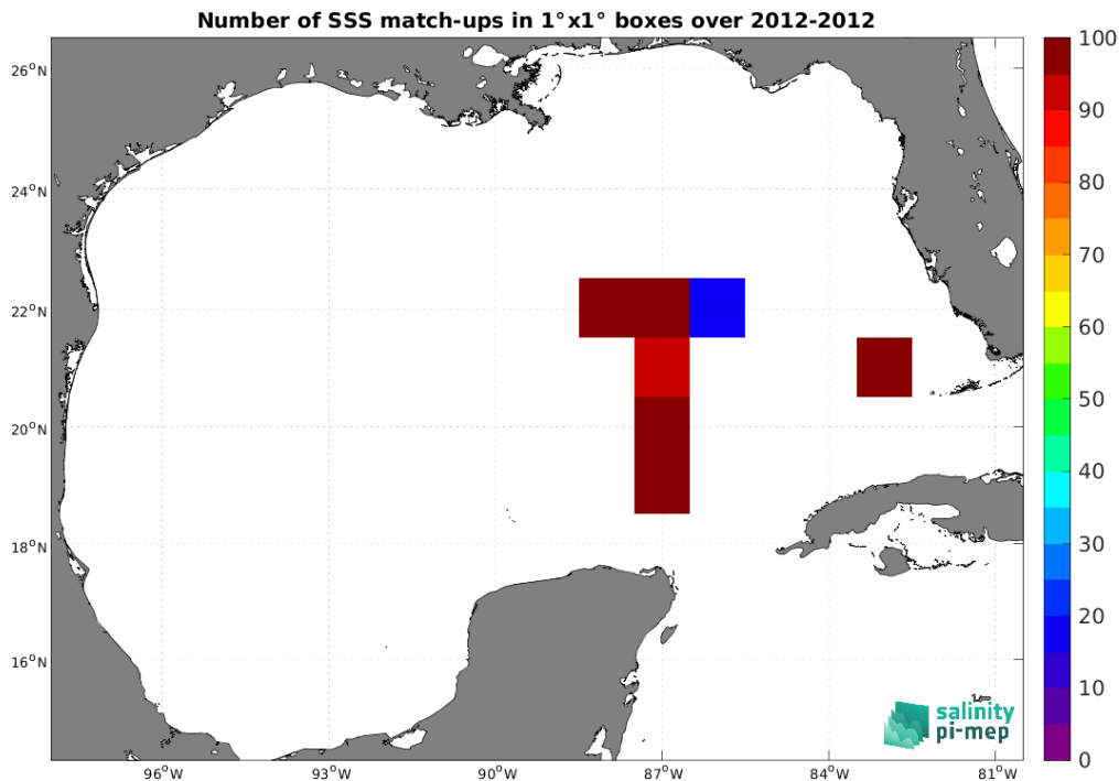
Figure 4: Number of SSS match-ups between TSG (GOSUD-Sailing-ship) SSS and the SMOS SSS L2Q v331 - No FLAG (CMEMS-CATDS-CPDC) SSS product for the Gulf of Mexico Pi-MEP region over 1^\circ \times 1^\circ boxes and for the full satellite product period.
