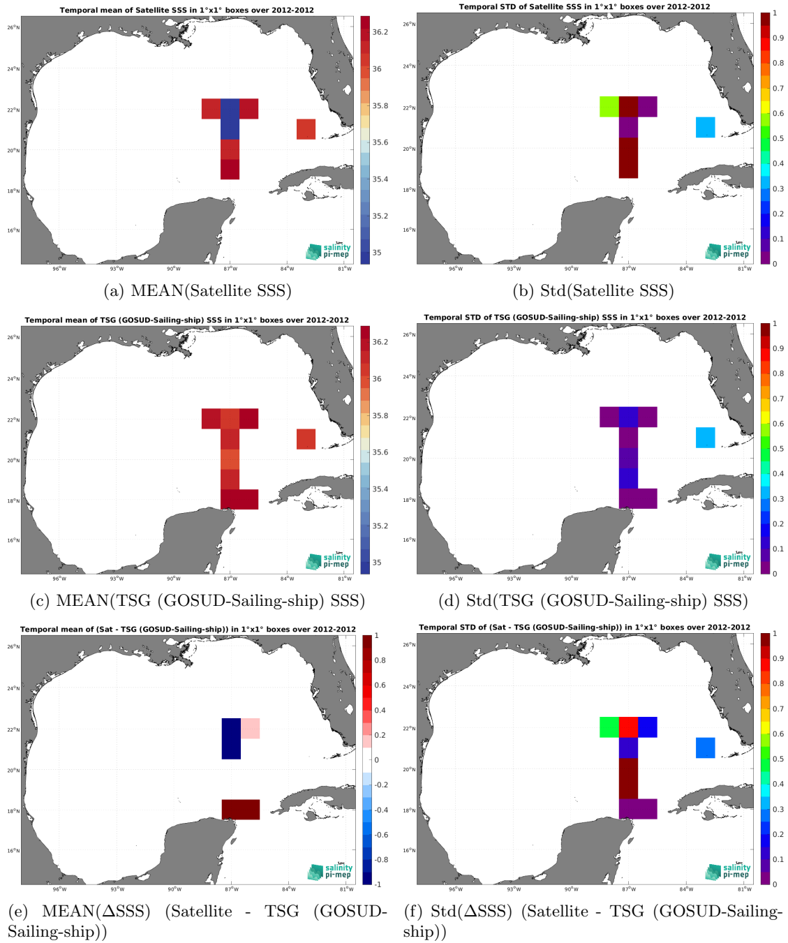
Figure 6: Temporal mean (left) and Std (right) of SSS from SMOS SSS L2Q v331 - No FLAG (CMEMS-CATDS-CPDC) (top), TSG (GOSUD-Sailing-ship) (middle), and of \Delta SSS (Satellite - TSG (GOSUD-Sailing-ship)). Only match-up pairs are used to generate these maps.
