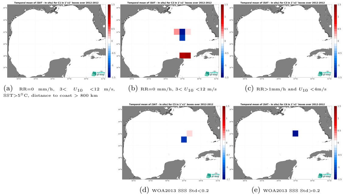
Figure 12: Temporal mean gridded over spatial boxes of size 1^{\circ}\times 1^{\circ} of \Delta SSS (SMOS SSS L2Q v331 - No FLAG (CMEMS-CATDS-CPDC) - TSG (GOSUD-Sailing-ship)) for 5 different sub-datasets corresponding to:RR=0 mm/h, 3 < U_{10} < 12 m/s, SST >5^{\circ}\text{C} , distance to coast > 800 km (a), RR=0 mm/h, 3 < U_{10} < 12 m/s (b), RR >1 mm/h and U_{10} < 4 m/s (c), WOA2013 SSS Std <0.2 (d), WOA2013 SSS Std >0.2 (e).
