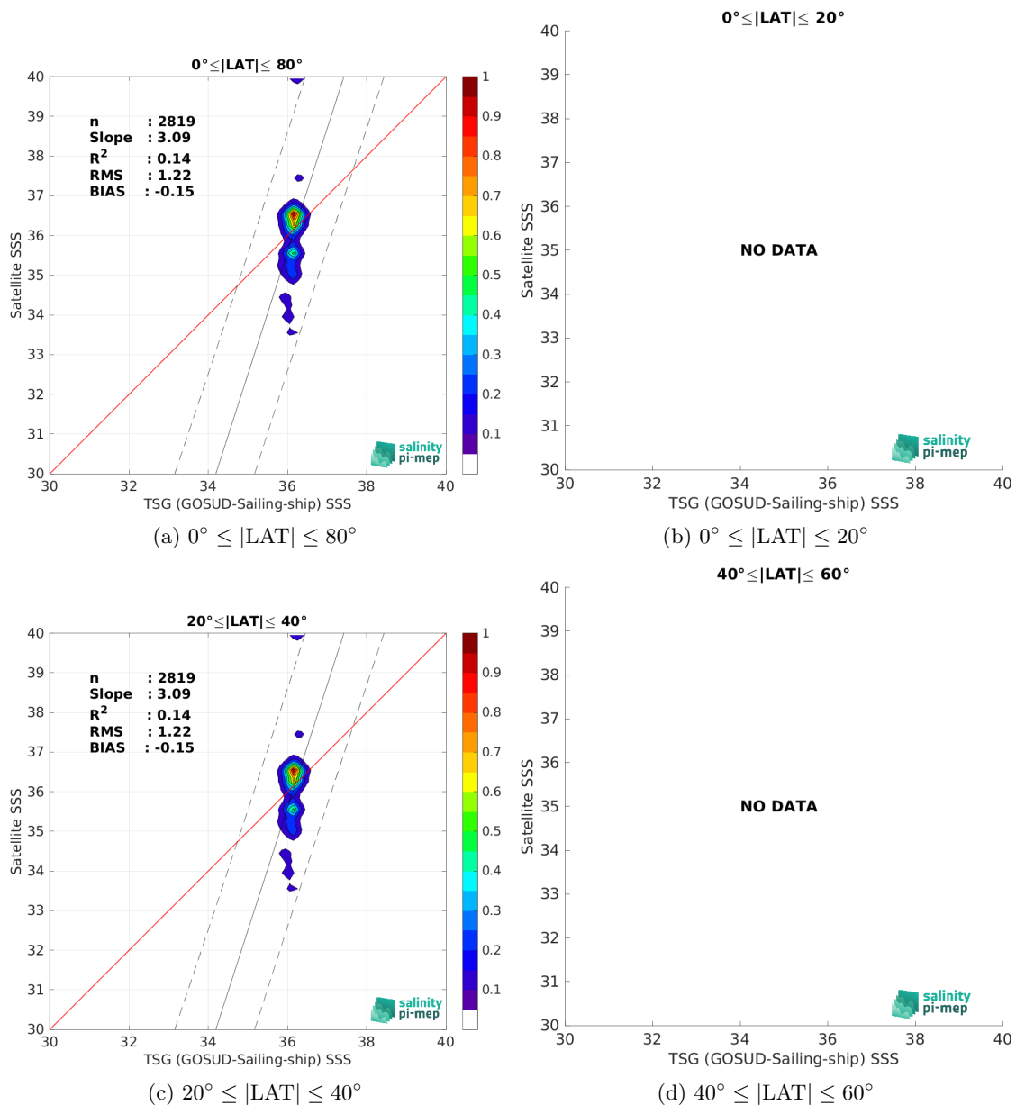
Figure 9: Contour maps of the concentration of SMOS SSS L2Q v331 - No FLAG (CMEMS-CATDS-CPDC) SSS (y-axis) versus TSG (GOSUD-Sailing-ship) SSS (x-axis) at match-up pairs for different latitude bands. For each plot, the red line shows x=y . The black thin and dashed lines indicate a linear fit through the data cloud and the \pm 95\% confidence levels, respectively. The number match-up pairs n , the slope and R^2 coefficient of the linear fit, the root mean square (RMS) and the mean bias between satellite and in situ data are indicated for each latitude band in each plots.
