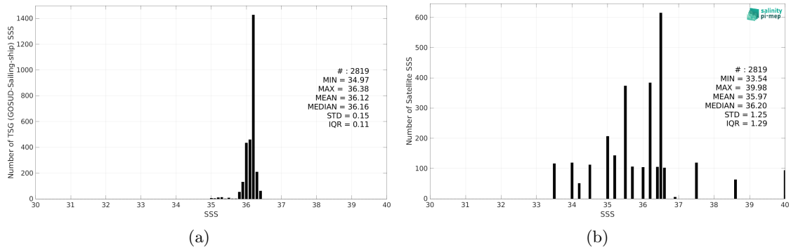
Figure 2: Histograms of SSS from TSG (GOSUD-Sailing-ship) (a) and SMOS SSS L2Q v331 - No FLAG (CMEMS-CATDS-CPDC) (b) considering all match-up pairs per bins of 0.1 over the Gulf of Mexico Pi-MEP region and for the full satellite product period.
