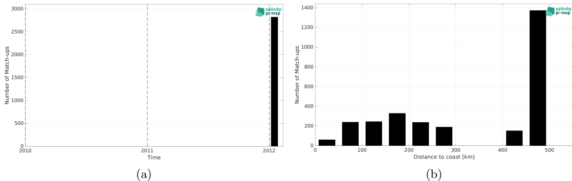
Figure 1: Number of match-ups between TSG (GOSUD-Sailing-ship) and SMOS SSS L2Q v331 - No FLAG (CMEMS-CATDS-CPDC) SSS as a function of time (a) and as function of the distance to coast (b) over the Gulf of Mexico Pi-MEP region and for the full satellite product period.
