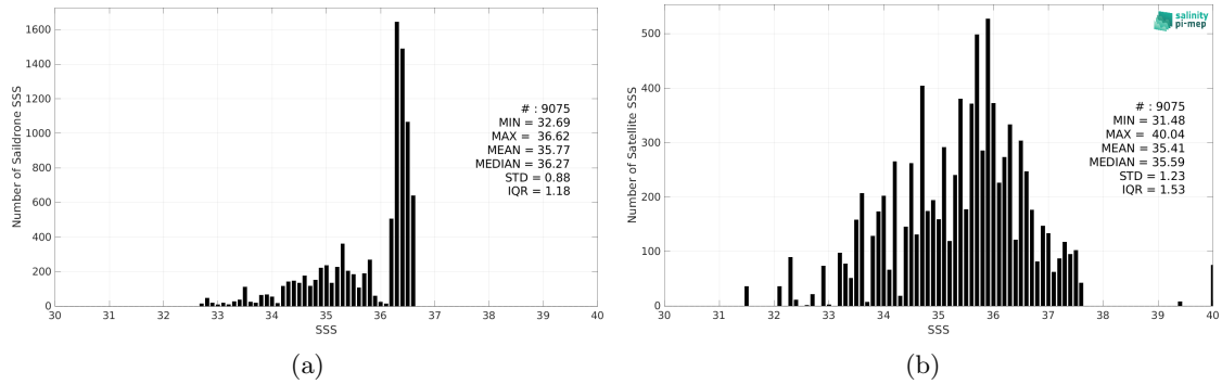
Figure 2: Histograms of SSS from Saifdrone (a) and SMOS SSS L2Q v331 - No FLAG (CMEMS-CATDS-CPDC) (b) considering all match-up pairs per bins of 0.1 over the Gulf of Mexico Pi-MEP region and for the full satellite product period.
