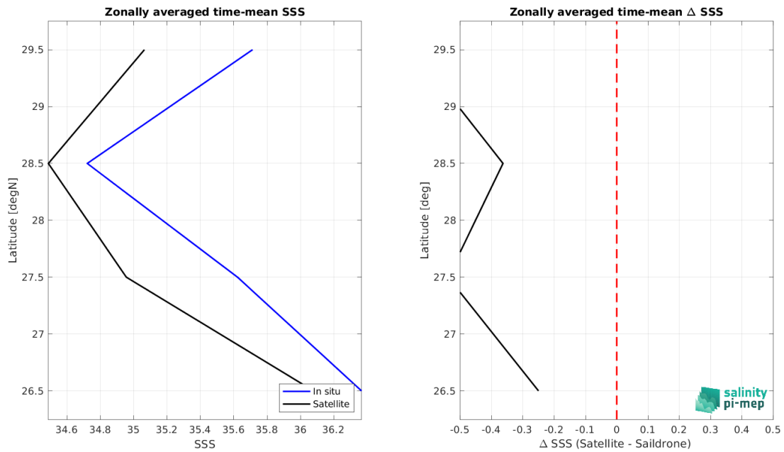
Figure 8: Left panel: Zonal mean SSS from SMOS SSS L2Q v331 - No FLAG (CMEMS-CATDS-CPDC) satellite product (black) and from Sairdrone (blue). Right panel: Zonal mean of \Delta SSS (Satellite - Sairdrone) for all the collected Pi-MEP match-up pairs estimated over the full satellite product period.
