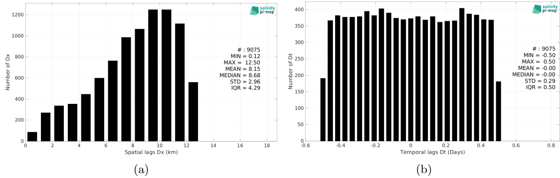
Figure 5: Histograms of the spatial (a) and temporal (b) lags between the location/time of the Saildrone measurement and the date of the corresponding SMOS SSS L2Q v331 - No FLAG (CMEMS-CATDS-CPDC) SSS pixel.
