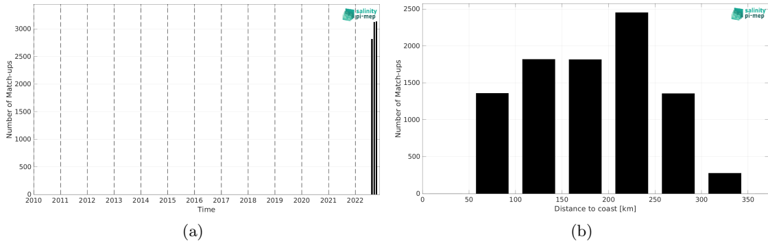
Figure 1: Number of match-ups between Saildrone and SMOS SSS L2Q v331 - No FLAG (CMEMS-CATDS-CPDC) SSS as a function of time (a) and as function of the distance to coast (b) over the Gulf of Mexico Pi-MEP region and for the full satellite product period.
