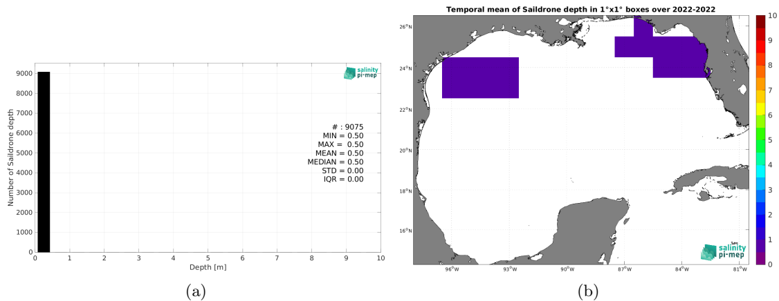
Figure 3: Histograms of the depth of the upper level SSS measurements from Saifdrone in the Match-up DataBase for the Gulf of Mexico Pi-MEP region (a) and temporal mean spatial distribution of pressure of the in situ SSS data over 1^\circ \times 1^\circ boxes and for the full satellite product period (b).
