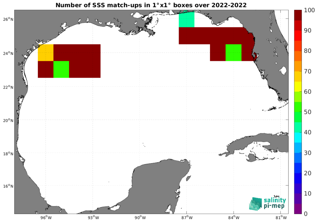
Figure 4: Number of SSS match-ups between Saildrone SSS and the SMOS SSS L2Q v331 - No FLAG (CMEMS-CATDS-CPDC) SSS product for the Gulf of Mexico Pi-MEP region over 1^\circ \times 1^\circ boxes and for the full satellite product period.
