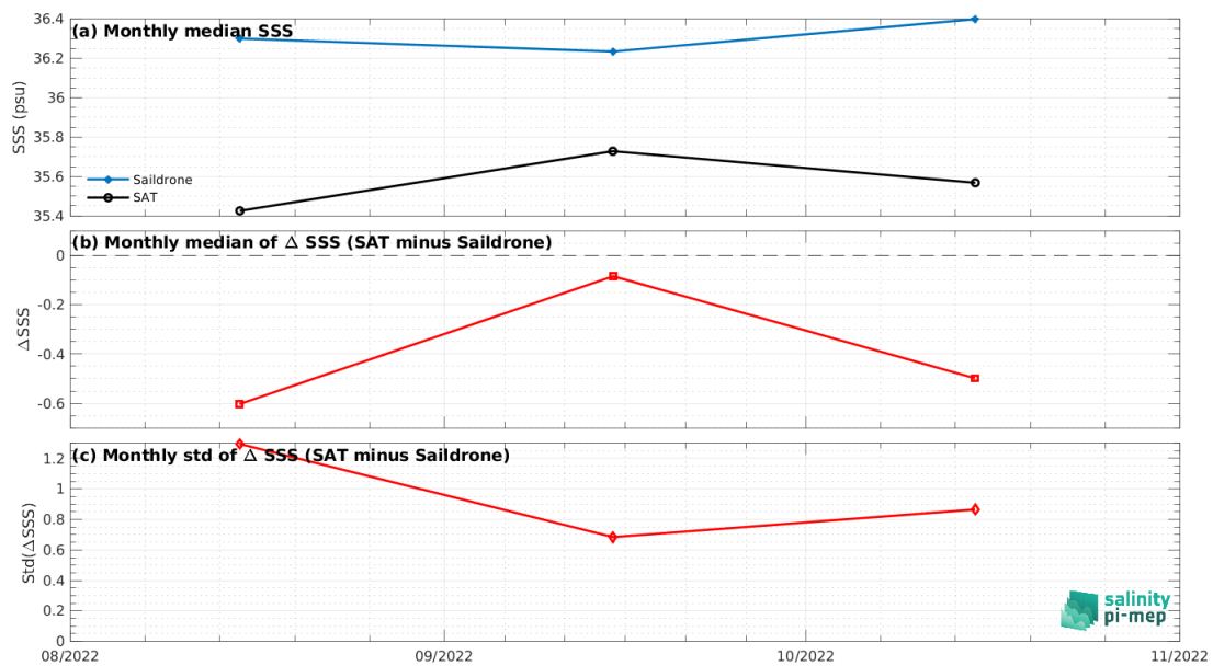
Figure 7: Time series of the monthly median SSS (top), median of \Delta SSS (Satellite - Saildrone) and Std of \Delta SSS (Satellite - Saildrone) over the Gulf of Mexico Pi-MEP region considering all match-ups collected by the Pi-MEP.
