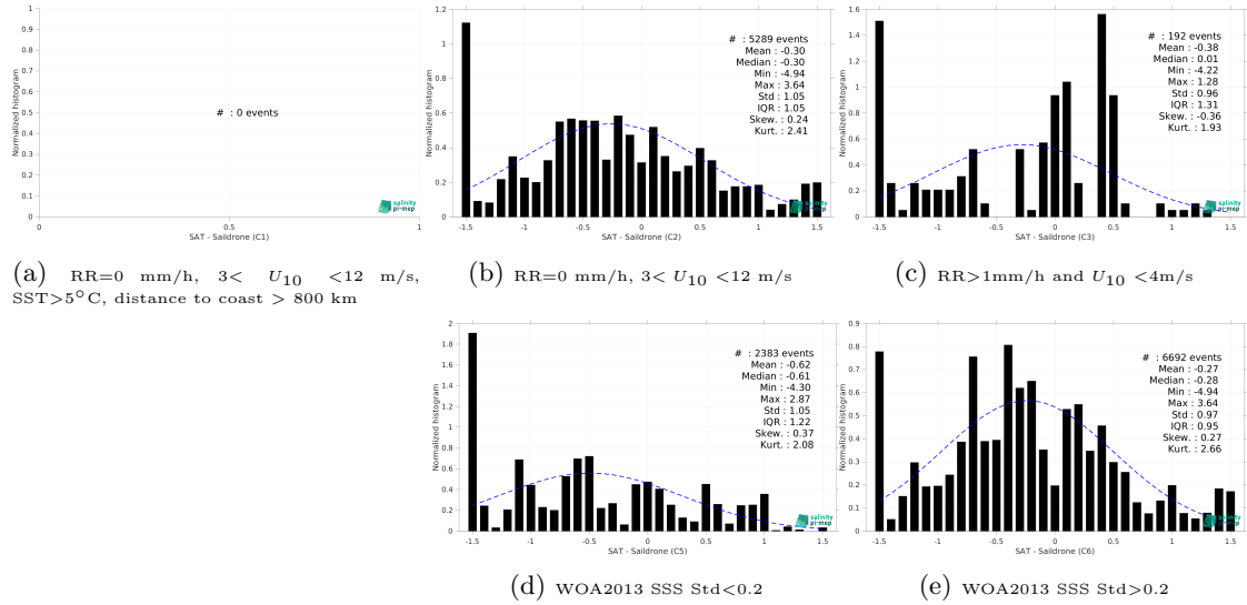
Figure 13: Normalized histogram of \Delta SSS (SMOS SSS L2Q v331 - No FLAG (CMEMS-CATDS-CPDC) - Saildrone) for 5 different subdatasets corresponding to: RR=0 mm/h, 3 < U_{10} < 12 m/s, SST > 5°C, distance to coast > 800 km (a), RR=0 mm/h, 3 < U_{10} < 12 m/s (b), RR > 1mm/h and U_{10} < 4 m/s (c), WOA2013 SSS Std < 0.2 (d), WOA2013 SSS Std > 0.2 (e).
