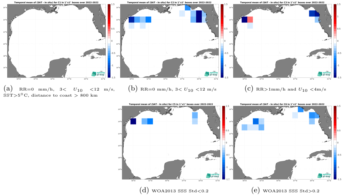
Figure 12: Temporal mean gridded over spatial boxes of size 1^{\circ}\times 1^{\circ} of \Delta\text{SSS} (SMOS SSS L2Q v331 - No FLAG (CMEMS-CATDS-CPDC) - Saildrone) for 5 different subdatasets corresponding to:RR=0 mm/h, 3 < U_{10} < 12 m/s, SST >5^{\circ}\text{C} , distance to coast > 800 km (a), RR=0 mm/h, 3 < U_{10} < 12 m/s (b), RR >1 mm/h and U_{10} < 4 m/s (c), WOA2013 SSS Std <0.2 (d), WOA2013 SSS Std >0.2 (e).
