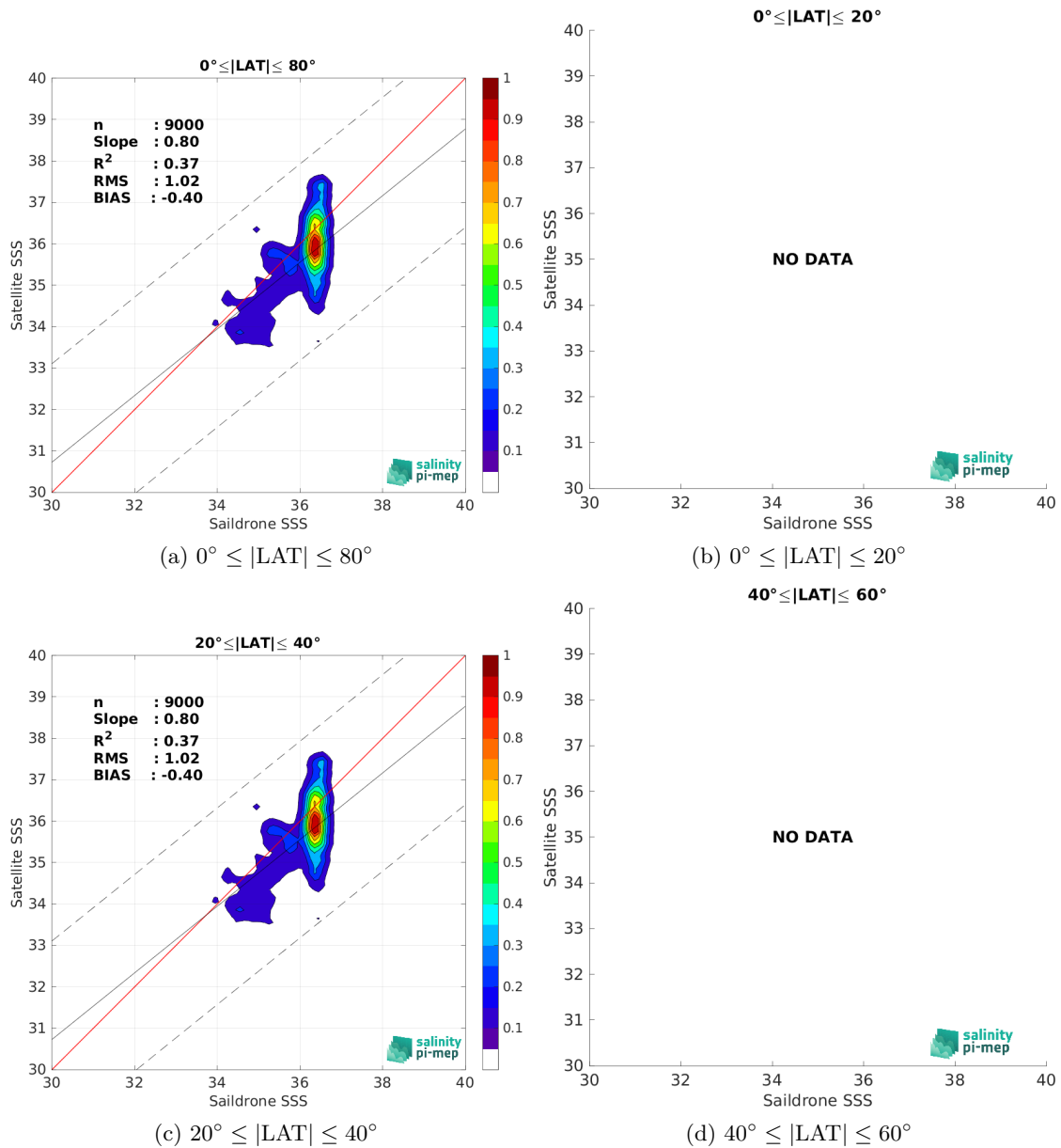
Figure 9: Contour maps of the concentration of SMOS SSS L2Q v331 - No FLAG (CMEMS-CATDS-CPDC) SSS (y-axis) versus Saildrone SSS (x-axis) at match-up pairs for different latitude bands. For each plot, the red line shows x=y . The black thin and dashed lines indicate a linear fit through the data cloud and the \pm 95\% confidence levels, respectively. The number match-up pairs n , the slope and R^2 coefficient of the linear fit, the root mean square (RMS) and the mean bias between satellite and in situ data are indicated for each latitude band in each plots.
