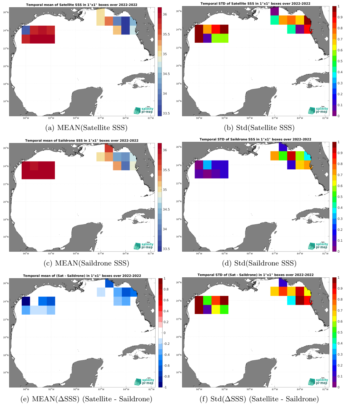
Figure 6: Temporal mean (left) and Std (right) of SSS from SMOS SSS L2Q v331 - No FLAG (CMEMS-CATDS-CPDC) (top), Saildrone (middle), and of \Delta SSS (Satellite - Saildrone). Only match-up pairs are used to generate these maps.
