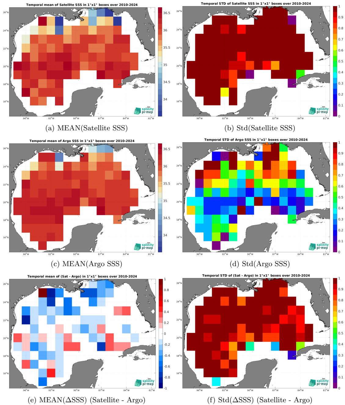
Figure 7: Temporal mean (left) and Std (right) of SSS from SMOS SSS L2Q v331 - No FLAG (CMEMS-CATDS-CPDC) (top), Argo (middle), and of \Delta SSS (Satellite - Argo). Only match-up pairs are used to generate these maps.
