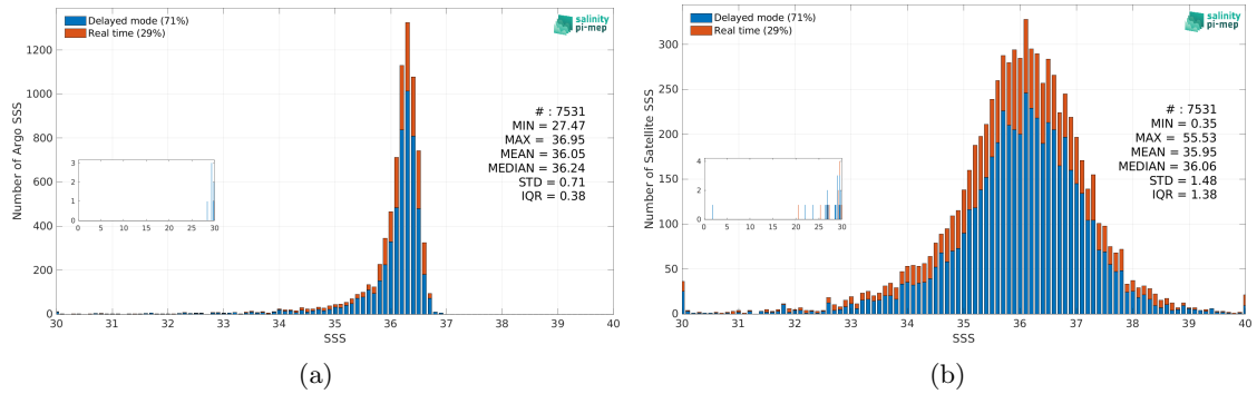
Figure 3: Histograms of SSS from Argo (a) and SMOS SSS L2Q v331 - No FLAG (CMEMS-CATDS-CPDC) (b) considering all match-up pairs per bins of 0.1 over the Gulf of Mexico Pi-MEP region and for the full satellite product period.
