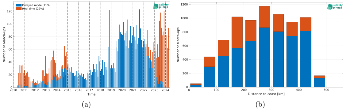
Figure 2: Number of match-ups between Argo and SMOS SSS L2Q v331 - No FLAG (CMEMS-CATDS-CPDC) SSS as a function of time (a) and as function of the distance to coast (b) over the Gulf of Mexico Pi-MEP region and for the full satellite product period.
