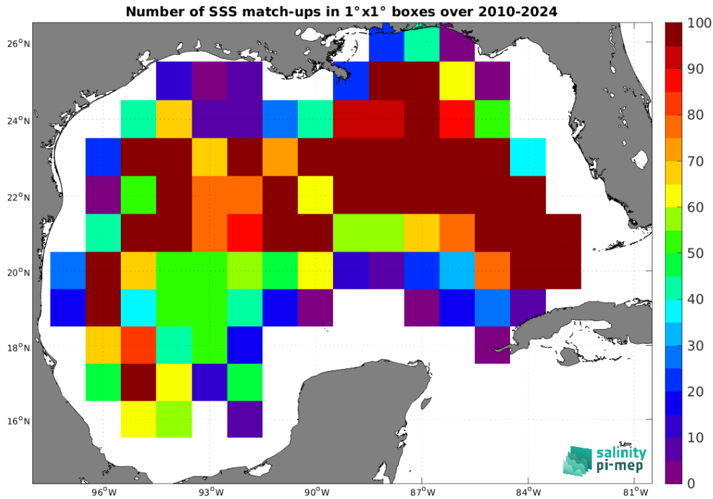
Figure 5: Number of SSS match-ups between Argo SSS and the SMOS SSS L2Q v331 - No FLAG (CMEMS-CATDS-CPDC) SSS product for the Gulf of Mexico Pi-MEP region over 1^\circ \times 1^\circ boxes and for the full satellite product period.
